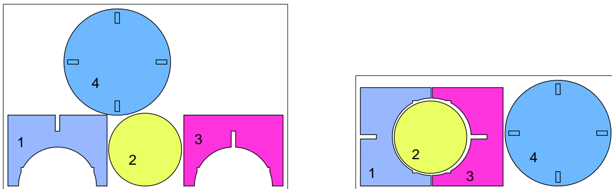
FIGURE 3.20 – Two layouts obtained with the same docking order. Left : Without taking enclosed area into account the first part is placed with the concavity against the bottom packing border. This prevents the second part to nest within and cascades into a series of poor placements. Right : Taking into account enclosed areas results in a placement of the first part that allows nesting of the second part and produces a layout with lower wastage.
