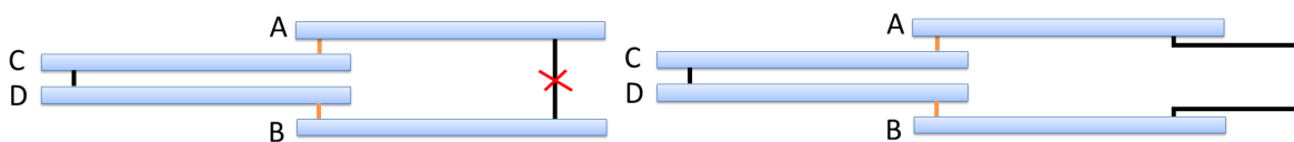
FIGURE 3.6 – Left : Four bars seen from the top. Black segments indicate a fixed joint, while orange indicates a hinge joint. C,D can rotate around A,B but will cut the fixed axle between A,B. This system cannot be resolved by assigning different layers to A,B,C,D. Right : The only solution is to change the shape of the axle, making room for C,D.
