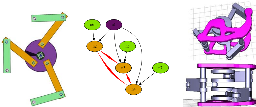
FIGURE 3.3 – Left : Input 2D mechanism. Middle : Graph used to construct the layout. Edge orientation indicates which part includes which other, while the red edges show which parts have to be layered. Right : Two views of the generated mechanism. The synthesized chassis appears in pink. The crankshaft configuration automatically results from the inclusion and layering constraints.
