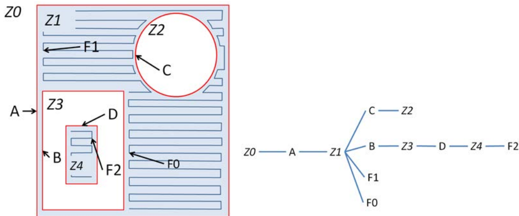
FIGURE 1.10 – Left : a slice with perimeters (in red) and infill paths (in blue). The perimeters are cyclic and delimit zone. Right : the tree structure shows the topology of the different paths.
