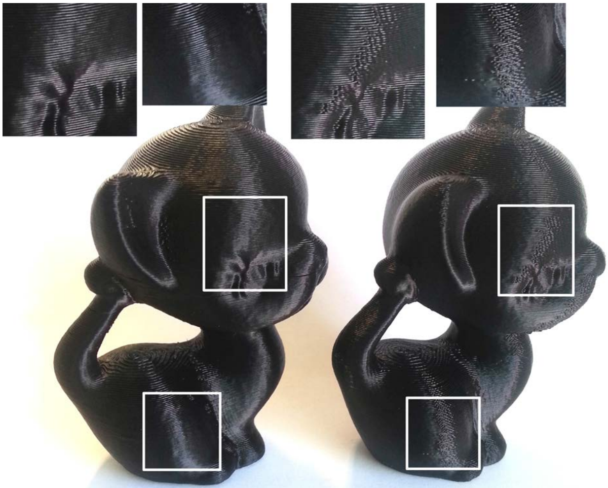
FIGURE 2.20 – Left : Our result, zippers are hidden in low visibility regions. Right : Skeinforge with jitter plugin.
