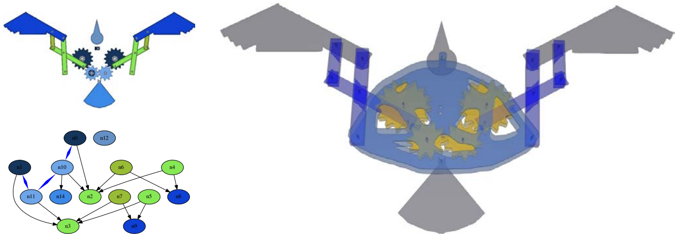
FIGURE 3.11 – Eagle model. The mechanism shown in transparency (right) is generated from the design (top left). The mechanism graph (bottom left) shows inclusions and contact edges (bold blue). No contradictions were encountered : there is no layering. Note the double gears including the bars, as well as the space carved for the inner bars in the bars actioning the wings.
