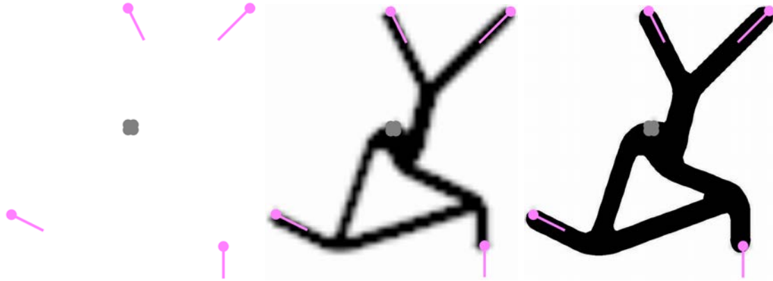
FIGURE 3.8 – Chassis synthesis by topology optimization. Left : four forces resulting from hinges at a given time frame (pink) and attachment point (gray). Middle : Optimized densities for these forces. Right : Final shape after smoothing and contour extraction.
