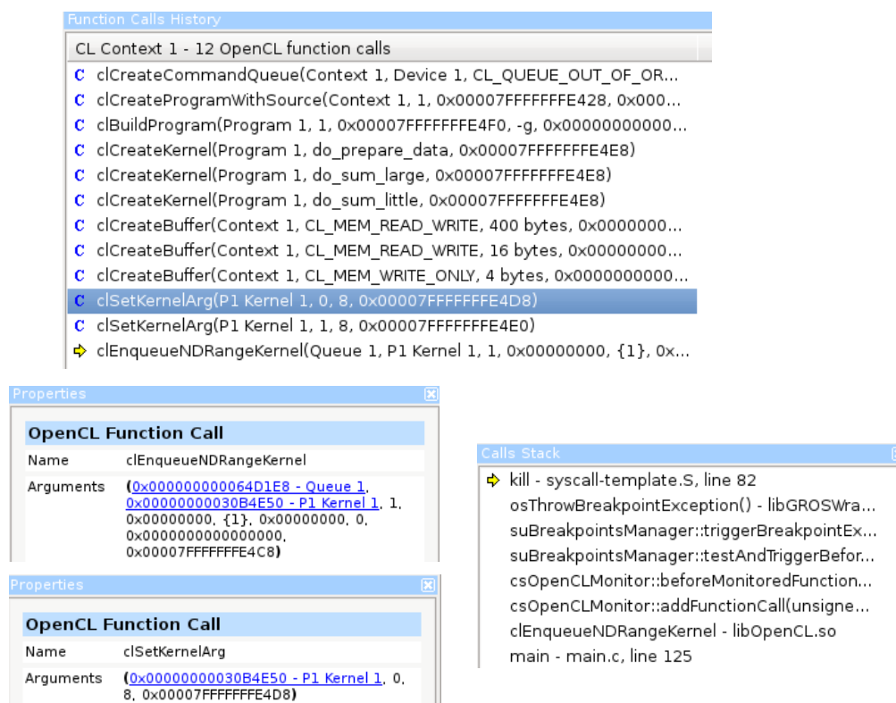
Figure 7.2: GDB interface of OpenCL debugging.
