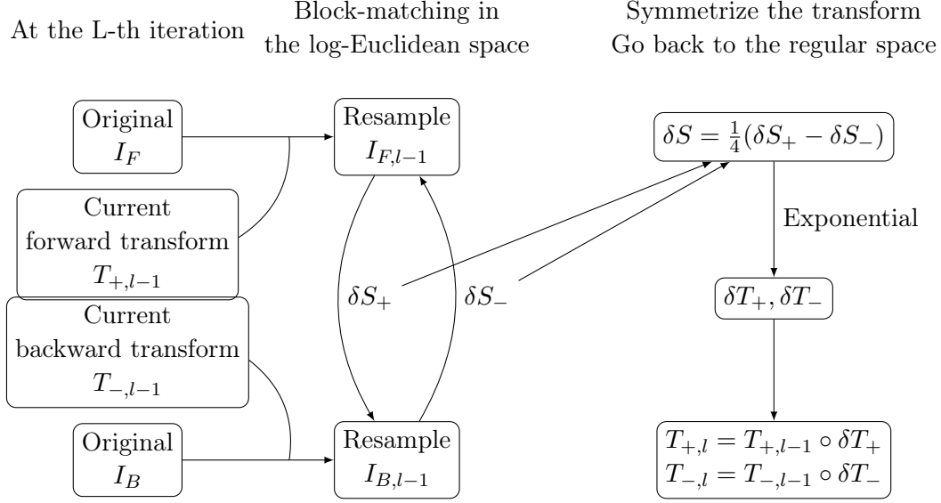
Figure 4.1: Graphical illustration of one iteration of the block-matching algorithm.
