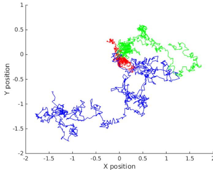
Figure 3.4: Illustration of Brownian motion of three particles with different diffusion coefficients, red: D = 1.10^{-3} \text{ mm}^2.\text{s}^{-1} , green: D = 2.10^{-3} \text{ mm}^2.\text{s}^{-1} , blue: D = 4.10^{-3} \text{ mm}^2.\text{s}^{-1} for 1000 steps and a time between step \Delta = 0.1\text{s}
