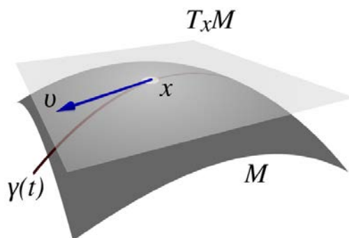
Figure 3.10: Illustration of a curved Riemannian space with a tangent space T_x M defined for a point x ( common license https://en.wikipedia.org/wiki/Tangent_space ).
