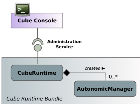
Figure 6.25: Cube Console
