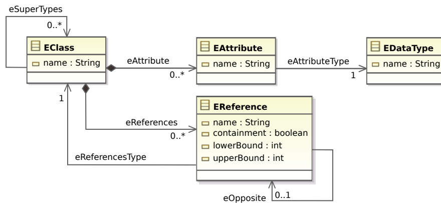
Figure 5.3: ECORE Meta-model
