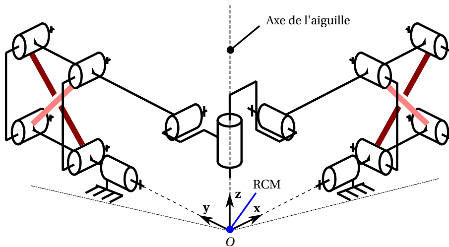
FIGURE 4.3 – Architecture du porte-aiguille.
