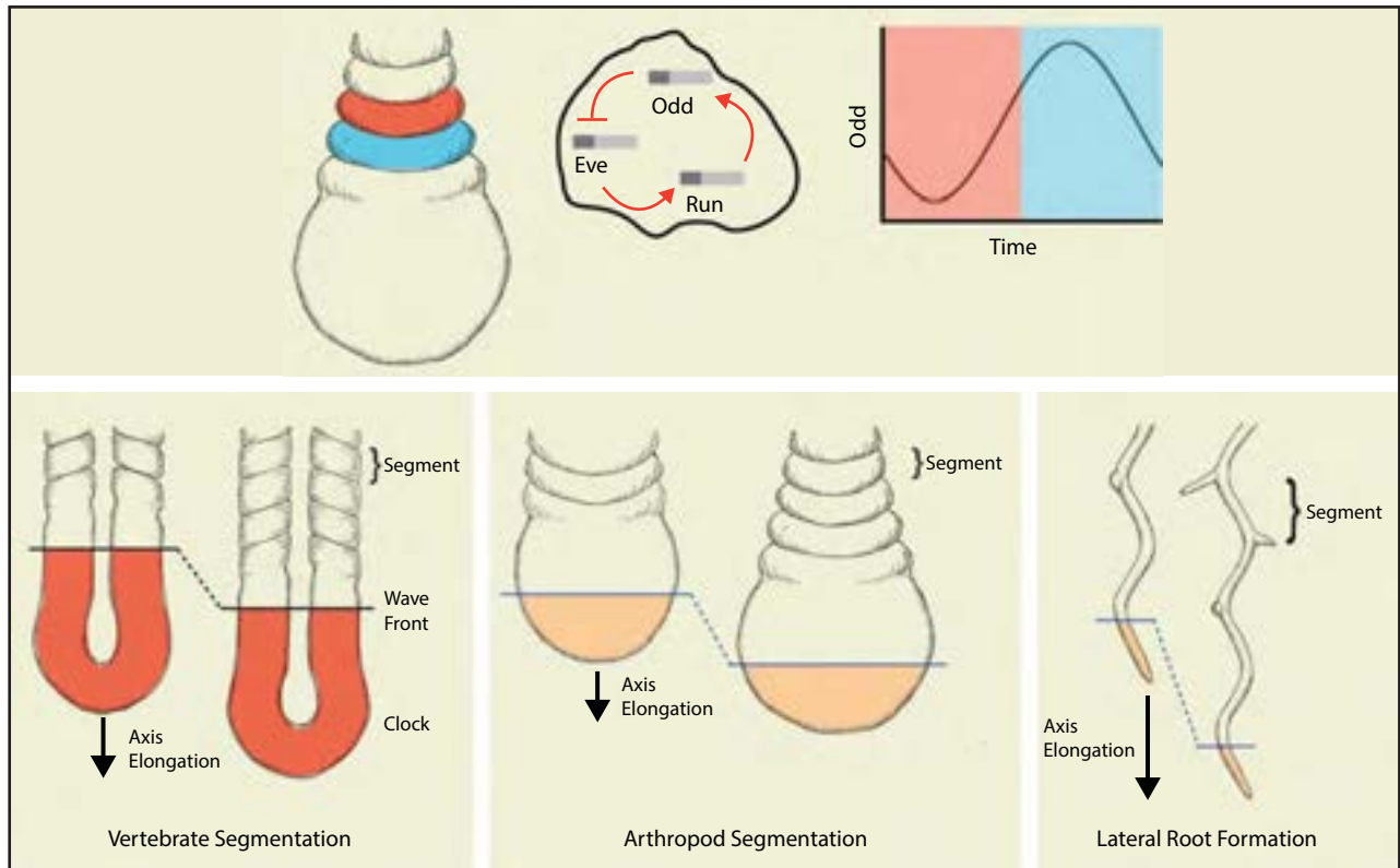
Figure 24 - Clock-mechanisms as developmental rulers
