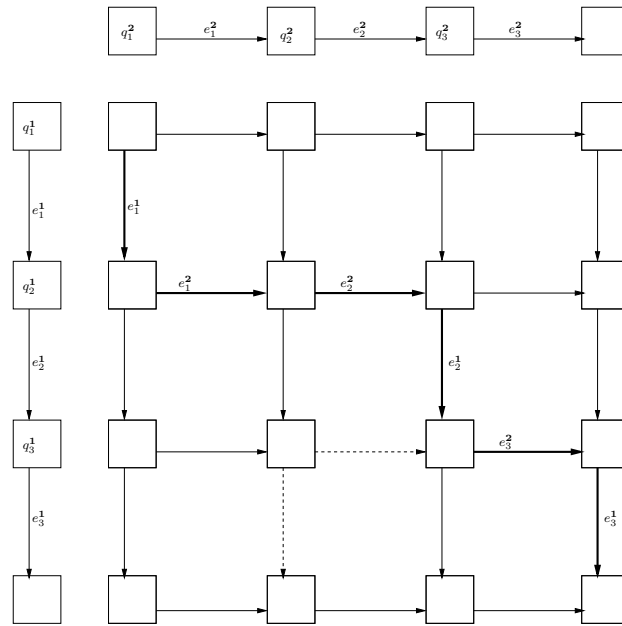
Figure 4.3: The product automaton for a process system with n = 2, k = 3 . The thick arrows indicate the path corresponding to the qualitative behavior w = e_1^1 e_1^2 e_2^2 e_1^3 e_2^3 e_2^1 e_3^1 e_2^3 e_3^3 . The race between e_3^1 and e_2^2 in state (q_3^1, q_2^2) is indicated by the dashed arrows.
