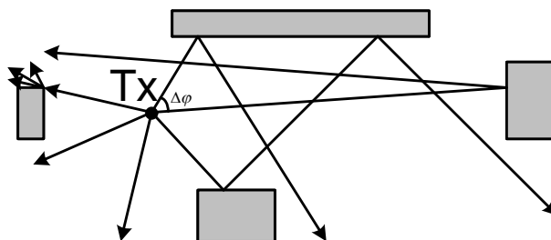
Figure 2.2: Ray launching.
