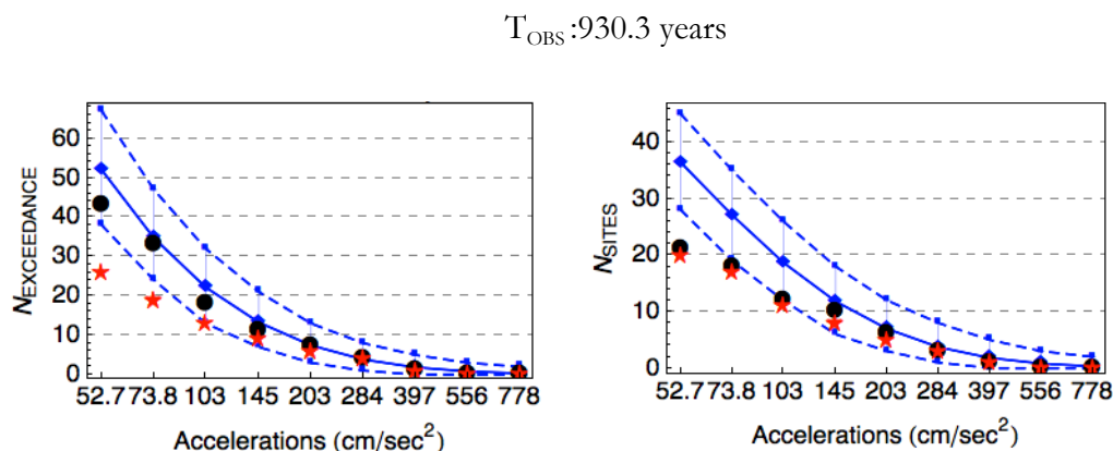
Figure 3.13: Comparison of the observed and predicted number of exceedances at different acceleration levels considering original observation lifetimes at 137 stations with minimum inter-site distance of 10 km. Left: the comparison based on the number of exceedances at sites considered, Right: the comparison based on the number of sites with exceedance. Blue curves: median and percentiles 2.5 and 97.5 of the predicted distributions (see section 2.2 of second chapter), black circles: observed exceedances considering all records (including foreshocks/aftershocks), red stars: observed exceedances considering only records of mainshocks.
