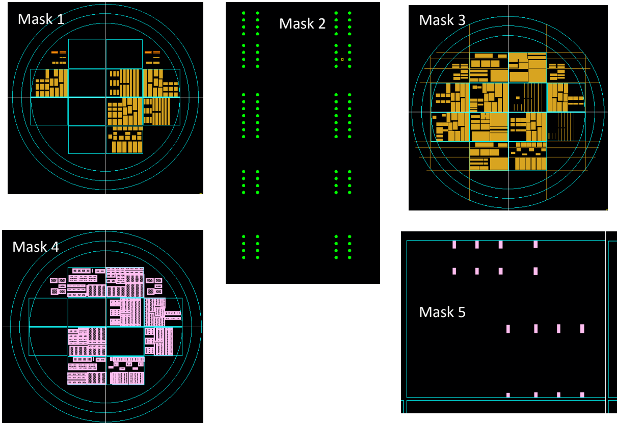
Figure 4-42: The designed five masks to fabricate the whole patterns.
