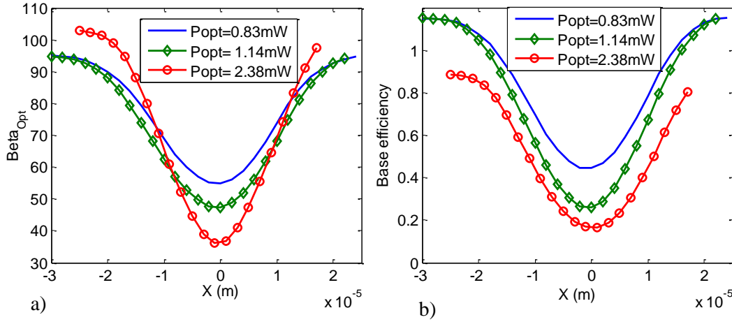
Figure 3-55: a) Photocurrent amplification, \beta_{opt} at different P_{opt} . b) Base efficiency at different P_{opt} .
