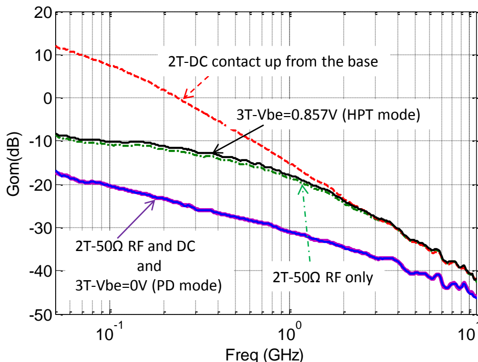
Figure 3-14: Opto-microwave gain versus frequency 10 \times 10 \mu\text{m}^2 SiGe HPT under 2-terminal and 3-terminal configuration.
