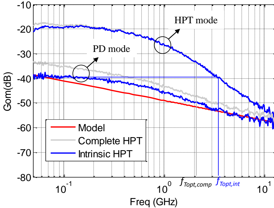
Figure 3-19: The complete and intrinsic G_{om} versus frequency for 10 \times 10 \mu\text{m}^2 HPT in PD and HPT modes at V_{ce}=2\text{V} .
