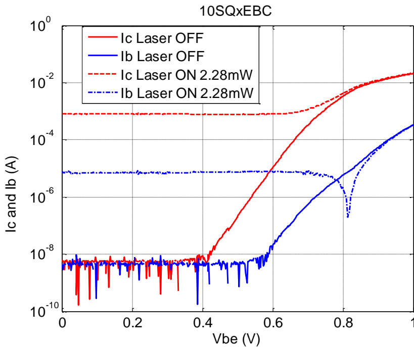
Figure 2-17: Gummel plot of 10 \times 10 \mu\text{m}^2 HPT under 2.28mW illumination and dark condition
