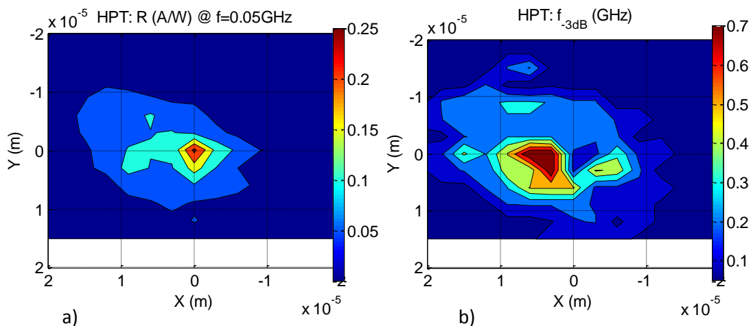
Figure 5-19: OM-SNOM of SiGe HPT with edge illumination at V_{ce}=1.5V and V_{be}=0.85V a) low frequency responsivity and b) cutoff frequency.
