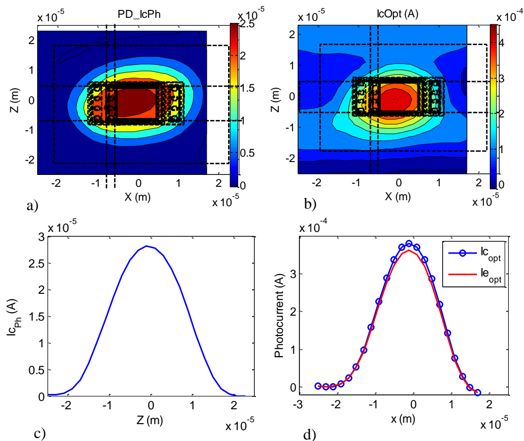
Figure 3-41: Photocurrent measured at the collector of the 10 \times 10 \mu\text{m}^2 HPT in a) PD Mode, b) HPT mode. The slice curves of the collector photocurrent c) PD mode, d) HPT mode.
