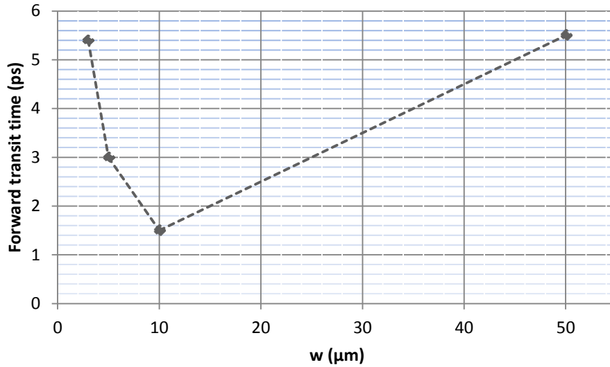
Figure 3-26: Experimentally measured forward transit time versus the optical window size at V_{be}=0.823V and V_{ce}=3.5V
