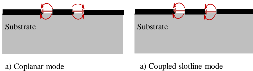
Figure 4-2: coplanar line wave propagation modes.
