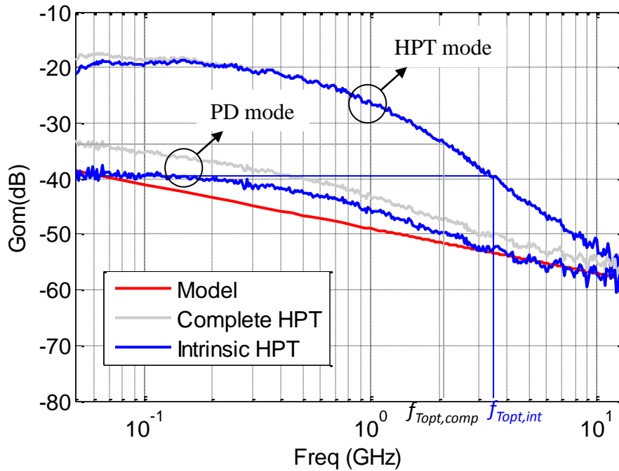
Figure 3-19: The complete and intrinsic G_{om} versus frequency for 10 \times 10 \mu m^2 HPT in PD and HPT modes at V_{ce}=2V .
