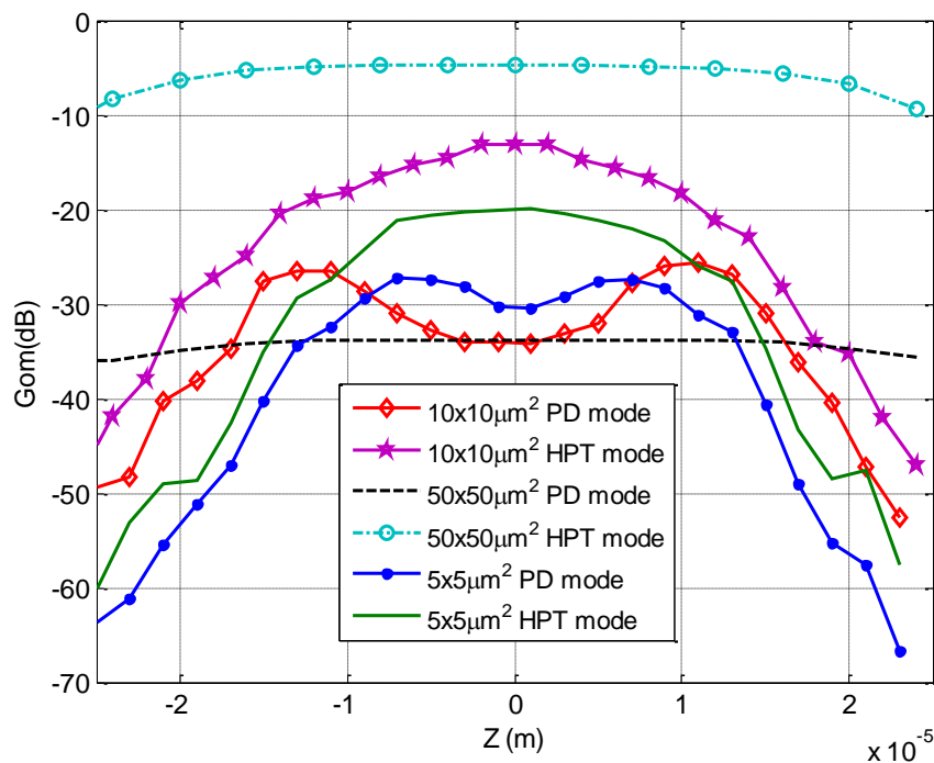
Figure 3-64: The slice curve of the low frequency opto-microwave gain of 50 \times 50 \mu\text{m}^2 , 10 \times 10 \mu\text{m}^2 and 5 \times 5 \mu\text{m}^2 optical window size HPTs at X=0 \text{m} in HPT ( V_{be}=0.857 \text{V} ) and PD ( V_{be}=0 \text{V} ) modes of operation for V_{ce}=3 \text{V} .
