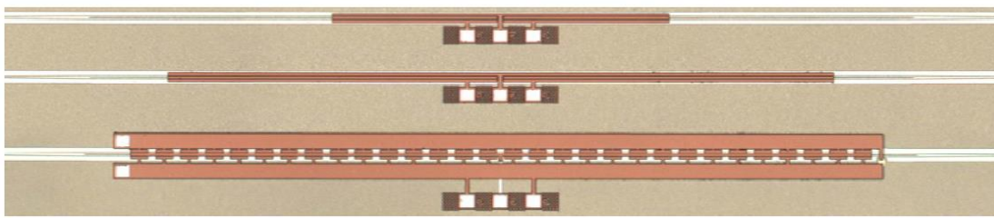
Figure 1-30: The three MZMs under test; from top to bottom the 1000- \mu\text{m} Push-Pull MZM, the 2000- \mu\text{m} Push-Pull MZM, and the 1500- \mu\text{m} segmented TW electrode MZM with a built-in 50 \Omega termination on the TWE. The TW device is self-terminated with an n+ resistor (far right of device)[210].
