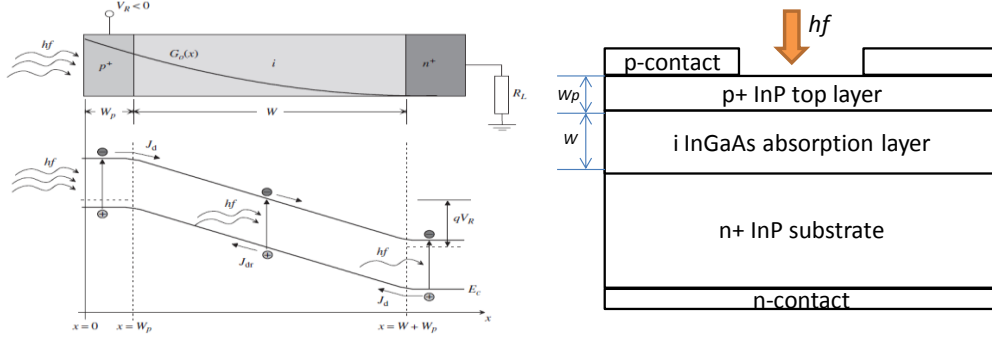
Figure 1-13: Schematic structure (right) and band diagram with structure (left) of a pin photodiode in reverse bias. J_{dr} and J_d are drift and diffusion current densities, respectively
