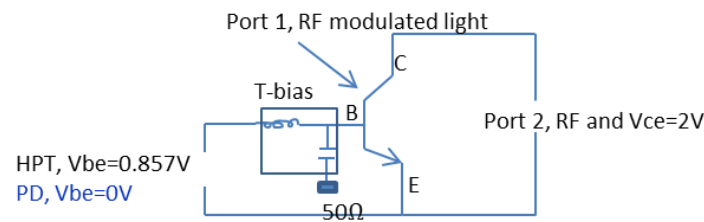
Figure 3-12: 3T configuration
