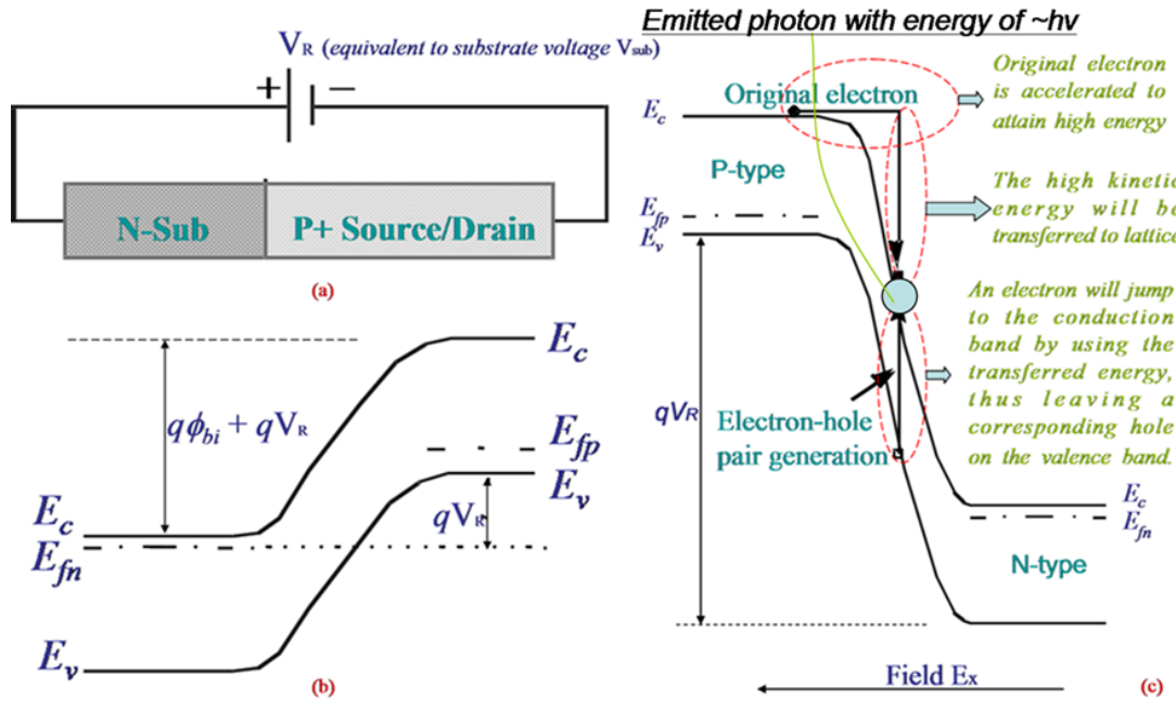
Figure 5-23: Energy band scheme for the impact ionization process for an electron in a reverse biased pn silicon junction [114]
