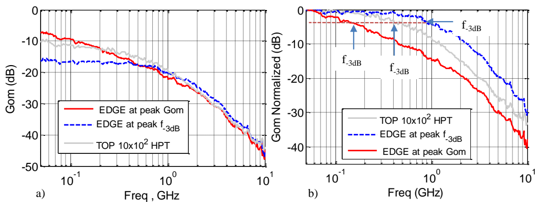
Figure 5-22: The Gom versus frequency of edge and top illuminated HPTs at their peak low frequency gain and cutoff frequency. a) Un-normalized Gom, b) the normalized Gom to indicate the cutoff frequency.
