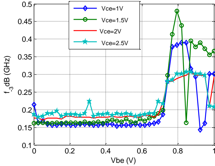
Figure 5-8: Cutoff frequency versus V_{be} at different V_{ce} .
