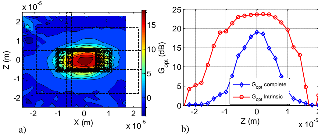
Figure 3-49: Optical gain ( G_{\text{opt}} ) a) The complete HPT topological mapping. b) The complete and intrinsic slice curves at X=0\text{m} of the 10\times 10\mu\text{m}^2 HPT.
