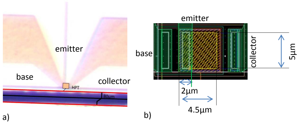
Figure 5-1: a) Microscopic picture of the edge SiGe HPT, b) Layout of structure along with its dimensions.
