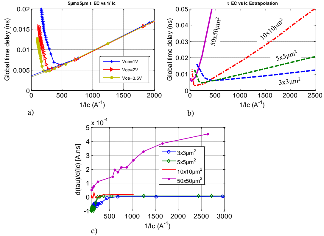
Figure 3-23: Global time delay versus 1/I_c a) 5 \times 5 \mu m^2 HPT at different V_{ce} to show how to extract the junction capacitance and transit time, b) Different size HPTs ( 3 \times 3 \mu m^2 , 5 \times 5 \mu m^2 , 10 \times 10 \mu m^2 and 50 \times 50 \mu m^2 ) at V_{ce} = 3.5V and c) The first derivative of global time delay with respect to 1/I_c .
