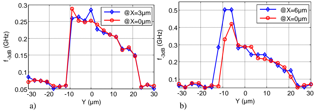
Figure 5-17: The cross section curve of the cutoff frequency along y axis (for top into the substrate) at V_{ce}=1.5V in a) PD mode ( V_{be}=0.8V ), b) HPT mode ( V_{be}=0V ).
