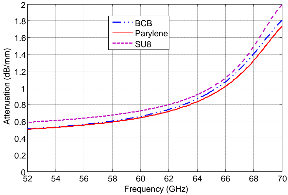
Figure 4-5: The simulated result of the attenuation of coplanar line versus frequency with 16 \mu m polymer layers and line dimensions for 50 \Omega characteristic impedance.
