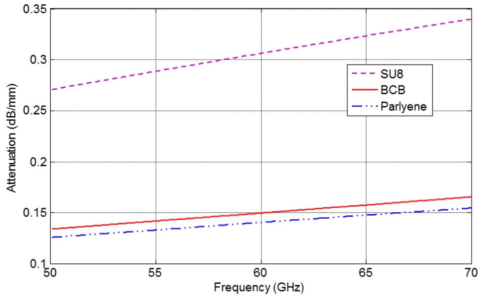
Figure 4-17: The simulated result of the attenuation of grounded coplanar line versus frequency for different dielectric layers. The metal strip width is of 80\mu\text{m} for SU8 and 88\mu\text{m} for BCB or Parylene, whereas the slot width is of 30\mu\text{m} .
