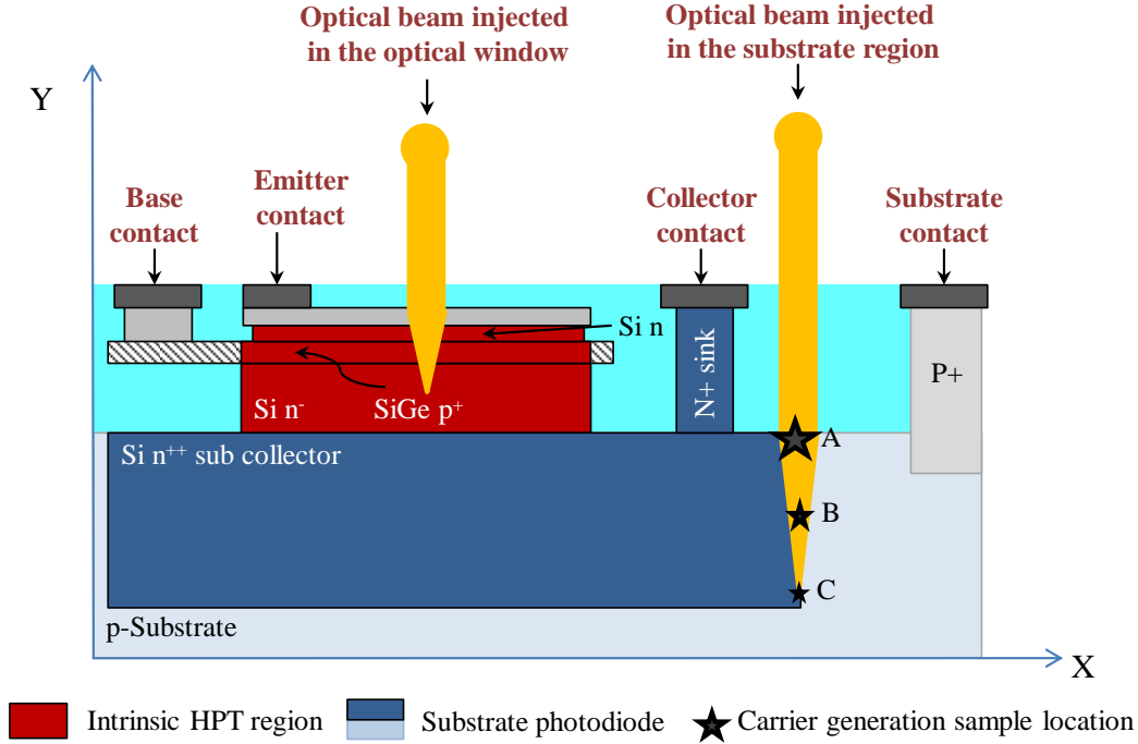
Figure 2-25: The phototransistor structure cross section along X and y plane. The intrinsic and the substrate photodiode regions are indicated, and also the expected light penetration region are shown in the intrinsic and substrate regions.
