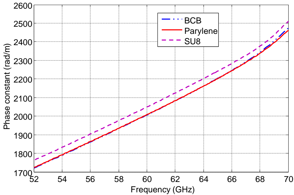
Figure 4-6: The imaginary part of the propagation constant of coplanar line versus frequency with 16 \mu m polymer layer and line dimensions for 50 \Omega characteristic impedance extracted from the HFSS simulator.
