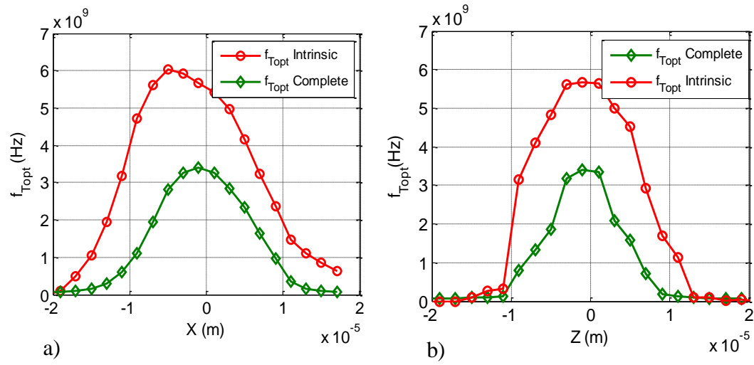
Figure 3-52: The raw and extracted f_{T_{opt}} a) at z=0\mu\text{m} , b) at x=0\mu\text{m} of the 10 \times 10 \mu\text{m}^2 HPT.
