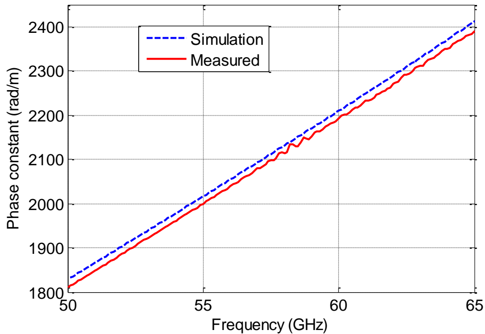
Figure 4-45: The measured and simulation phase constant of the fabricated coplanar line having a strip width of 108\mu\text{m} a slot width of 19\mu\text{m} and with a SU8 thickness of 16\mu\text{m} .
