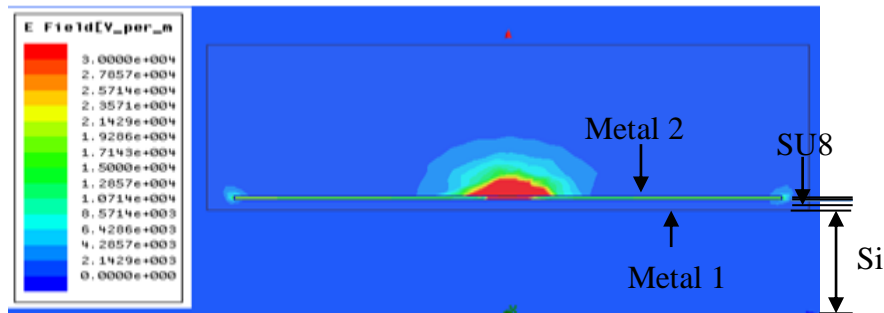
Figure 4-19: Electric field amplitude (V/m) in the transverse plane of the grounded coplanar line on low resistive silicon substrate with SU8 layer and a strip width of 80\mu\text{m} .
