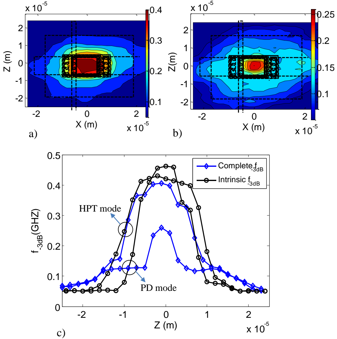
Figure 3-50: Opto microwave -3dB frequency a) The complete HPT topological map in HPT mode, b) The complete HPT topological map in PD mode and c) the complete and intrinsic slice curves at X=0 in PD and HPT modes, of the 10 \times 10 \mu\text{m}^2 HPT.
