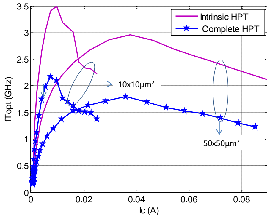
Figure 3-20: The complete and intrinsic optical transition frequency versus collector current for 10 \times 10 \mu\text{m}^2 and 50 \times 50 \mu\text{m}^2 HPTs at V_{ce}=2\text{V} .
