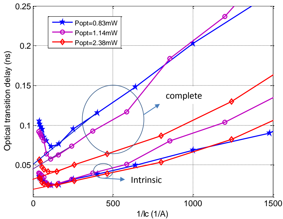
Figure 3-62: Global optical transition delay of the 10 \times 10 \mu\text{m}^2 HPT versus 1/IC at different optical power levels before and after substrate effect corrected.
