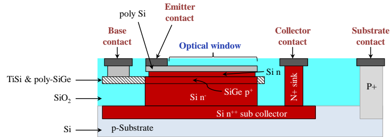
Figure 3-40: Phototransistor structure under study.
