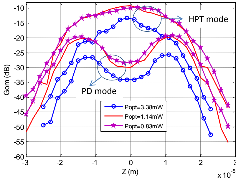
Figure 3-58: The slice figure of low frequency G_{om} in PD and HPT mode at x=0\mu\text{m} and different injected optical power levels on the 10\times10\mu\text{m}^2 HPT.
