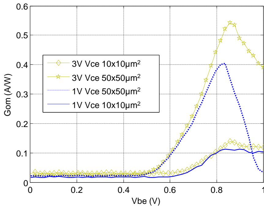
Figure 3-6: Low frequency complete opto microwave responsivity versus base voltage. of 10 \times 10 and 50 \times 50 HPTs at different collector voltages with injected optical power of 2.38mW.
