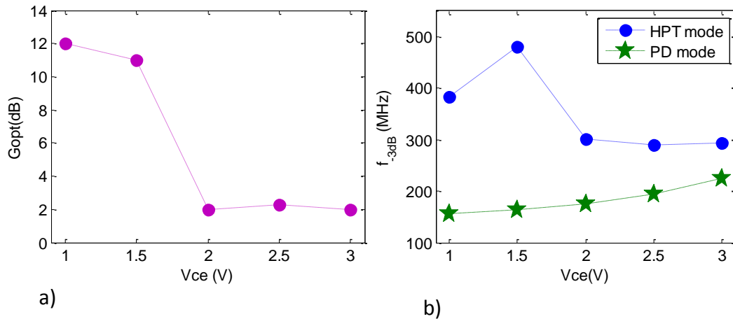
Figure 5-9: a) Optical gain versus V_{ce} , b) cutoff frequency versus V_{ce} in PD and HPT mode ( V_{be}=0.8V ).
