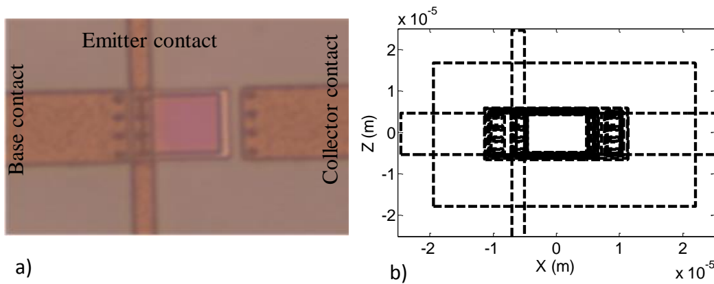
Figure 3-34: a) Top view of the 10 \times 10 \mu\text{m}^2 phototransistor. b) The layout of the HPT with optical window at the center of the optical probe position coordinate system. X and Z are given in meter.
