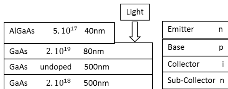
Figure 1-26: Schematic diagram of an npn GaAs/AlGaAs phototransistor.
