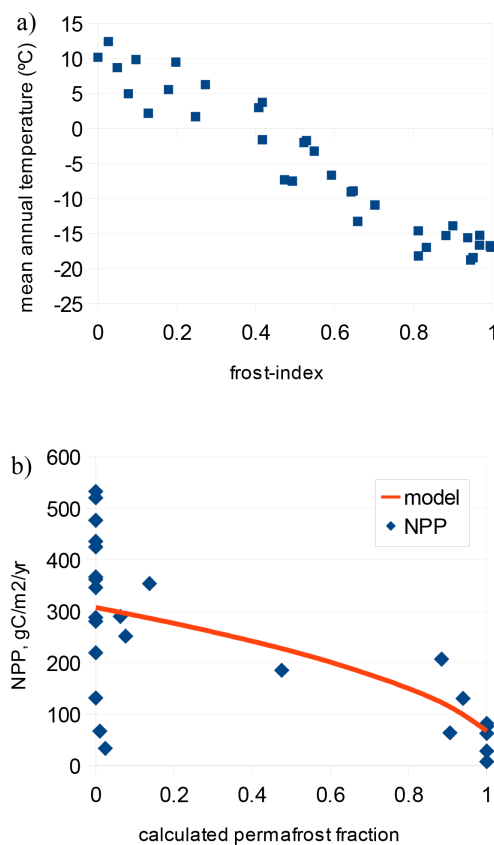
Figure A2. Relationships between frost index and MAT on the CLIMBER-2 grid scale (data from Zhang, 1998; Jones et al., 1999). Frost index determines permafrost fraction according to the model described in Sect. 3.2 (main text). NPP data for the permafrost zone from MODIS plotted against permafrost fraction (calculated from frost index values of Zhang, 1998) on the CLIMBER-2 grid scale.
