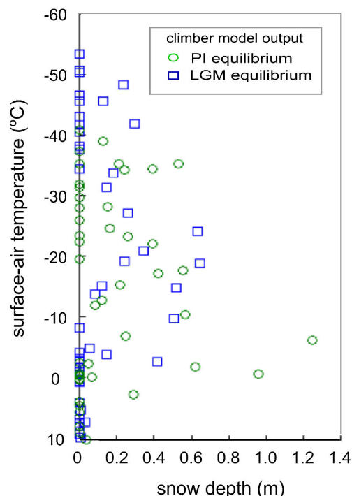
Figure B3. CLIMBER-2 model output for snow depth (m) plotted against surface air temperature (°C) for the PI(eq) (green circles) and LGM(eq) (blue squares) climates. Model output does not show extreme conditions for snow cover due to the very large grid-cell size.
