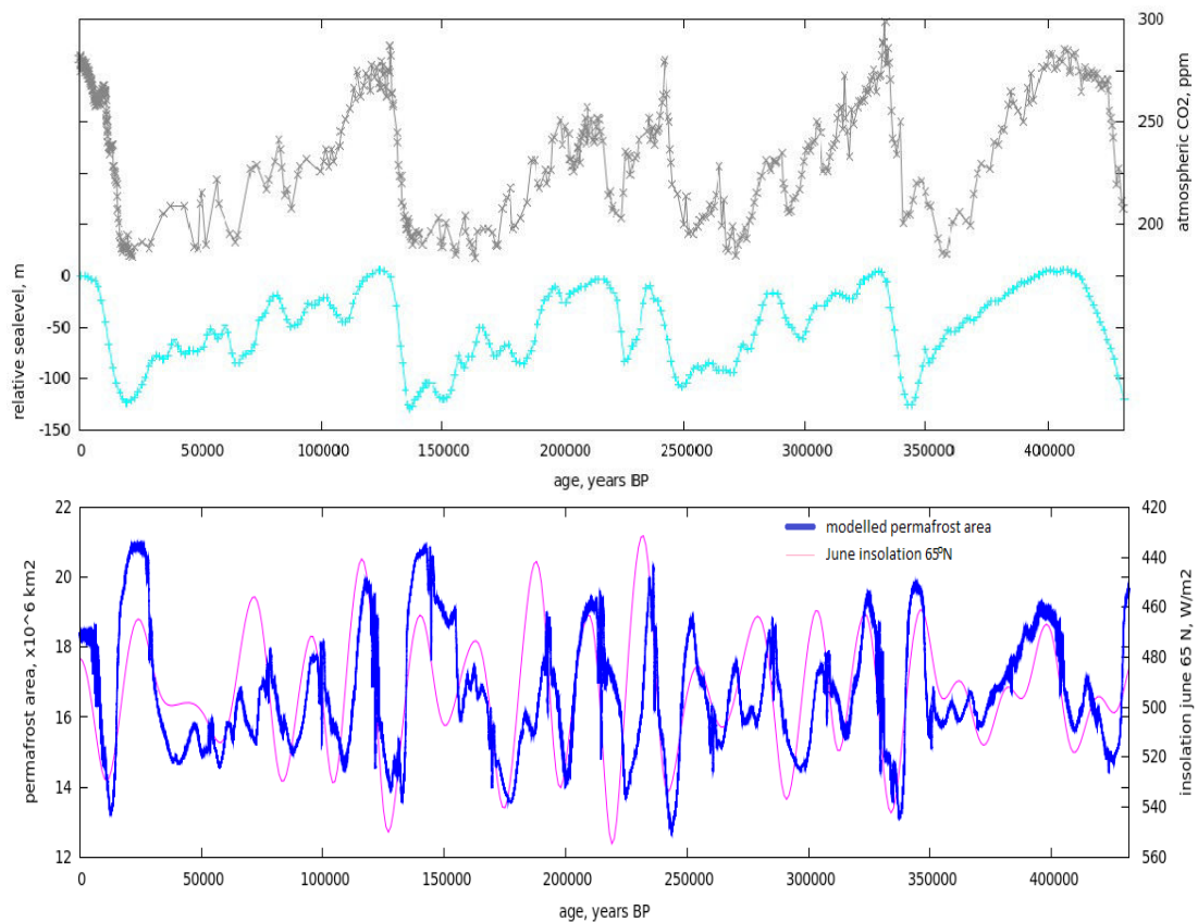
Fig 5.6, Top: model drivers for CO_{2\_RAD} (Luthi et al 2008) and relative sea-level (Peltier 1994). Bottom: Modelled permafrost area for the 432kyr simulation, overlaid on June insolation 65°N (Laskar et al 2004), inverted scale.
