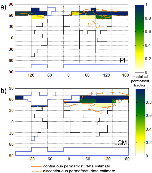
Figure 14. Modelled permafrost area for (a): PI(tr) simulation, (b) LGM(eq) simulation for LOW-MEDIUM permafrost area. Overlaid in orange are data estimates from Circumpolar Atlas (Jones et al., 2009) for the present day, Vandenberghe et al. (2008) for LGM Eurasia, French and Millar (2013) for LGM N. America.
