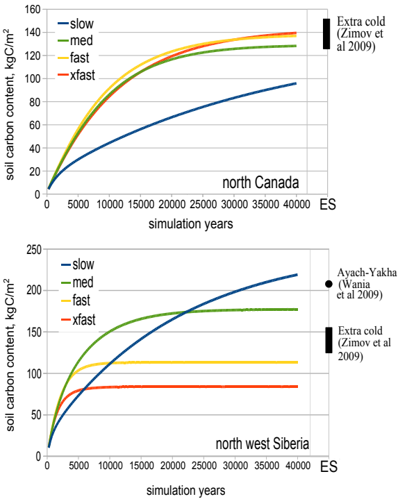
Figure 15. Modelled PI(eq) simulation output for total soil column carbon content for two grid cells. ES is equilibrium state ( > 50 kyr).
