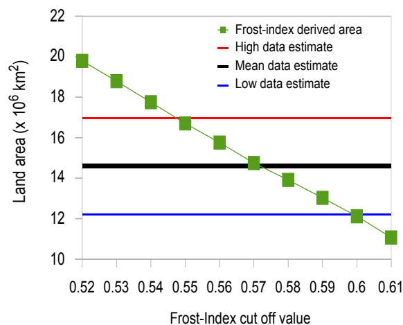
Figure 8. Total land area with a frost index higher (colder) than the x axis cut-off value, for frost-index data from Zhang (1998) (NSIDC). Horizontal lines show the Zhang et al. (2000) data estimates for area of land underlain by permafrost.
