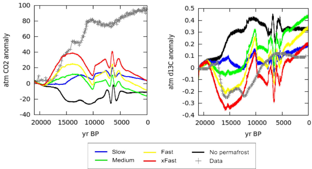
Fig 4, Clim and Perm modelled atmospheric CO 2 (left) and \delta^{13}\text{C} (right). Data for CO 2 is Monnin et al (2001), \delta^{13}\text{C} is Schmitt et al (2012). All data plotted with respect to the LGM value.
