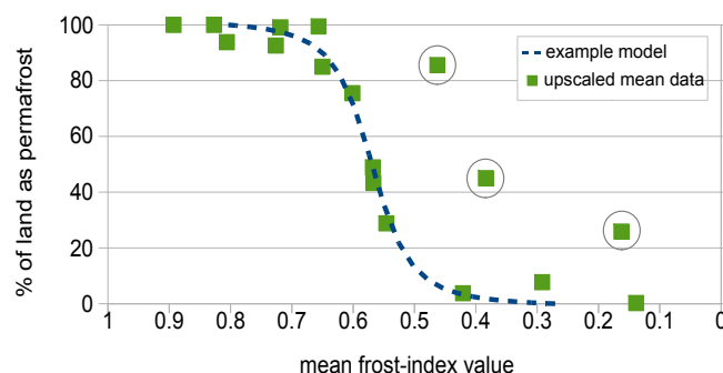
Figure 10. Frost-index-predicted permafrost fraction of land from Fig. 8 upscaled to the CLIMBER-2 grid and plotted against mean frost index for the same CLIMBER-2 grid cell. Circled points are where the total fraction of land vs. ocean in the grid cell is small (land is less than 25 % of the grid cell) and ocean temperatures pull frost index lower (warmer). The dashed line is a representative relationship between frost index and permafrost land fraction.
