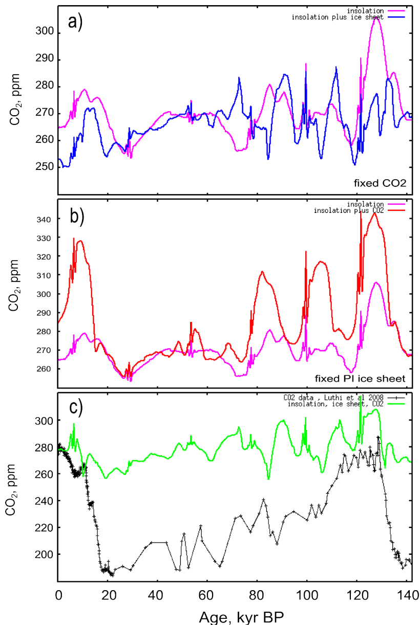
Fig 5.3, Modelled atmospheric \text{CO}_2_{cc} per simulation. a) insolation only and insolation plus ice sheet, b) insolation only and insolation-plus- \text{CO}_2 , c) insolation, ice sheet and \text{CO}_2 (combined) simulation, with \text{CO}_2 data from Luthi et al 2008.
