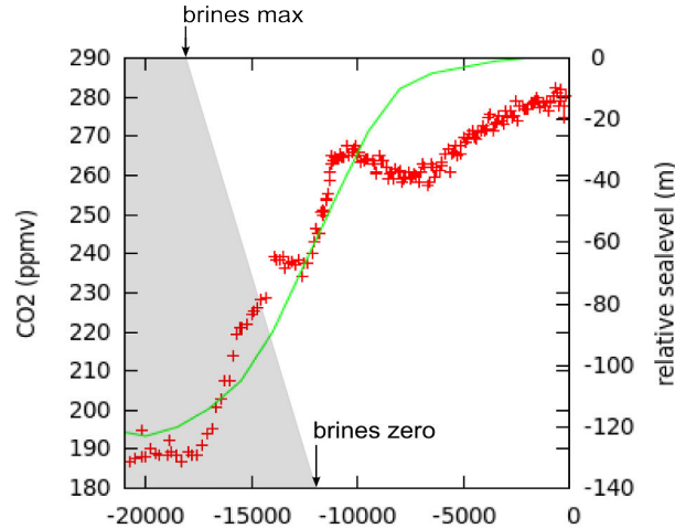
Fig 2, Drivers for the last deglaciation, red crosses: atmospheric \text{CO}_2 to drive the radiative code (Monnin et al 2001), green line: relative sea-level for ocean volume and ice sheet extent (Peltier 1994), grey shaded: brines controller; maximum at 18kyr BP with linear reduction to zero at 12kyr BP, as Bouttes et al (2012).
