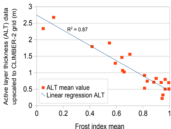
Figure 7. Measurement data for active layer thickness (CALM network, Brown et al., 2003) and frost index (Zhang, 1998) upscaled to the CLIMBER-2 grid scale, showing the distinct relationship of reducing active layer with increasing frost index at this scale. Note that permafrost fraction is calculated from frost index in our model (see Sect. 3.2).
