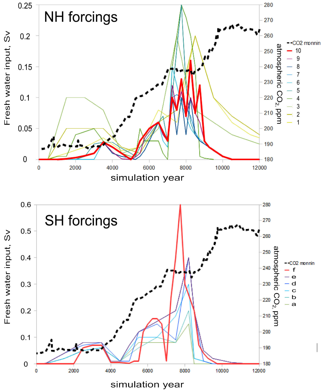
Fig 2, Forcing profiles plotted per hemisphere forcing. The CO 2 record is a comparison to show the timing of maximum FWFs.
