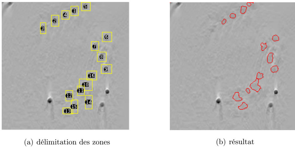
FIGURE 4.5 — L'algorithme snake .
