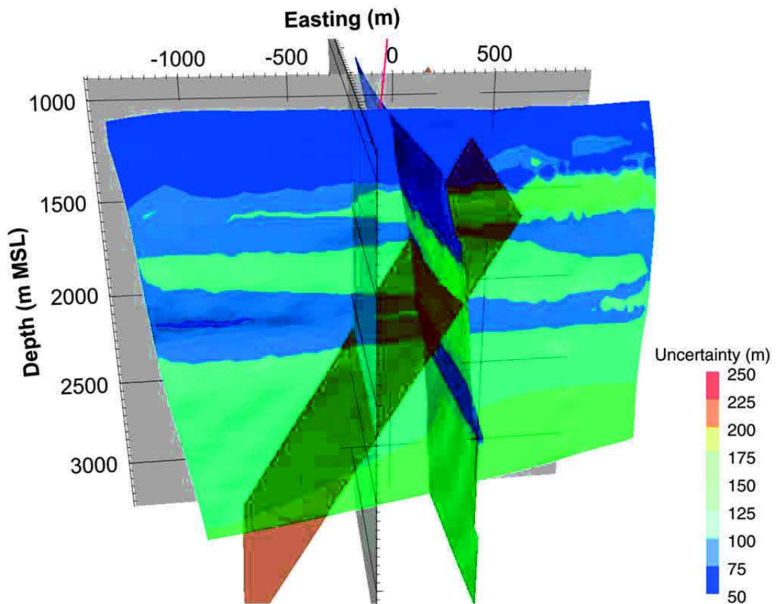
Figure 5-17: 3D view of the relocation, by the 16-station network, of the synthetic events initially located on the horizontal plane and along the fault (top) and on the N-S and E-W vertical plane (bottom). The initial locations were on the grey planes whereas the relocations are on the coloured planes. The colour scale is associated with the largest uncertainty value which varies between 50 m and 250 m. The location of the fault is shown by the brown plane (bottom). Same display as Figure 5-14.
