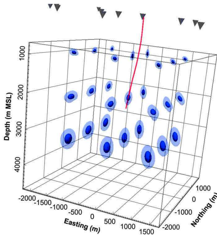
Figure 5-6: 3D view of the relocation uncertainties at 68.3% (dark blue) and 99.7% (light blue) confidence levels of 27 sources distributed around GRT1 well (red curve). Part of the seismic stations is also displayed (grey cones).
