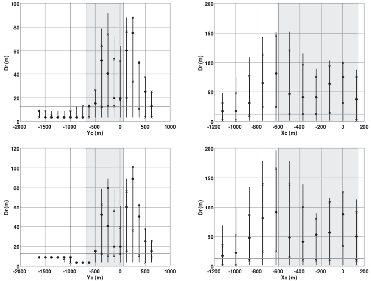
Figure 10-6: Boxplots showing total inaccuracies for location computed with the combined network (top panels) and the down-hole network alone (bottom) with data from a synthetic modelling in a profile with a LVZ. The locations were carried out in the reference velocity model. The location were computed for sources on vertical- Y_c plane (left), vertical- X_c plane (right) and horizontal plane (not shown). The perpendicular grey-line accounts for the mesh size used for the location and the shadowed zone corresponds to the simulated injection zone. The symbols concerning the boxplots are described in Figure 10-3.
