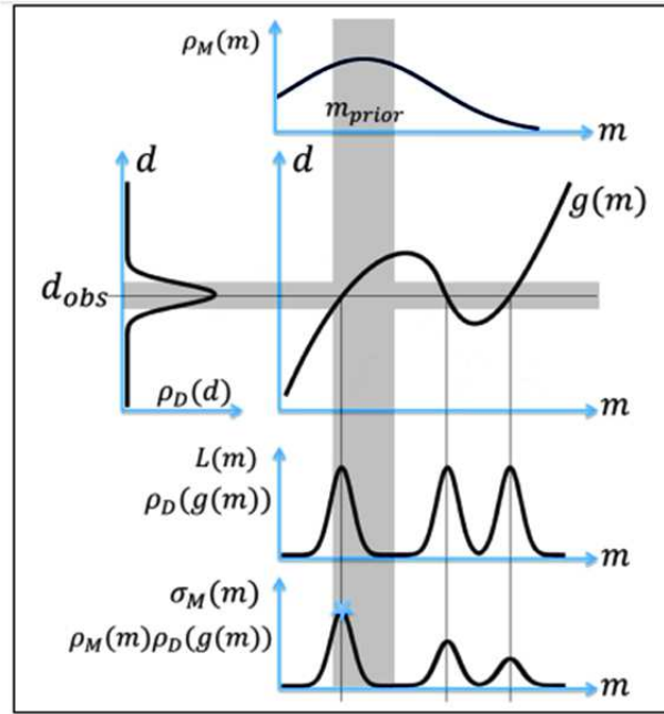
Figure 2-1: Schematic representation of the method proposed by Tarantola concerning the different states of information and their combination. The horizontal axes called “ m ” represent the model space whereas the vertical axes, called “ d ” account for the data space. The function g(m) introduces the theory relating both. For this example, it is assumed to be perfect. The probability densities for the a-priori model and for the observations are represented by \rho_M and \rho_D respectively. On those diagrams m_{prior} is the preferred model used a-priori and d_{obs} the most probable observation. The blue star accounts for the best fit model according to the data set. The grey horizontal (vertical) grey zone is the domain of acceptable data (parameters) values according to the associated uncertainties.
