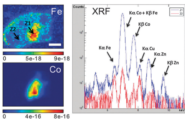
Fig. 6 Iron and cobalt distribution and abundance determined using SR-nXRF in a micro-alga exposed to 10^{-3} mol L -1 of cobalt. The micro-alga originates from the Co 10^{-3} M sample. Experimental conditions as in Fig. 2. (Fe), (Co): respective SR-nXRF quantitative distribution maps of the elements. The color bar indicates intensities in g pixel -1 ; the white scale bar in the Fe map represents 1 \mu m. Z1 and Z2 arrows indicate the center of two zones containing 5 \times 5 pixels. (XRF): summed XRF spectra for pixels in Z1 (blue) and Z2 (red) zones. K \alpha and K \beta peaks of the elements of interest are indicated on the spectra.
