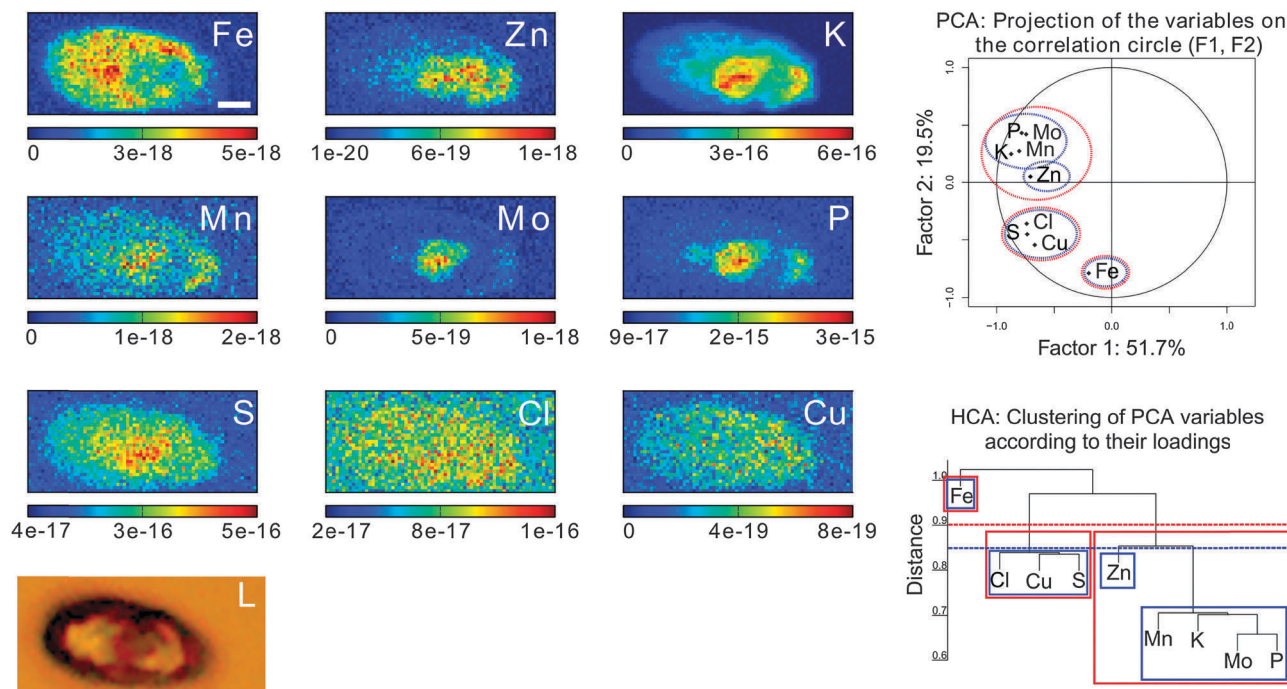
Fig. 2 Elemental distribution and abundance determined using SR-nXRF in a control micro-alga. The micro-alga originates from Control 1. Experiments were performed on beamline ID22NI at ESRF. (Fe), (Zn), (K), (Mn), (Mo), (P), (S), (Cl), (Cu): respective SR-nXRF quantitative distribution maps of the elements. The color bar indicates intensities in \text{g pixel}^{-1} ; each pixel is 100 \text{ nm} \times 100 \text{ nm} . The white scale bar in the Fe map represents 1 \mu\text{m} . (L): light microscopy picture of the analyzed cell. (PCA): projection of the variables used for PCA in the factor plane obtained with the first and second principal components. The PCA was performed on a data set representing all the analyzed cells in Control 1. The color circles show the clustering resulting from the HCA (HCA): hierarchical clustering analysis performed on the loadings of the elements on all the principal components. The horizontal lines and corresponding color boxes indicate threshold distances and their corresponding clusters.
