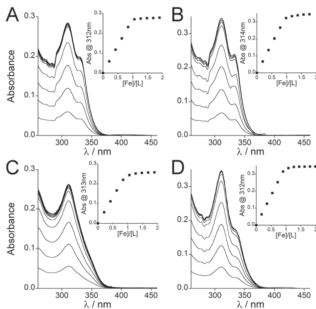
Fig. 2 UV-Vis absorption titrations under an inert atmosphere of (A) L ZR (44 μM), (B) L ZR lin (51 μM), (C) L TC (41 μM) and (D) L HSP (46 μM) by Fe 2+ in HEPES/NaOH buffer 20 mM pH 7.5, TCEP 250 μM, 298 K (path length = 1.0 cm). The insets show the evolution of the absorbance at \lambda_{max} (~310 nm) against the Fe 2+ /peptide ratio. All spectra were corrected for dilution and the spectrum of the apo-peptide was subtracted from each spectrum.
