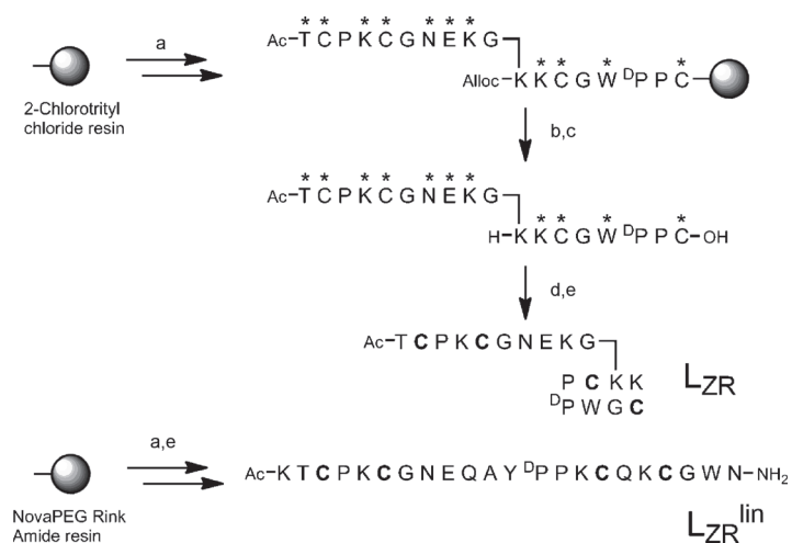
Scheme 1. Synthesis of L ZR and L ZR lin . a) Fmoc SPPS; b) [Pd(PPh 3 ) 4 ], PhSiH 3 , CH 2 Cl 2 ; c) CH 2 Cl 2 /TFA (99:1); d) 0.25 mM, PyBOP, DIEA, CH 2 Cl 2 ; e) TFA/TIS/H 2 O/DTT. * denotes the standard side-chain protecting groups.
