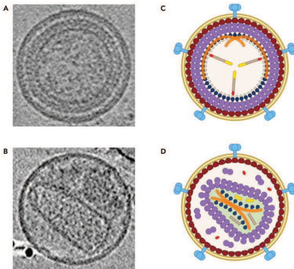
Figure 27: HIV-1 virion. Central slices through cryo-EM tomograms of immature (A) and mature (B) virus particles that are ~130 nm in diameter. Schematic representation of immature (C) and mature (D) HIV-1 particles (Balasubramaniam & Freed 2011).
