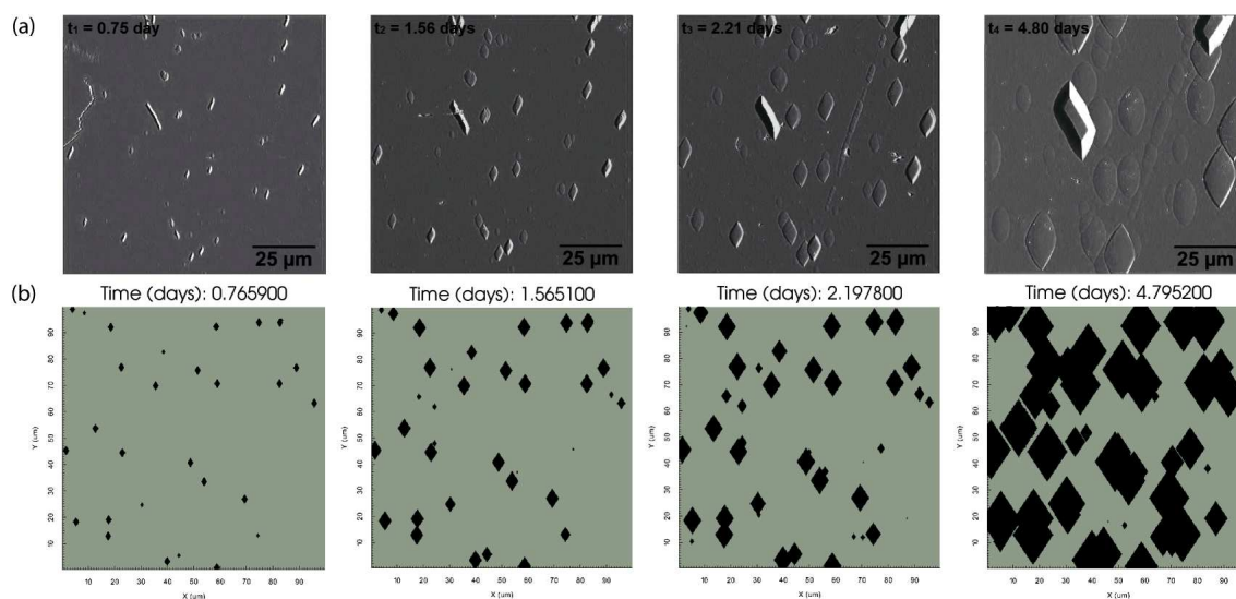
Figure XII.5: Evolution of the (001) orthoclase surface topography over the course of the dissolution process. (a) AFM images in deflection mode ( 100 \times 100 \mu\text{m}^2 ) of the surface evolution after 0.75, 1.56, 2.21 and 4.80 days of alteration. The images show the nucleation and growth of etch pits during the dissolution experiment carried out at 180^\circ\text{C} in an alkaline solution ( \text{pH}_{180^\circ\text{C}} = 9 ). (b) Numerical simulation of the (001) surface evolution. See text for details.
