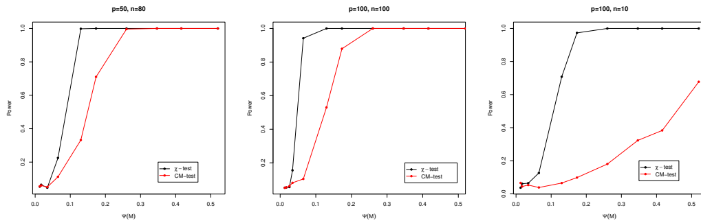
Figure 2.3 – Power curves of the \chi -test and the CM-test as functions of \psi(M) , when the alternative consists of matrices whose elements decrease polynomially when moving away from the main diagonal
