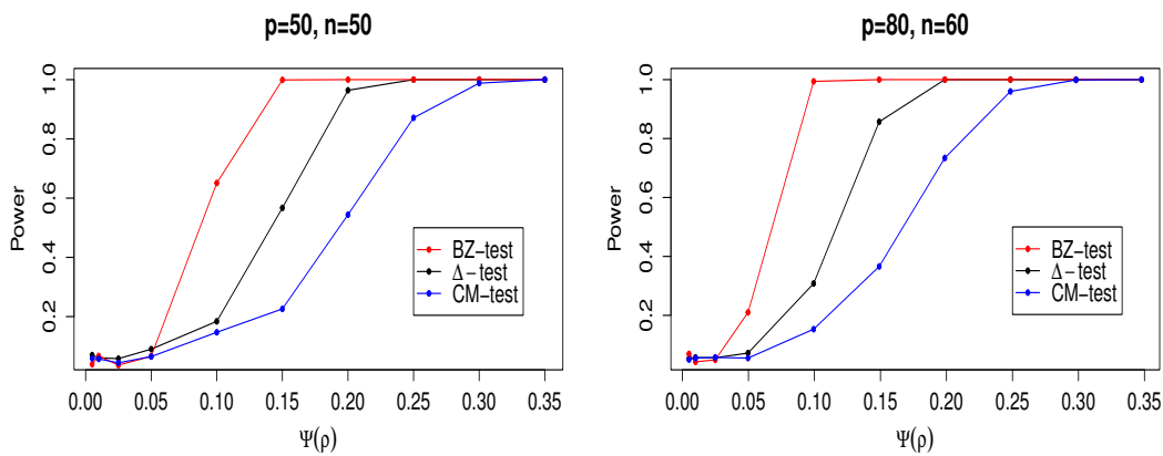
Figure 3.2 – Power curves of the BZ-test, \Delta -test and CM-test as function of \psi(\rho)
