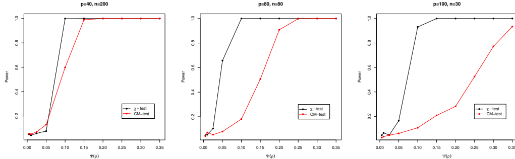
Figure 2.4 – Power curves of the \chi -test and the CM-test as functions of \psi(\rho) , when the alternative consists of tridiagonal matrices
