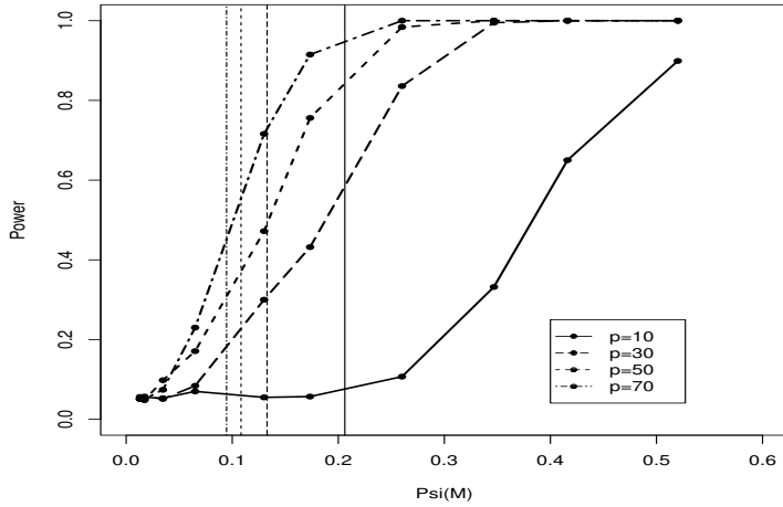
Figure 2.2 – Power curves of the \chi -test as function of \psi(M) for n = 10 and p \in \{10, 30, 50, 70\}
