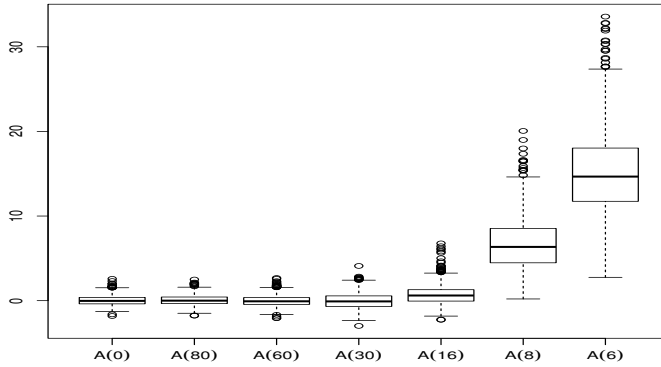
Figure 2.1 – Distributions of A(M) = n(p-T)\widehat{\mathcal{A}}_n^T for I = \Sigma(0) and \Sigma = \Sigma(M) , when p = 60 and n = 40 .
