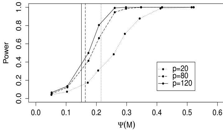
Figure 3.1 – Power curves of the \Delta -test as function of \psi(M) for n = 20 and p \in \{20, 80, 120\}
