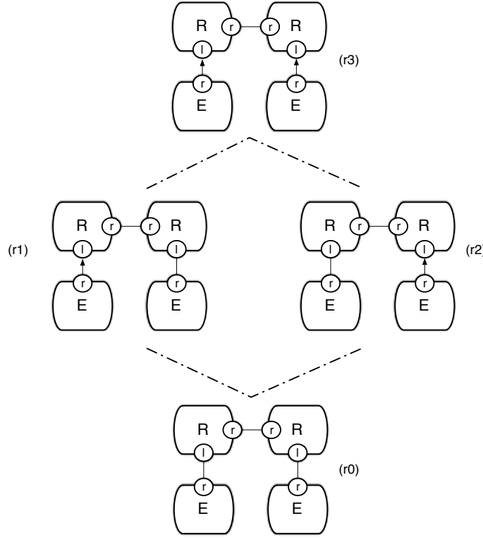
Figure 7.6: Lattice \mathcal{C} .
