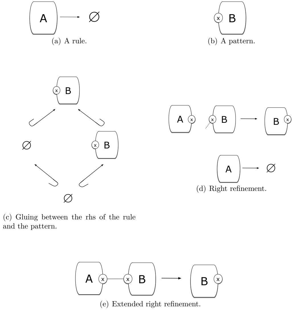
Figure 5.4: Production of a pattern.
