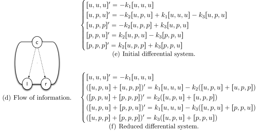
Figure 6.1: Chemical reactions, flow of information, and ODEs for the protein with hierarchical flow of information.
