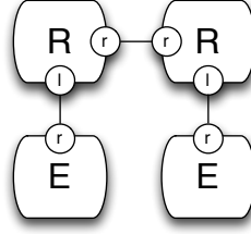
Figure 7.5: A dimer.
