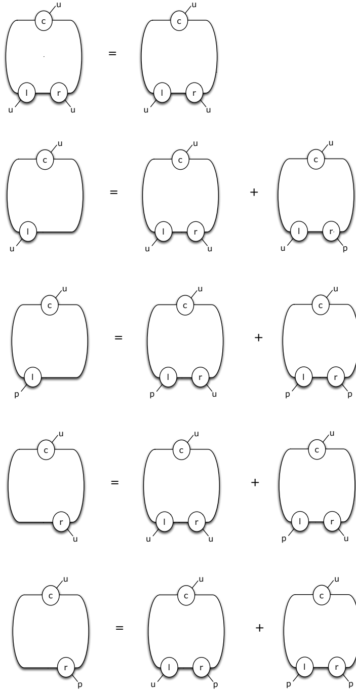
Figure 6.2: Change of variables.
