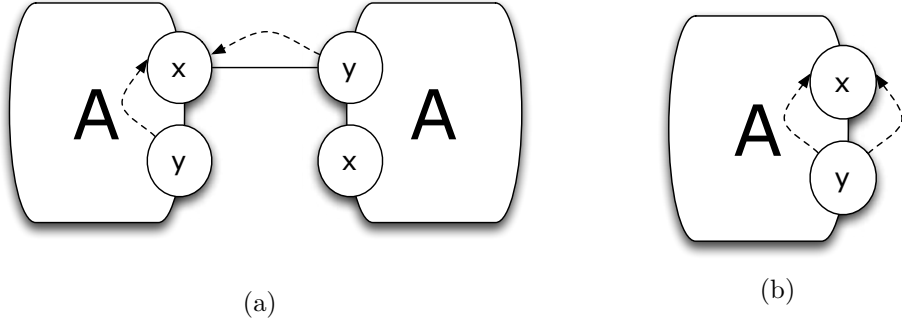
Figure 7.3: Example of annotated \Sigma -graphs.
