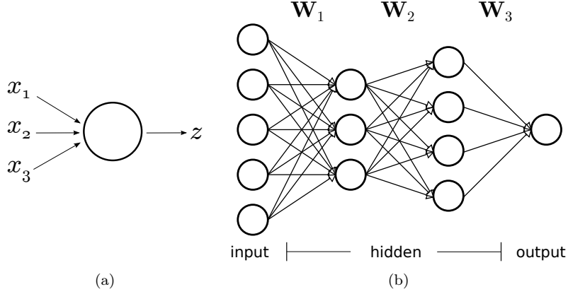
Figure 3.4: Illustrations of: (a) a perceptron with three inputs and (b) a 4-layered ANN architecture.
