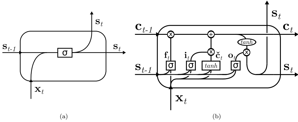
Figure 3.10: Internal structures of: (a) RNN and (b) LSTM units.
