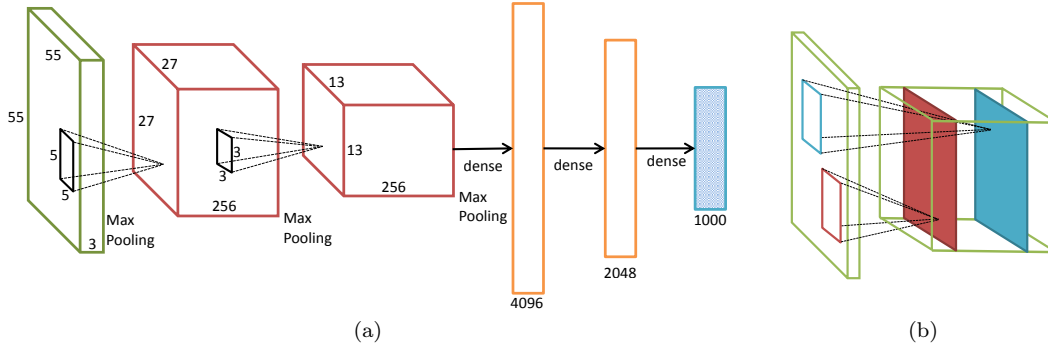
Figure 3.6: (a) CNN architecture example and (b) illustration of convolution layer.
