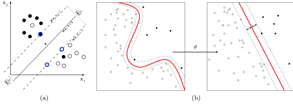
Figure 3.1: Illustration of: (a) linear SVM and (b) non-linear SVM with a kernel function.
