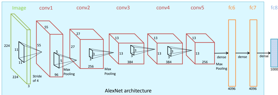
Figure 6.1: Illustration of the modified AlexNet architecture [Krizhevsky 2012].
