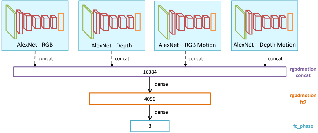
Figure 6.9: Multi-stream CNN architecture.
