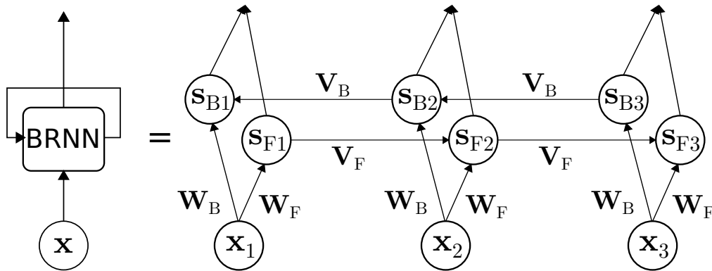
Figure 3.11: Unrolled bidirectional recurrent neural network (Bi-RNN). The number of unrolled elements corresponds to the length of the input sequence. In this case, we assume a sequence of length 3.
