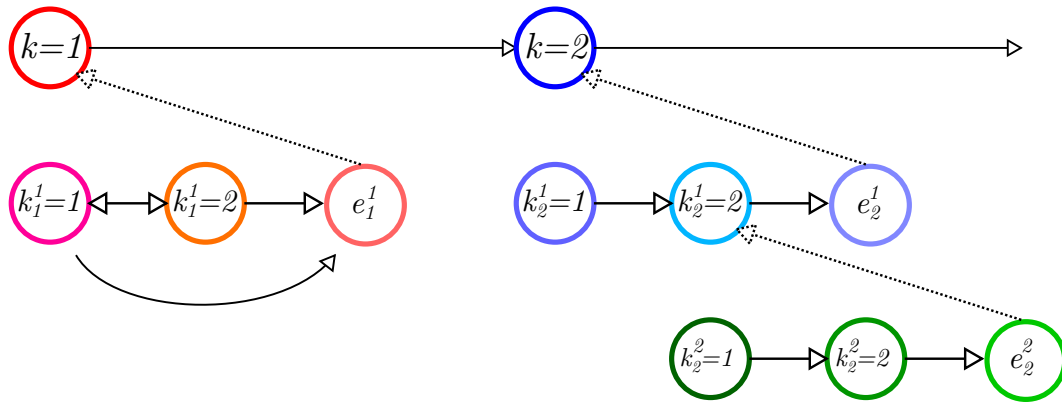
Figure 3.3: Illustration of a three-level hierarchical hidden Markov model. Grey and black edges respectively denote vertical and horizontal transitions. Dashed edges denote returns from the end state of each level to the level’s parent state. Note that the production states are not shown in this illustration and only some third-level states are shown, while in practice all the second-level states are represented by a probabilistic model as well.
