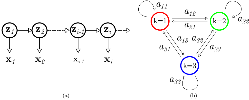
Figure 3.2: Illustration of Markov models: (a) hidden Markov model (HMM) and (b) state transitions in HMM.
