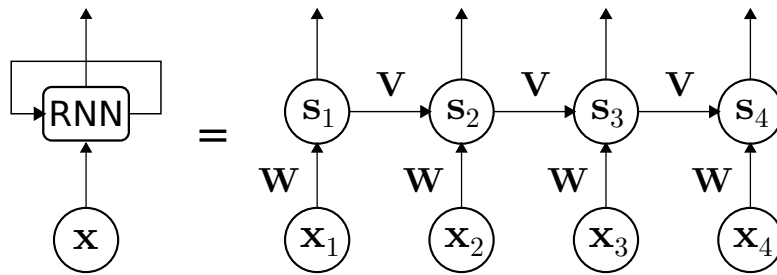
Figure 3.9: Unrolled recurrent neural network (RNN). The number of unrolled elements corresponds to the length of the input sequence. In this case, we assume a sequence of length 4.
