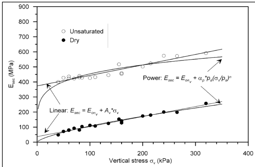
Figure I.34. Secant modulus vs. vertical stress for the unsaturated and dry materials at 5% water content and dry (Caicedo et al., 2009)
