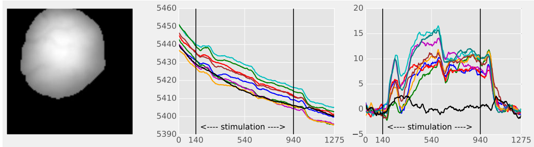
Figure 2.3: Left: the region of interest selected using r_{\text{thresh}} . Middle: the temporal traces of each condition averaged over all pixels and repetitions. Right: the temporal traces after preprocessing.
