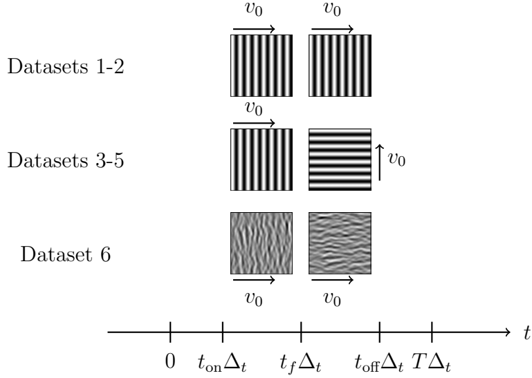
Figure 2.1: The 3 different protocols used to collect the data. The sampling time is \Delta_t whereas t_{\text{on}}, t_f, t_{\text{off}} and T are integers corresponding respectively to the frames numbers of stimulus onset, stimulus rotation, stimulus offset and recording offset.
