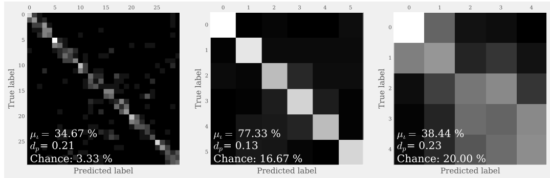
Figure 4.1: Dataset D^{(2)} . Confusion matrices \Lambda (left) and its reduction to orientation \Lambda^{(0)} (center) and to orientation bandwidths \Lambda^{(1)} (right).
