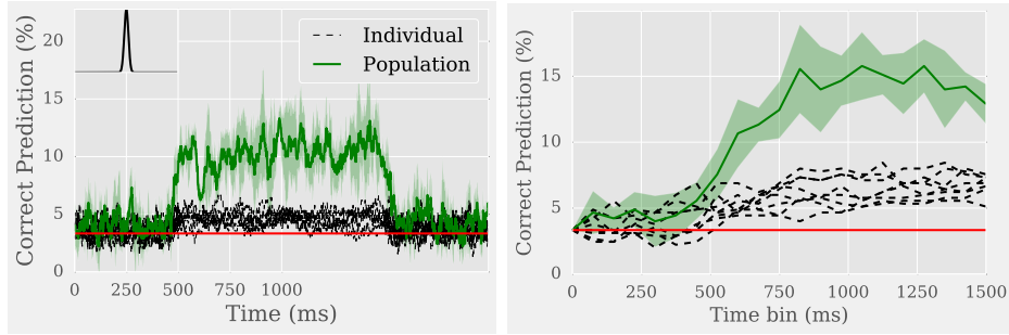
Figure 6.4: Simulated dataset 1. Left: the scores \mu_{\nu,t} for all t \in \mathcal{T} . Right: the scores \mu_{\nu,<t} for all t \in \{0, \dots, t_{\text{off}}\Delta_t\} . The red line represents the chance level.
