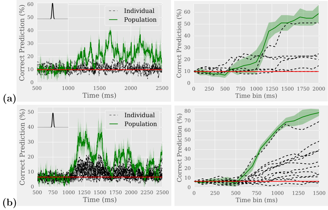
Figure 5.2: Left: the scores \mu_{\nu,t} for all t \in \mathcal{T} . Right: the scores \mu_{\nu,<t} for all t \in \{0, \dots, t_{\text{off}}\Delta_t\} . The red line represents the chance level. (a) Dataset D^{(5)} (b) Dataset D^{(6)} .
