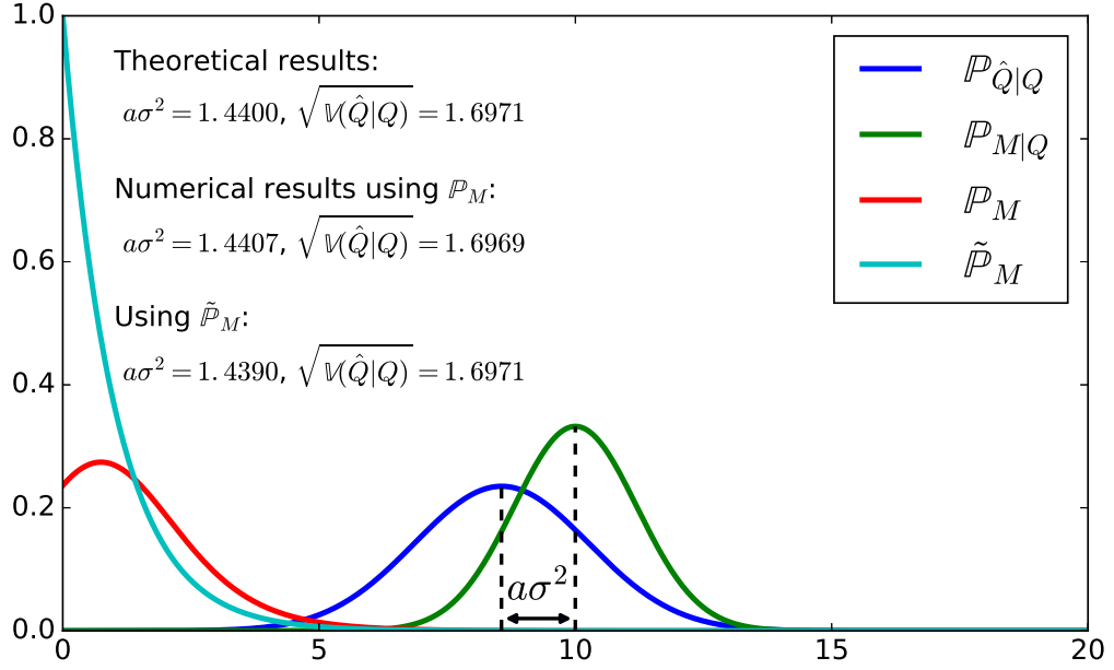
Figure 2.3: Numerical simulation of Proposition 13. The blue curve is obtain using \mathbb{P}_M , however the numerical results displayed for a\sigma^2 and \sqrt{V(\hat{q}|q)} indicates that the results for \mathbb{P}_{\hat{Q}|Q} is very close when computed using \tilde{\mathbb{P}}_M .
