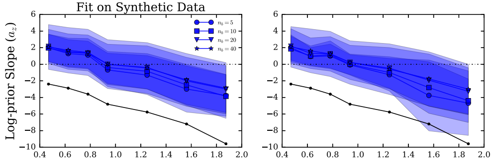
Figure 4.4: On the left the prior slope \hat{a} obtained after the first optimization step 4.1, on the right the prior slope \hat{a} obtained after the third optimization step 4.1. These estimations are represented for different numbers of block with one standard deviation error. The black line represents the ground truth values of the prior slopes used to generate the synthetic data.
