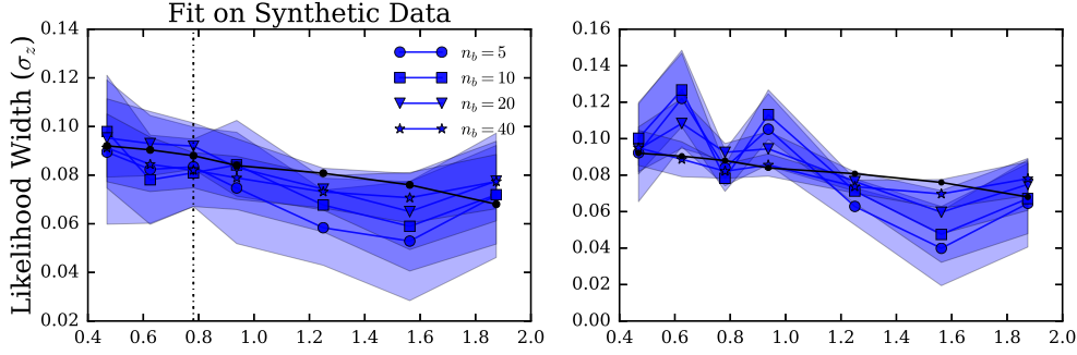
Figure 4.3: On the left the likelihood width \hat{\sigma} obtained after the first optimization step 4.1, on the right the likelihood width \hat{\sigma} obtained after the third optimization step 4.1. These estimations are represented for different numbers of block with one standard deviation error. The black line represents the ground truth values of the likelihood widths used to generate the synthetic data.
