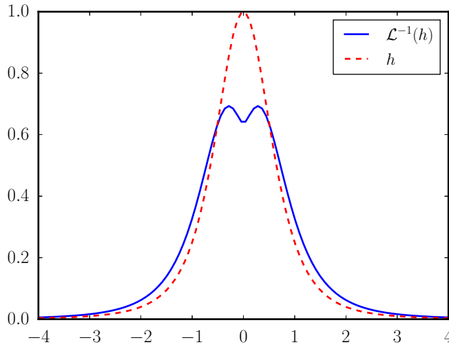
Figure 3.1: Functions h and \mathcal{L}^{-1}(h) .
