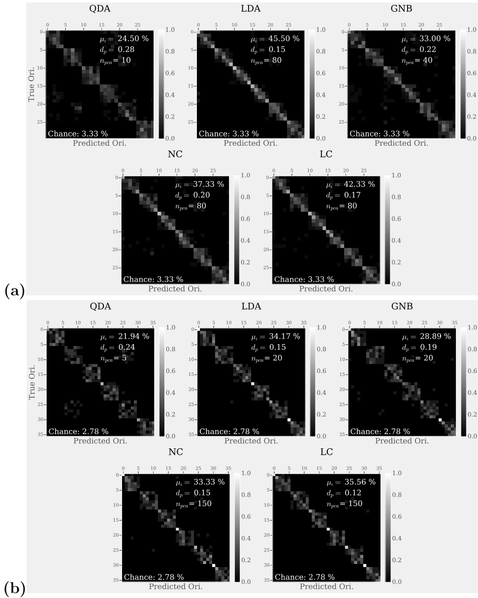
Figure 3.5: Confusion matrices \Lambda and distance d_p (defined in 9) obtained for each algorithm for dataset D^{(1)} (a) and D^{(3)} (b). QDA: Quadratic Discriminant Analysis. LDA: Linear Discriminant Analysis. GNB: Gaussian Naive Bayes. NC: Nearest Centroid. LC: Logistic Classification.
