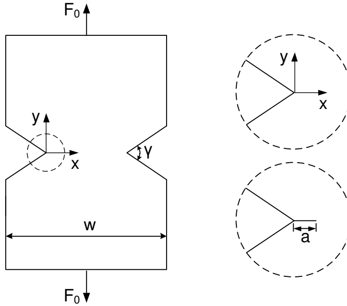
Figure 4.4: V-notched plate under tension loading and the corresponding emanating crack.
