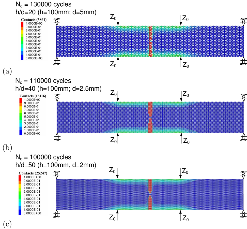
Figure 5.11: Damage distribution of a non-reinforced four point bending beam under applied strain \varepsilon = 150 \mu\text{m}/\text{m} for particle diameter (a) d = 5 \text{ mm} , (b) d = 2.5 \text{ mm} and (c) d = 2 \text{ mm} .
