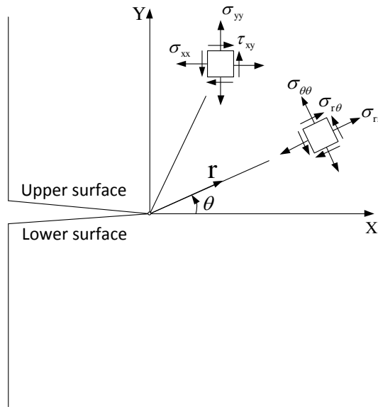
Figure 2.2: The rectangular and polar coordinate components of stress field around the crack tip (Modified from [8]).
