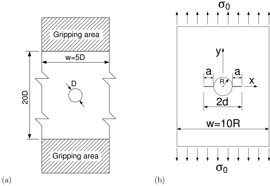
Figure 4.8: (a) Geometry of the plates with circular holes (modified from the illustration by [110]), and (b) the corresponding failure mechanism (two symmetric cracks emanating from two sides of the hole).
