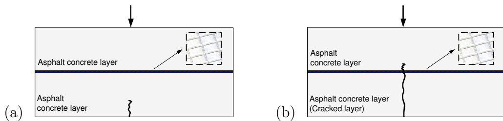
Figure 6.2: Crack initiates from the bottom of (a) the second layer and (b) the first layer.
