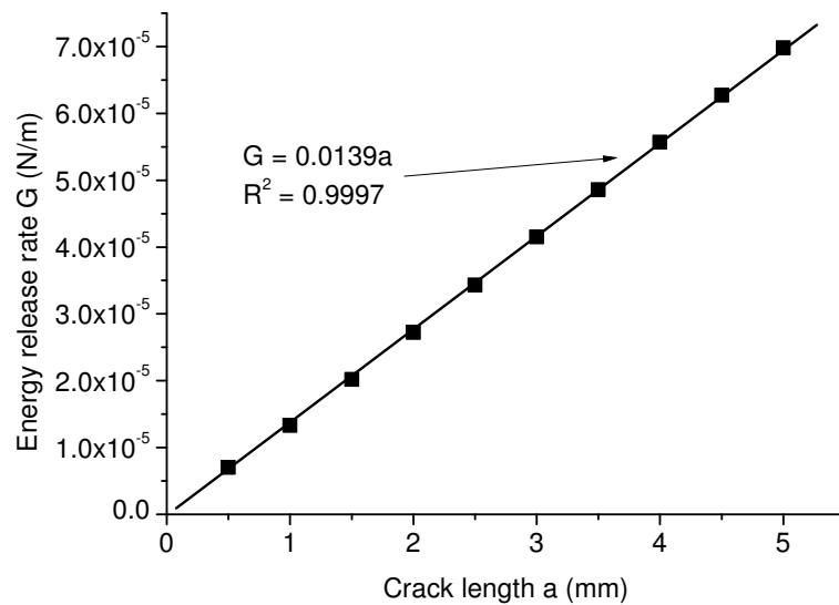
Figure 6.6: G versus a for crack initiation from the lower boundary of the second asphalt concrete layer (case 1).
