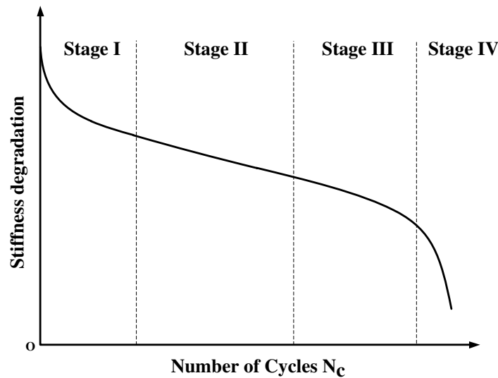
Figure 5.12: The four stages of the fatigue failure process.
