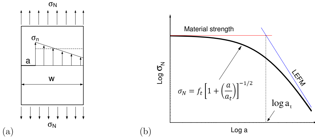
Figure 2.14: (a) An edge crack in a plate and (b) its nominal strength \sigma_N as a function of crack length a (modified from [17]).
