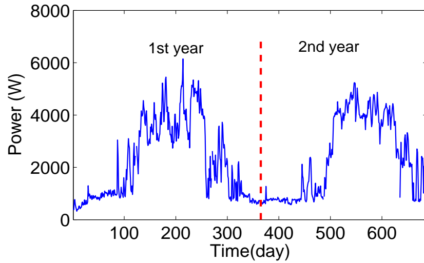
Figure 6.22: Power consumption of client no.17 during two years (July 01, 2004 ~ June 30, 2006). The vertical line separates the two-year period.
