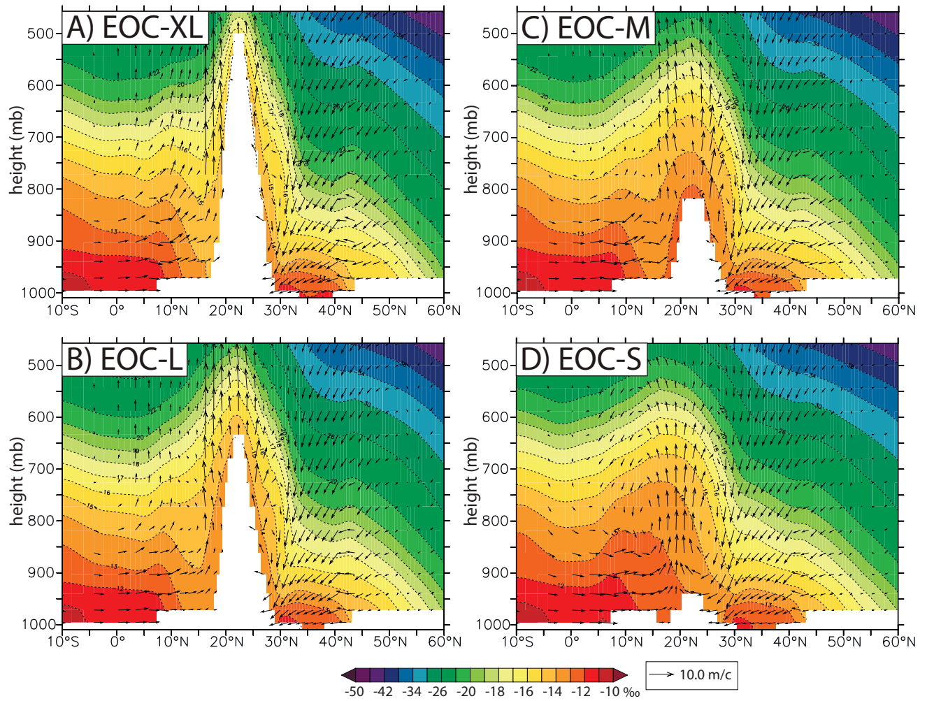
Extended Data Fig. 4. MJJAS \delta^{18}\text{O}_v and meridional-vertical wind velocities (m/c) for A) EOC-XL, B) EOC-L, C) EOC-M, and D) EOC-S simulations. Profiles are averaged between 72° E and 78° E for all Eocene simulations.
