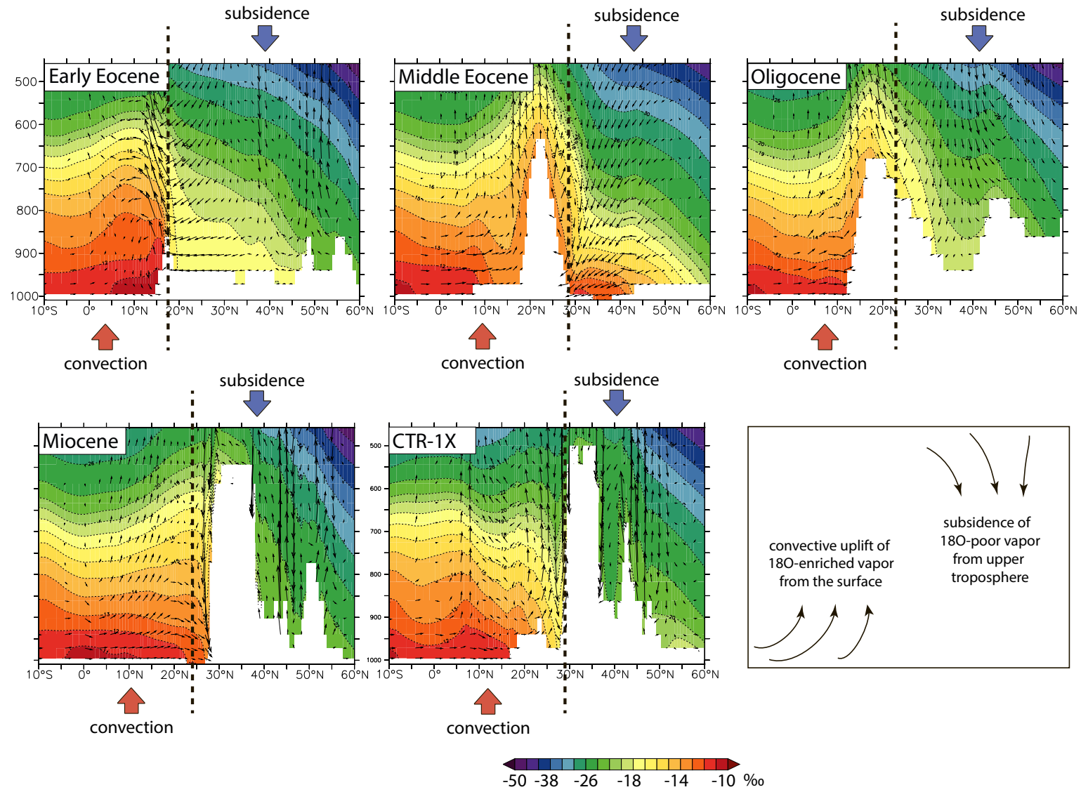
Figure 4.5 – MJDAS \delta^{18}\text{O}_v and meridional-vertical wind velocities for Early Eocene, Middle Eocene, Oligocene, Miocene and Control cases.
