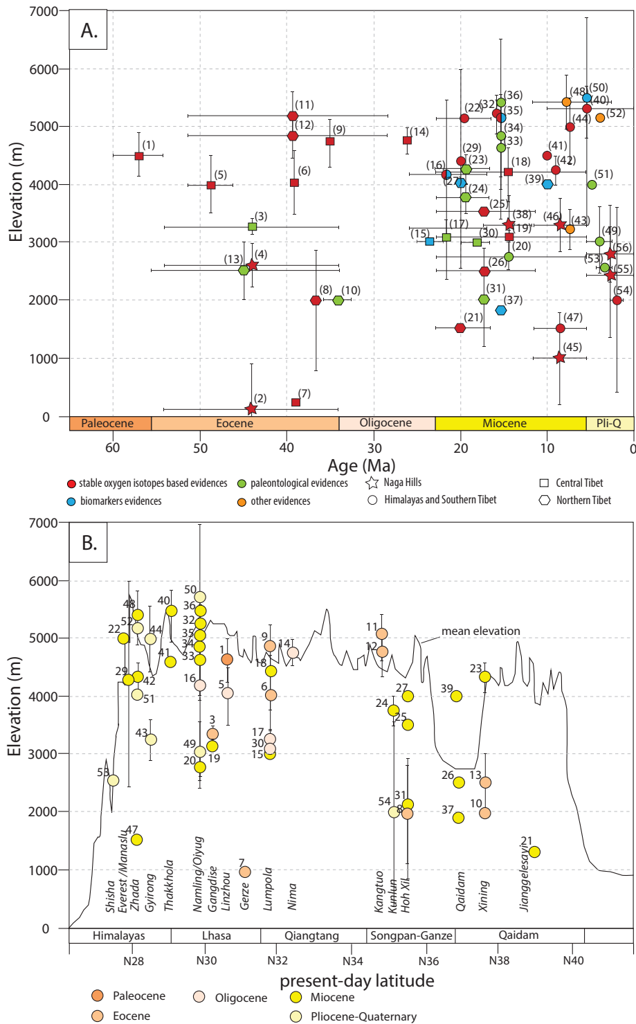
Figure 1.13 – A) Summary of paleoelevation evolution of the Himalayas and Tibetan Plateau region based on published quantitative estimates (see the compilation in the Table 1.1). Color shows the type of archive: red - stable oxygen isotopes evidences, green - palentological evidences, blue - biomarkers evidences, orange - other evidences. Geometry shows the location of sampling: stars - the Naga Hills (Liming and Chake basins), circles - the Himalayas and the Southern Tibet (Nanling, Oiyug, Zhada, Thakkhola, Gyirong, Everest, and Shisha basins); rectangles - the Central Tibet (Gangdise, Linzhou, Gerze, Nima, and Lumpola basins) polygons - the Northern Tibet (Kunlun, Kangtuo, Hoh Xil, Qaidam, Xining, Linxia, and Jianggelesayi basins). B) The S-N trending transect of the Himalayas and Tibetan Plateau . Ages are shown with different colors. Numbers on both figures corresponds to those in the Table 1.1 and on Figure 1.12.
