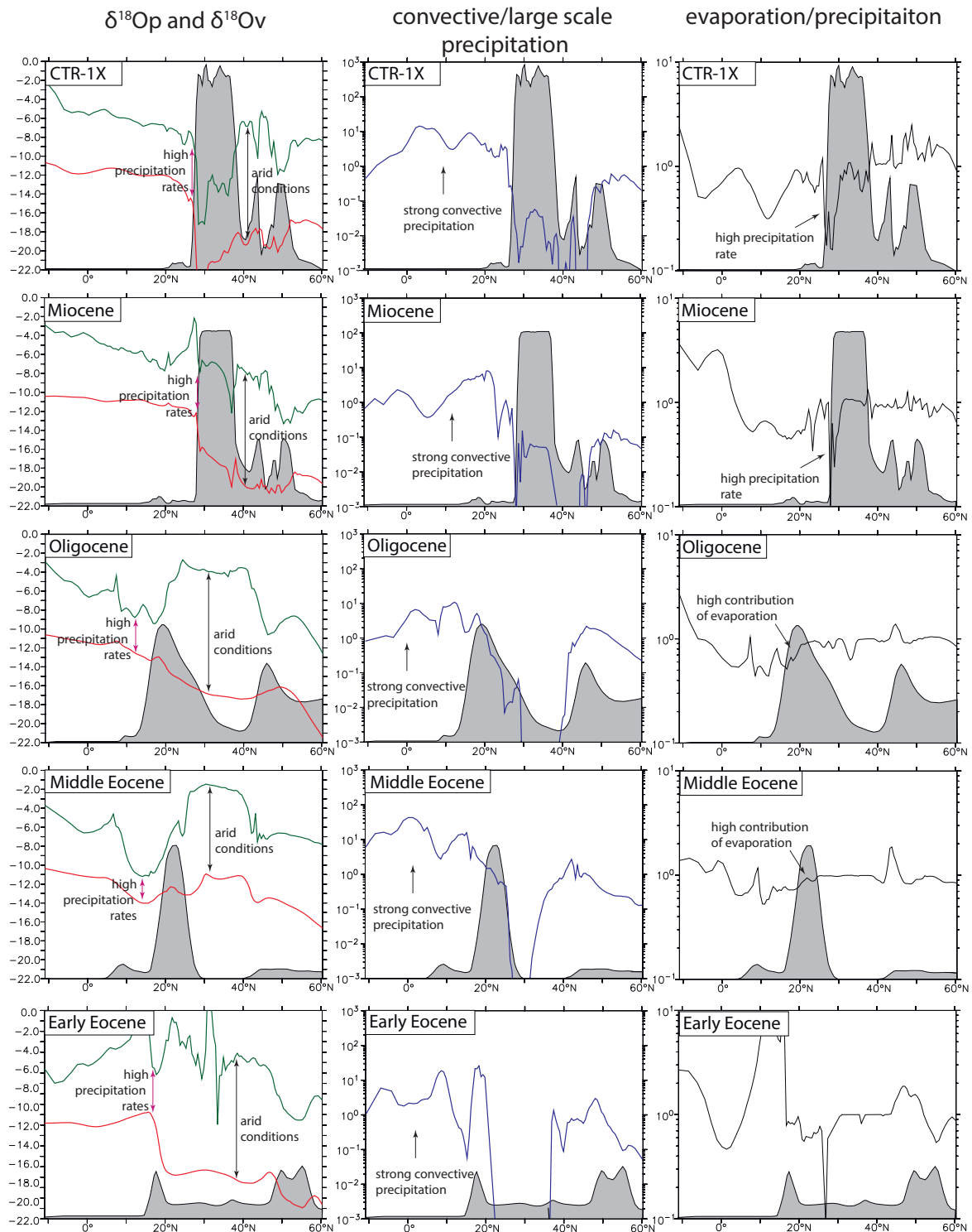
Figure 4.6 – South-North cross HTP sections for \delta^{18}\text{O}_v (red line), \delta^{18}\text{O}_p (green line), ratio between convective precipitation and large-scale precipitation (blue line) and the ratio between evaporation and precipitation (black line) for Middle Eocene, Oligocene, Miocene and Control cases. All variables are shown for MJJAS. Grey shade shows the topography for corresponding simulation.
