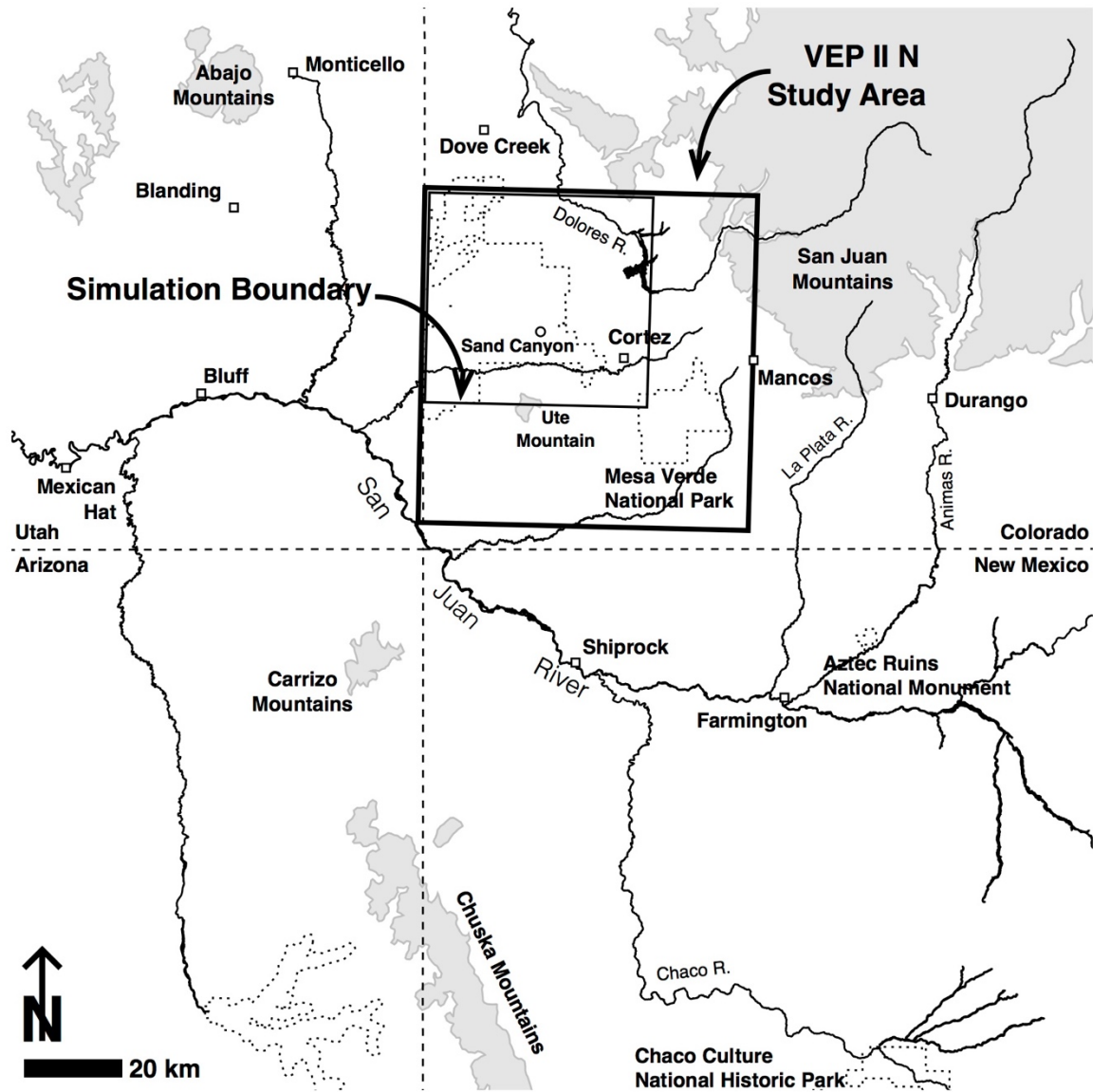
Figure 4.1. Location of the VEP I study area (shown by simulation boundary) within the VEP II N area, which encompasses the most populous portion of the central Mesa Verde region.
