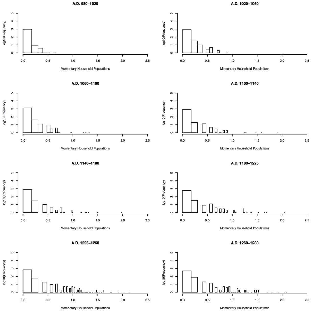
Figure S.4.0.2. PII-PIII momentary households by number of settlements in VEPIIN study area. Both axes logged.
