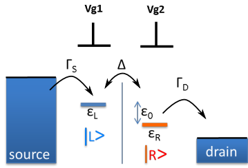
Figure 5.11 Scheme and notation used for the CAT.
