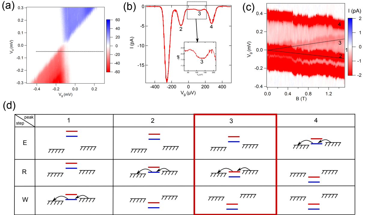
Figure 5.4 (a) diamond (in d.c. current) carried out at B=1.5 \text{ T} , without pulse. (b) current trace at V_d = -50 \mu\text{V} , along the black dotted line of (a), with pulse. The peak 3 (inset) corresponds to the current in the up state, as described in Fig. 5.3. (c) Current vs. magnetic field and gate voltage. The peak 2 and 3 are separated by the Zeeman energy as expected. (d) Sum-up for each peak (1 to 4) of the dot configuration, at each step of the pulse.
