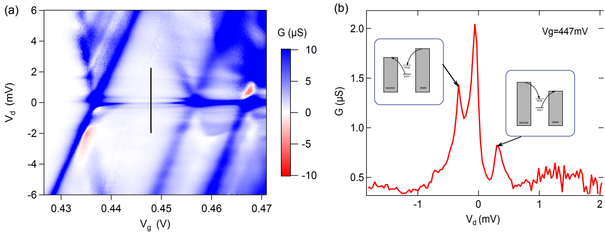
Figure 2.13 (a) diamond (differential conductance) recorded at V_b = 9\text{ V} with no magnetic field. (b) Cut along the black line of (a) showing the Kondo ridge and the satellite peaks attributed to inelastic valley cotunneling.
