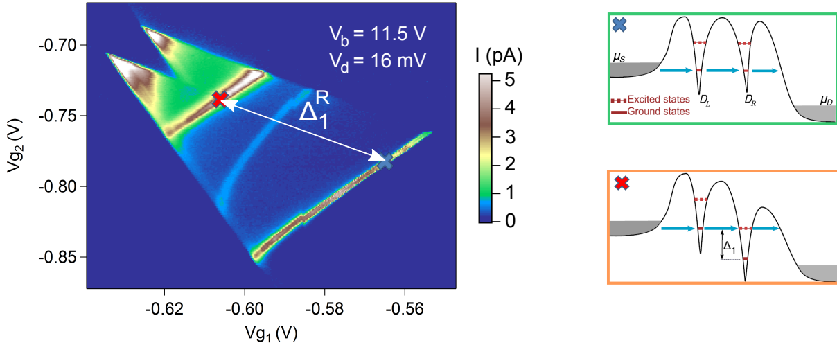
Figure 4.9 Same than Fig. 4.8 for a larger bias V_d = 16 mV. The line parallel to the baseline corresponds to the alignment of the ground state of the left donor and the first excited state of the right donor. We measured a valley splitting of about 10.3 meV.
