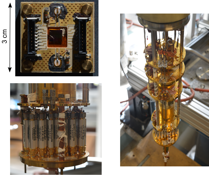
Figure 5.1 Pictures of the setup used for the high-frequency experiments. (top left) The sample holder with the RF connector (middle top and bottom), the DC connectors (middle left and right) and the resistance used for the bias-tee. (bottom left) The mixing chamber stage with the 80MHz-low pass filters. We also see the ends of the HF lines with a 3 dB attenuator. The thermal anchor is not shown. (right) The whole IVC stages.
