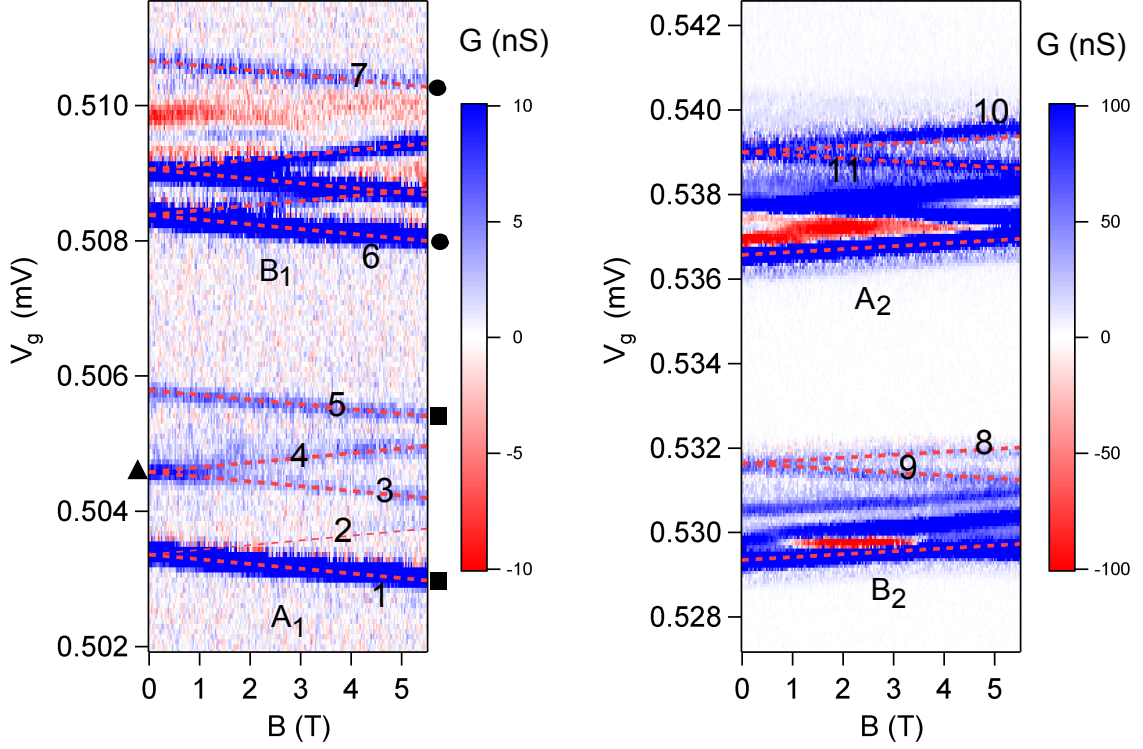
Figure 2.8 Magnetic field dependence of the first two electrons on dot A and B. We plot the differential conductance as a function of the field B and of V_g with a finite bias V_d = -2 mV, which corresponds to a cut along the red dotted line of Fig. 2.7. We evidence a spin 1/2 dependence (left) for the first electron on each dot and a singlet for the two-electron ground state (right).
