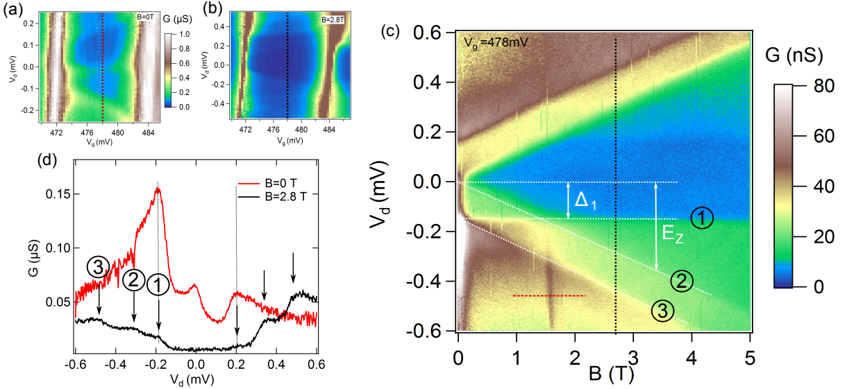
Figure 2.16 Magnetic field dependence of the Kondo and valley resonances. Sample #2. (a),(b) Diamonds at B=0 and 2.8 T. (c) Differential conductance vs. B and V_d . The spin Kondo vanishes with the magnetic field, but lines of different slopes appear, attributed to inelastic cotunneling process as explained in Fig 2.17. (d) SD conductance vs. V_d for B=0 and 2.8 T. At 2.8 T we observe the steps (labeled from 1 to 3) due to the inelastic cotunneling.
