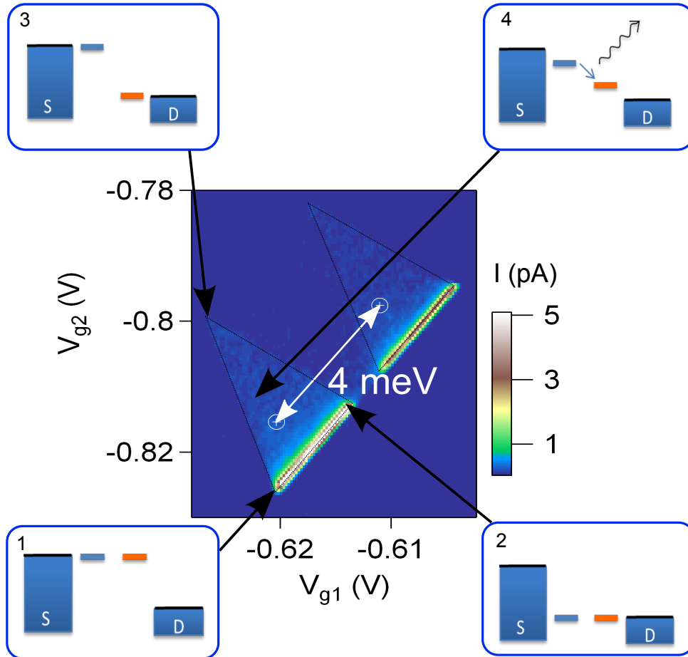
Figure 4.8 zoom on the circled region of Fig. 4.6. Here V_d = 3 mV. We observe a pair of triangles, characteristics of transport through two objects (here P atoms) in series. The edges of these diamonds correspond to different alignments of the levels between SD . We can measure the Coulomb repulsion between the two donors.
