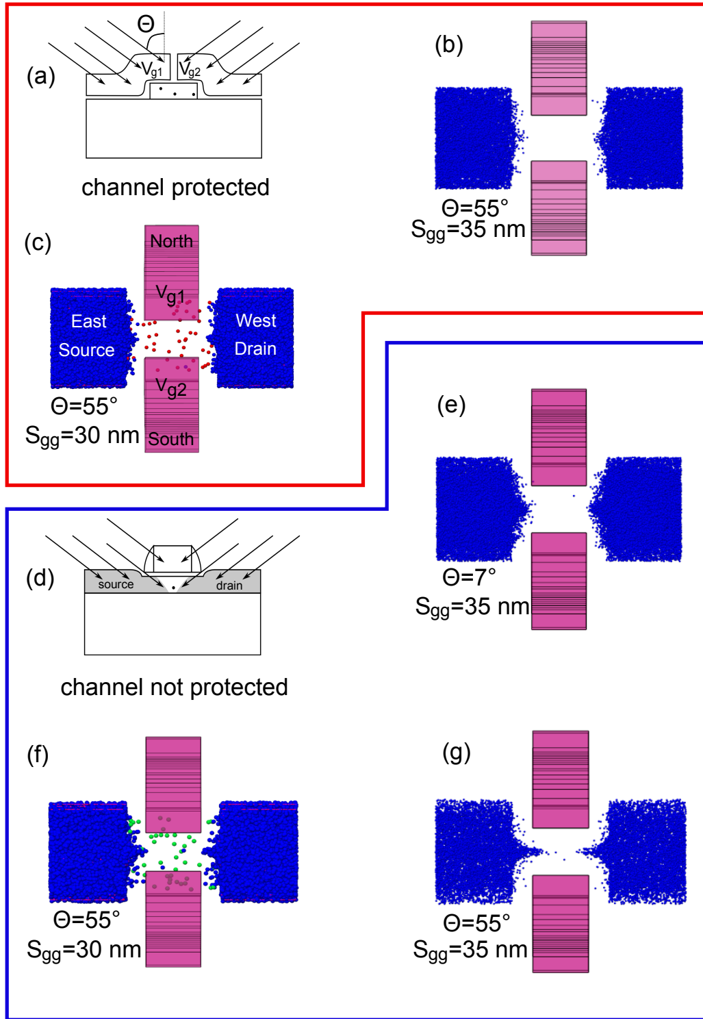
Figure 4.5 Results of KMC process simulations. Different geometries with different implantation angles \Theta , d directions. Simulations (b) and (c) correspond to a NS implantation. The gates and the spacers protect the channel in this case. For simulations (e) to (f), the implantation is done along SD: the channel is less protected, which induces a n increased implantation in the middle of the channel between the gates.
