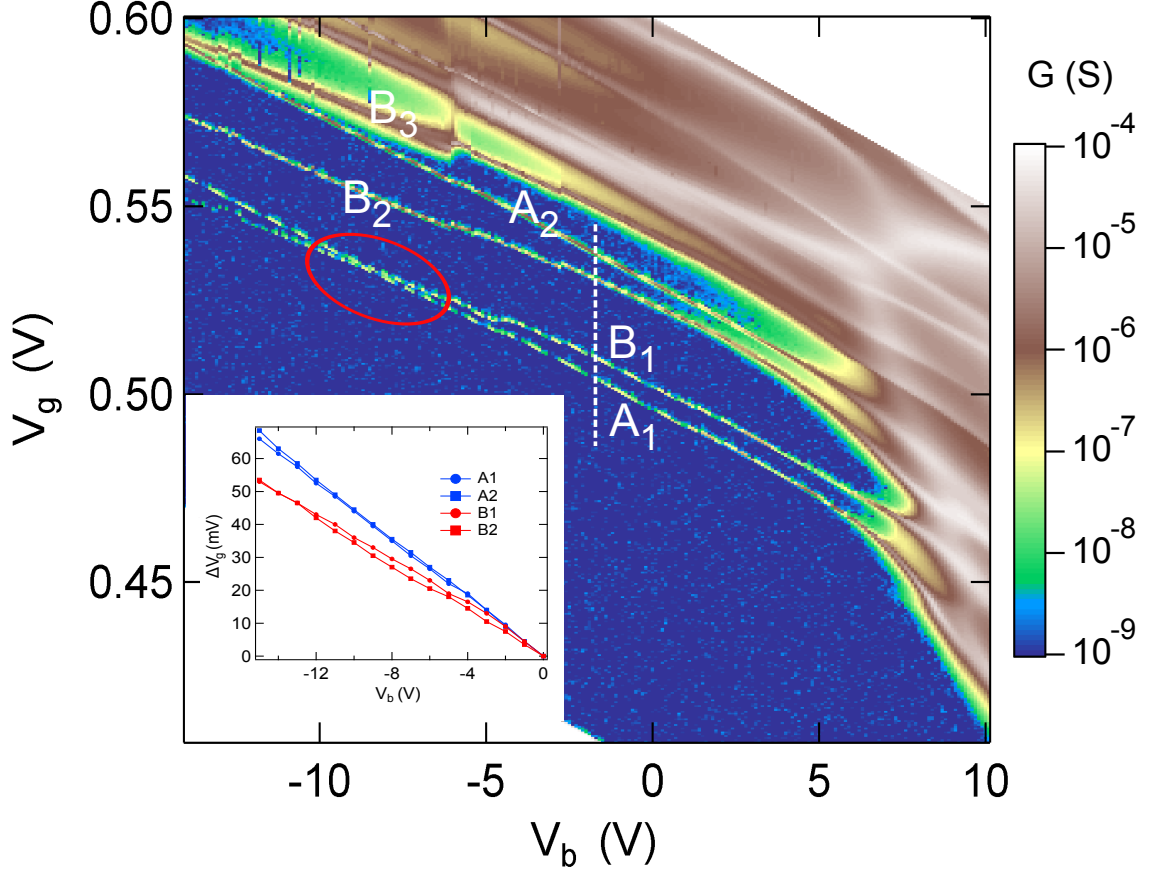
Figure 2.4 Differential conductance measured at T=100 mK with V_{ac} = 30\mu\text{V} as a function V_b and V_g . for negative V_b , one can observe two series of lines A and B which run in parallel. They are attributed to the corner states of the nanowire. Inset: position of each line relatively to their position at V_b = 0\text{V} .
