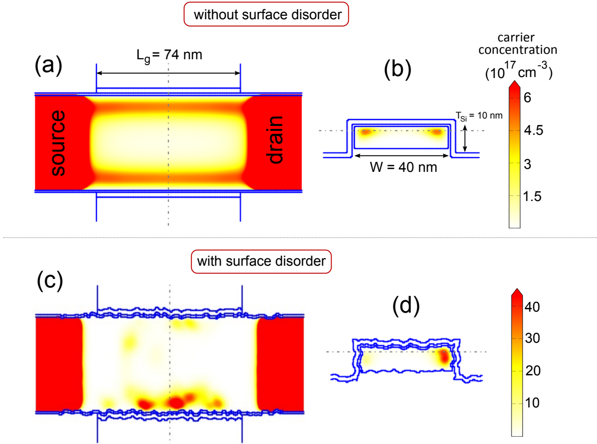
Figure 2.5 Simulations of the electron density at 77K (with V_b = -7\text{V} and a V_g corresponding to one electron) in the nanowire. (a) cut along SD, at a height given by the broken line of (b). (b) Transverse cut of SD in the middle of the channel (along broken line of (a)). One can clearly evidence a higher carrier concentration in the top corners of the nanowire. (c) and (d) Effect of realistic and calibrated surface disorder, which stochastically confines electrons in the corners. From Niquet et al., private communications.
