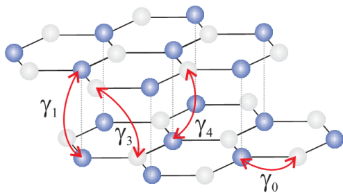
Figure 1.5: Crystal structure of the Bernal-stacked graphene bilayer with the corresponding SWM hopping parameters. From ref. [25]
