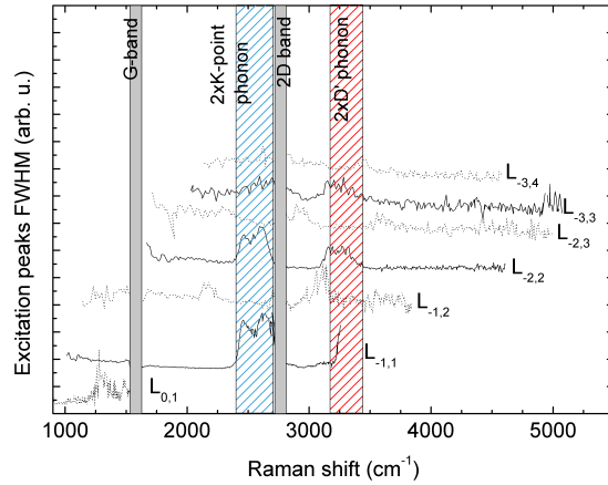
Figure 7.21: FWHM of a single Lorentzian fit to excitation peaks as a function of energy. Blue and red dashed rectangles show the range of energies when \Delta|n| = 0 transitions broaden simultaneously.
