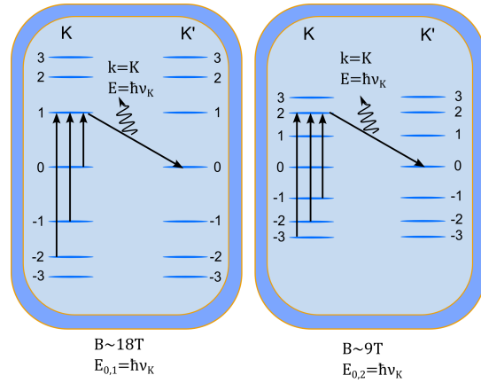
Figure 7.23: Illustration of a resonant scattering of an electron by K-point phonon
