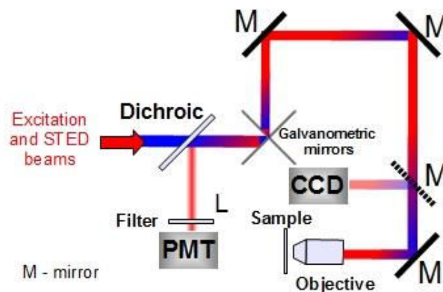
Figure 9.9: Optical layout of the SW-STED microscope
