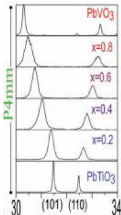
Fig. 1.21. Modification in peak position (caused by variation of lattice parameters) for the \text{PbTiO}_3 - \text{PbVO}_3 solid solution [41].
