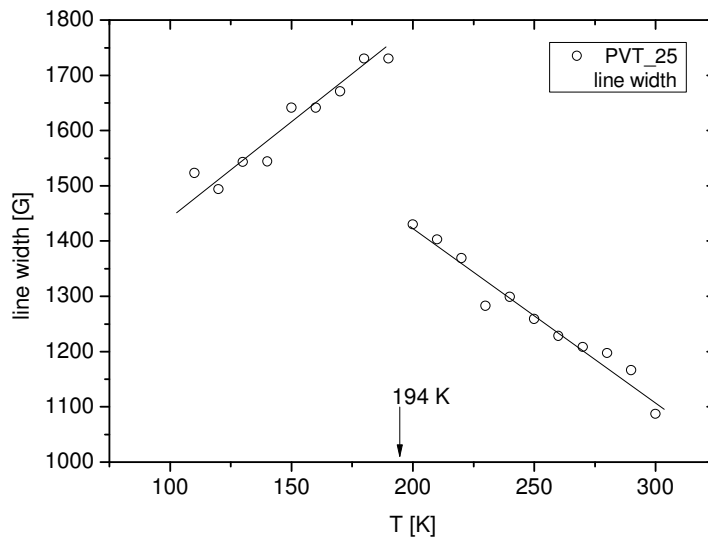
Fig. 5.40. Temperature dependence of the line width in function of temperature for PVT_25.
