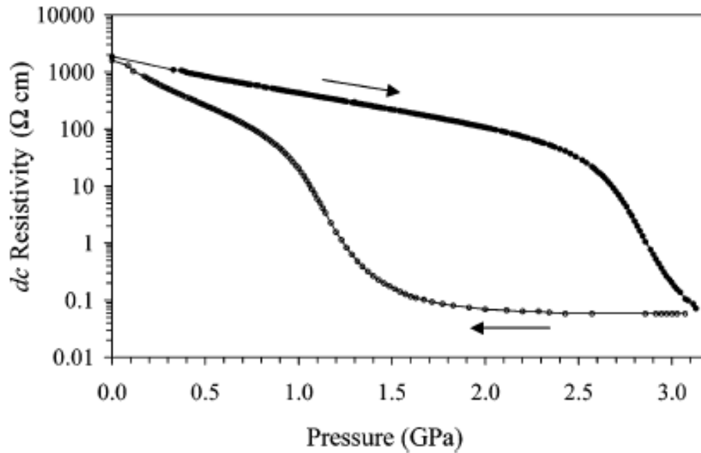
Fig. 1.23. Electric resistivity in function of pressure for PbVO_3 [33].
