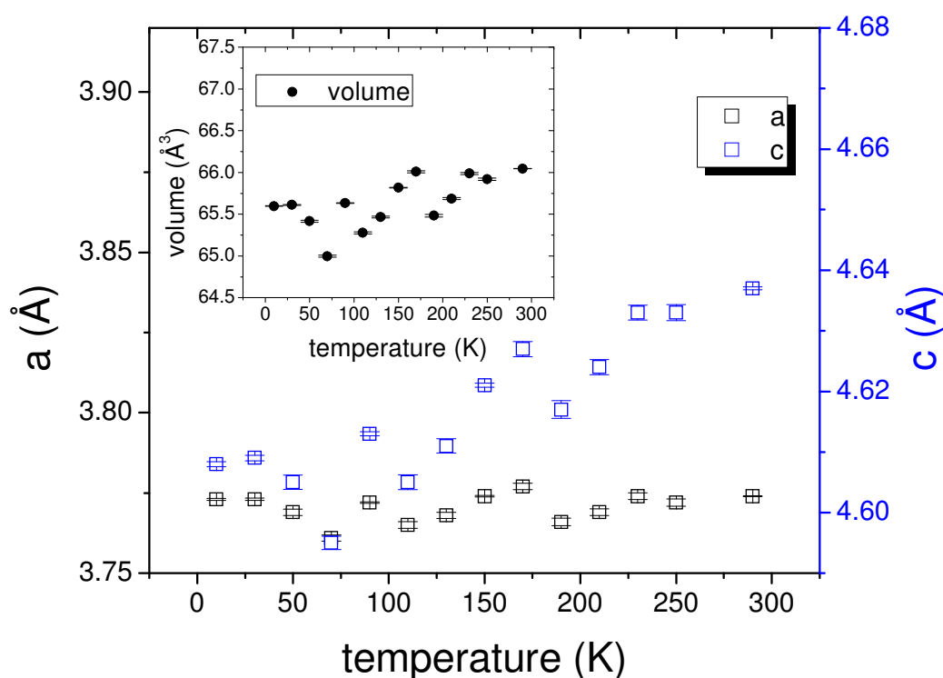
Fig. 4.5. Variation of lattice parameters with the temperature for PbVO_3 (sample labelled PVO_005). Insert shows the variation of the unit cell volume with the temperature.
