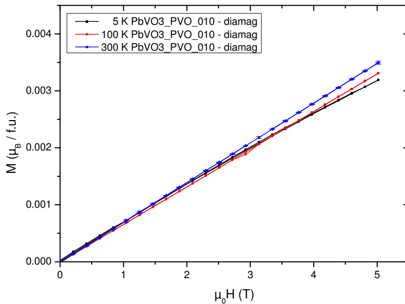
Fig. 5.5. M(H) for PbVO_3 (PVO_010) at 5 K, 100 K and 300 K.
