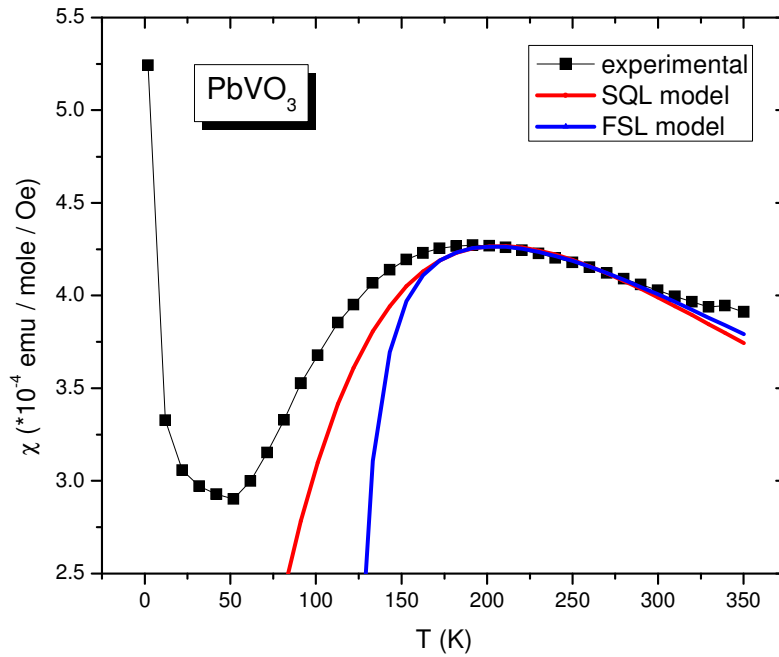
Fig. 5.4. SQL and FSL fits for the \chi(T) data of PbVO_3 . Black points are experimental data. The SQL fit is shown by the red line and FSL fit is the blue line.
