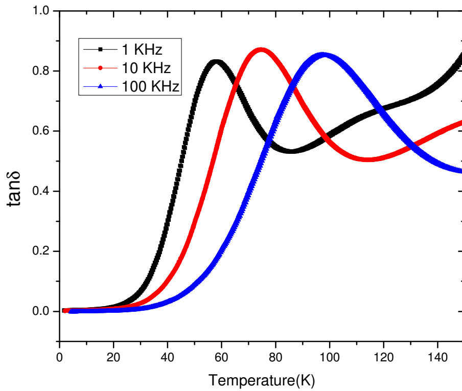
Fig. 5.64. Variation of \tan\delta in function of temperature and frequency for PbV_{0.6}Fe_{0.4}O_3 (PVF_020).
