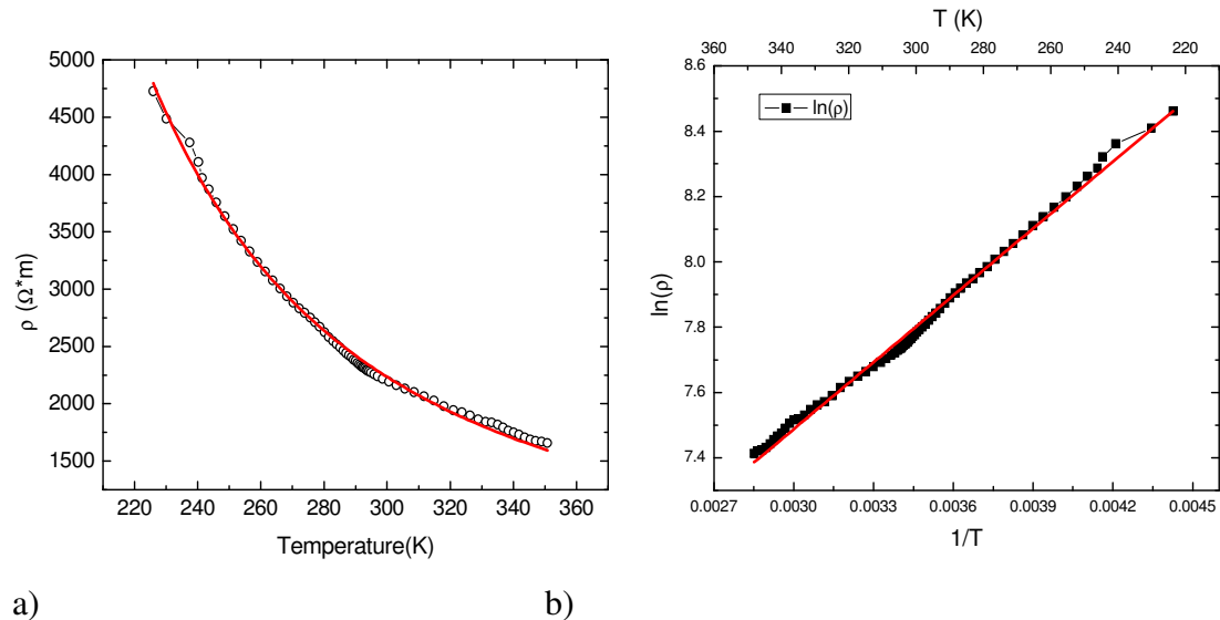
Fig. 5.59. a) \rho (T) for high temperature domain of resistivity measurement, b) \ln(R) in function of 1/T plot for PbVO_3 in the high temperature domain. Black points represent experimental data and the red line is the linear fit. The small fluctuations in the experimental data are caused by the instabilities in temperature.
