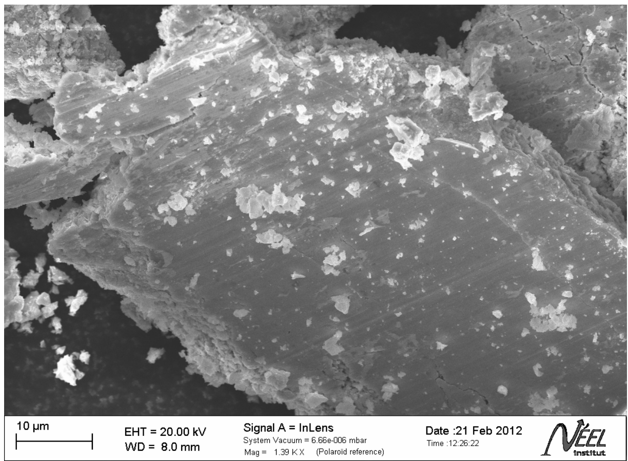
Fig. 3.20. Grains of PbVO_3 sample PVO_005. Parallel scratches can be observed on the surface of the grain.
