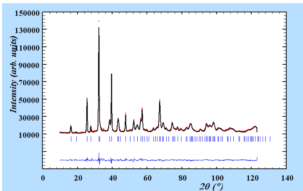
Fig. 4.38. Refinement for NPD data collected for the PVF_25 sample at the DIB. The PVF_25 sample is a mixture of different samples with the \text{PbV}_{0.75}\text{Fe}_{0.25}\text{O}_3 composition.
