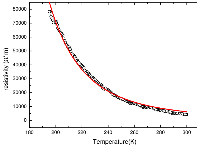
Fig. 5.57. Dependence of resistivity in function of temperature for a \text{PbVO}_3 single crystal. The hollow black dots represent the experimental data points and the red line is the exponential fit of the \rho(T) graph.
