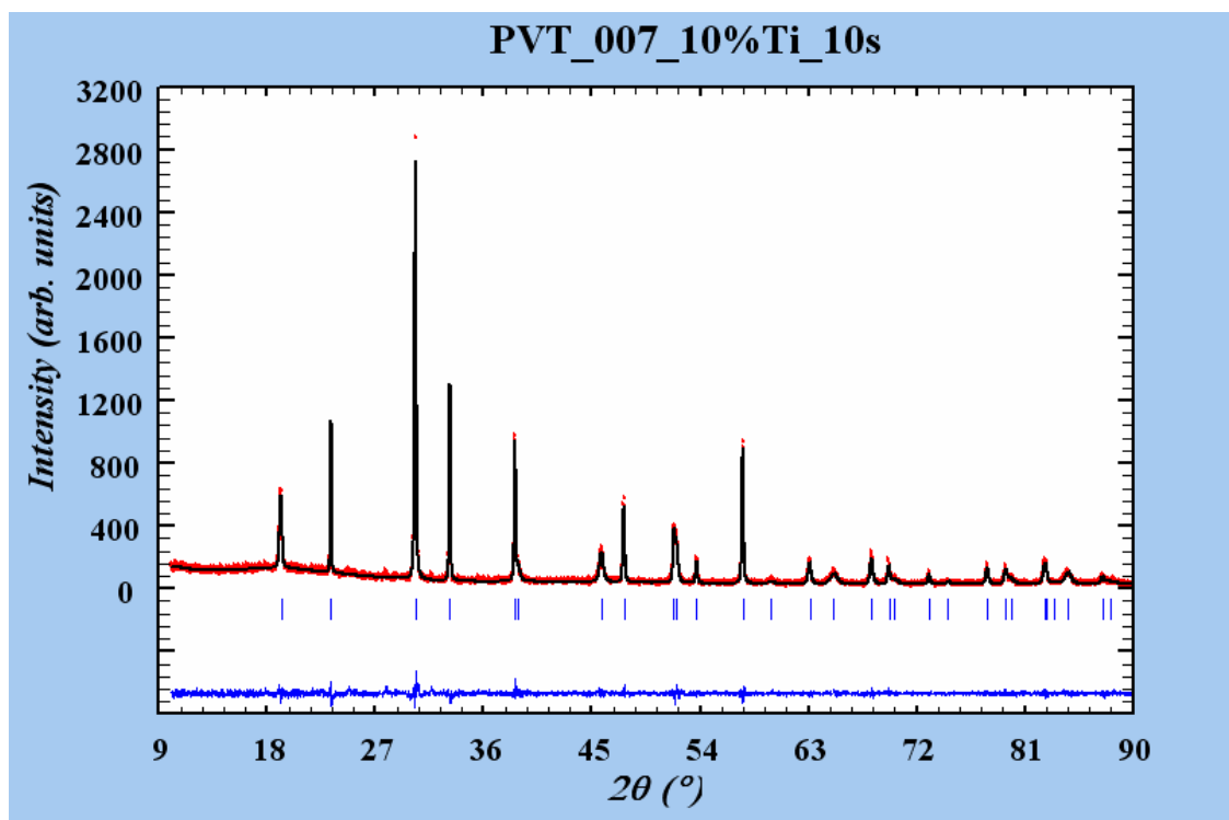
Fig. 4.13. Rietveld refinement for PbV_{0.9}Ti_{0.1}O_3 (the PVT_007 sample).
