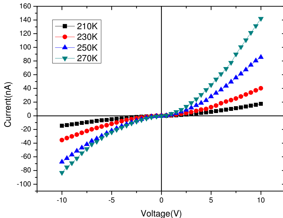
Fig. 5.61. I(V) characteristic of PbVO_3 single crystal with metal contacts.
