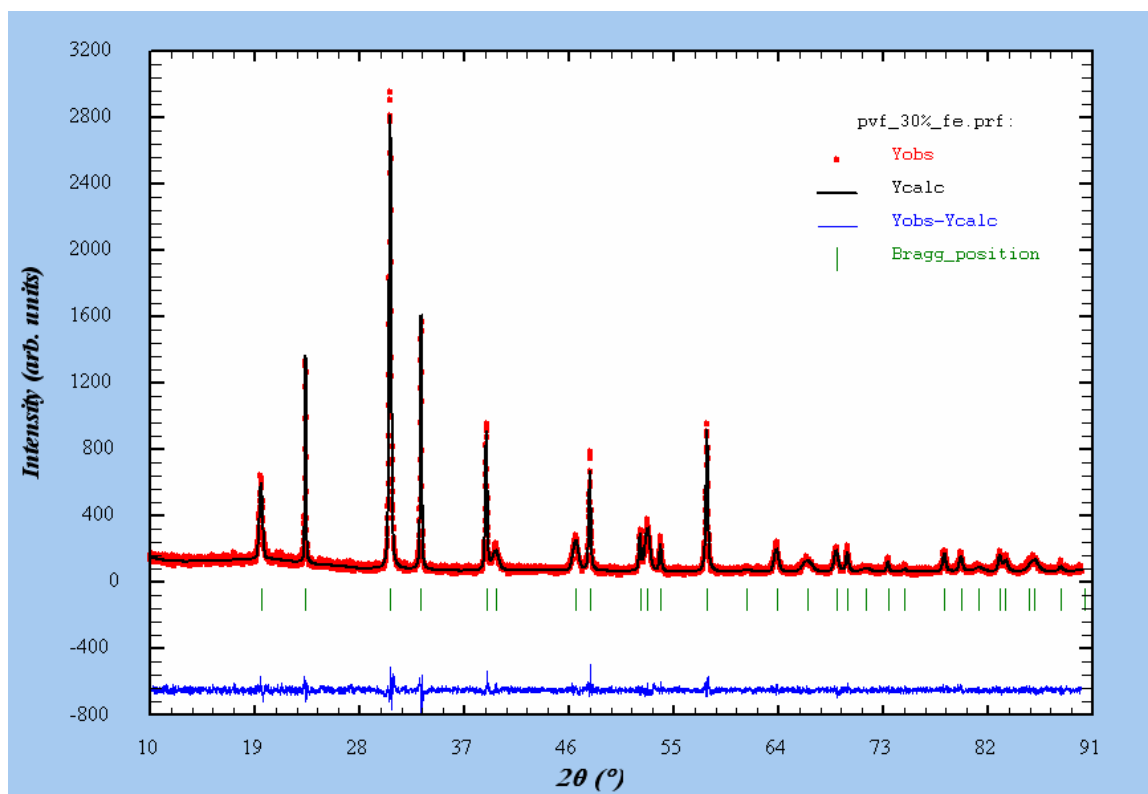
Fig 3.16. XRD and Rietveld refinement for \text{PbV}_{0.7}\text{Fe}_{0.3}\text{O}_3 (HP-HT conditions 6 GPa / 950 °C / 90 min), sample label PVF_004.
