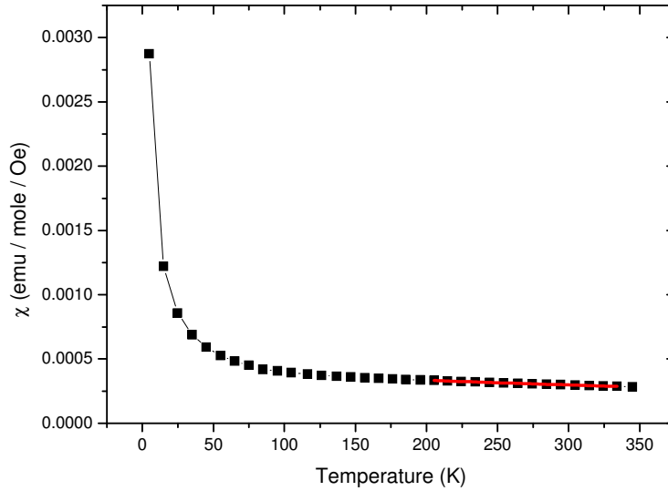
Fig 5.6. \chi(T) for PbV_{0.5}Ti_{0.5}O_3 (PVT_002). The red line represents the fit of the experimental data with a Curie-Weiss law. The fit was made without taking into account the supplementary diamagnetic contribution from the sample itself (the contribution from the film was removed before the data processing).
