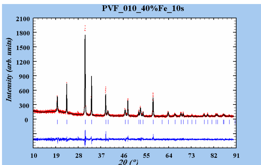
Fig. 4.29. Rietveld refinement of PbV_{0.6}Fe_{0.4}O_3 (the PVF_010 sample).
