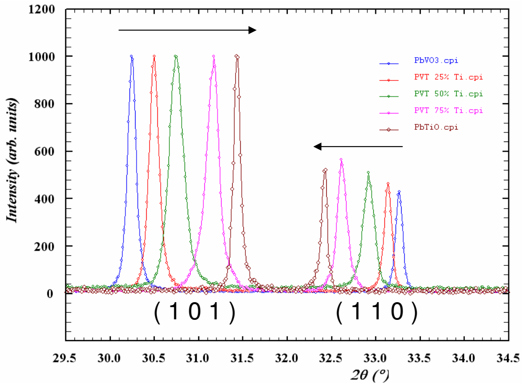
Fig. 4.9. The convergence of the diffraction peaks from PbVO_3 towards PbTiO_3 in the Pb(V_{1-x}Ti_x)O_3 compound. The arrows point in the direction in which the position of the diffraction peaks changes as the concentration of Ti is increased.
