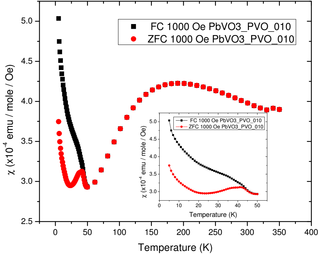
Fig. 5.3. Difference between ZFC and FC measurements for \text{PbVO}_3 . The insert is the low temperature region of the \chi(T) measurements.
