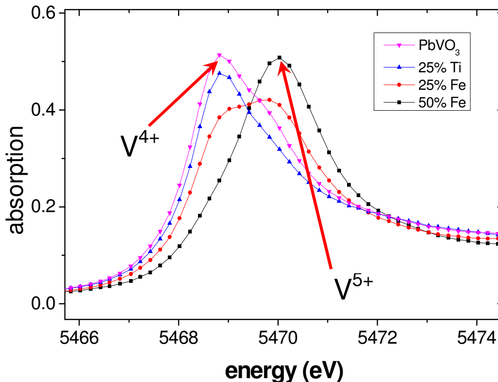
Fig. 3.25. XANES region for XAS of PbVO_3 , and substitution samples.
