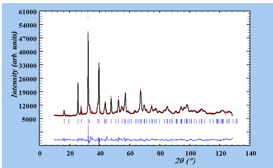
Fig. 4.40. PVF_40 (40% Fe) NPD Rietveld refinement. The PVF_40 sample is a mixture of several identical samples of the PbV_{0.6}Fe_{0.4}O_3 composition. The samples that were mixed are PVF_010, PVF_014, PVF_020 and PVF_022.
