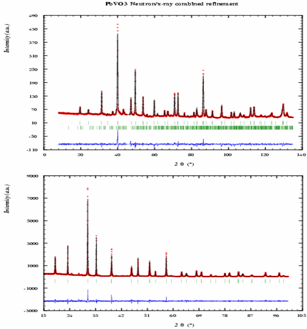
Fig. 1.16. PbVO 3 NPD (top) and XRD (bottom) refinement made by Dr. Bordet. The second row of ticks in the NPD pattern marks the reflections of Pb_3V_2O_8 [31].
