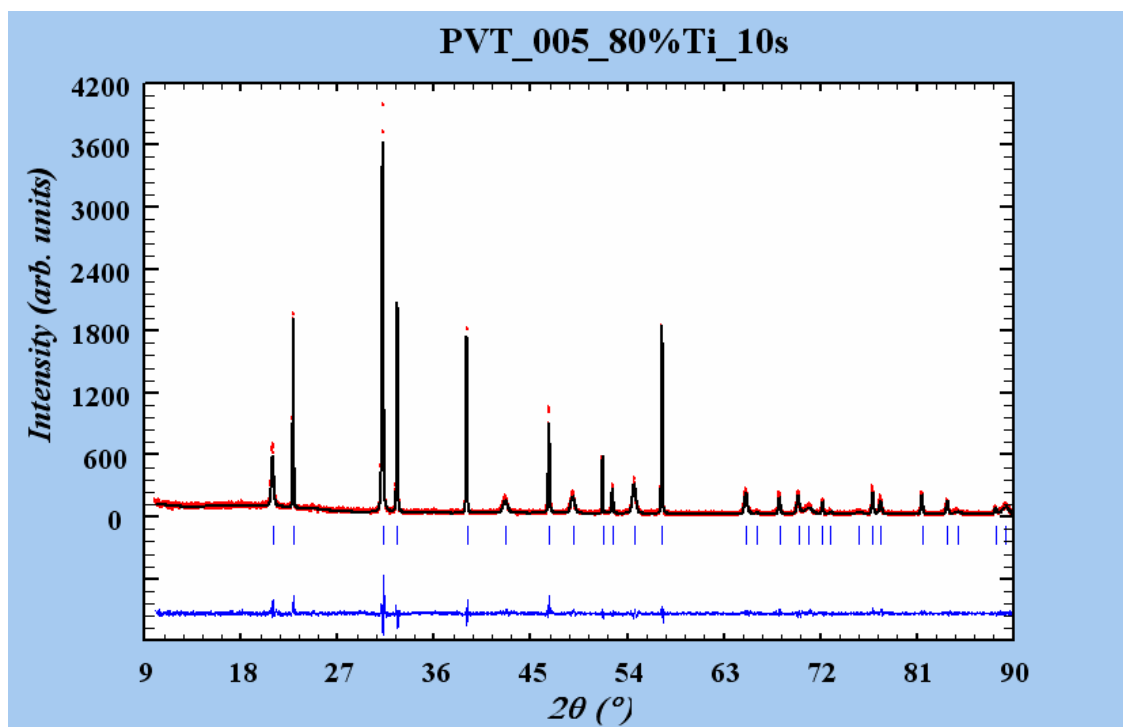
Fig 4.14. Rietveld refinement for PbV_{0.2}Ti_{0.8}O_3 (the PVT_005 sample).
