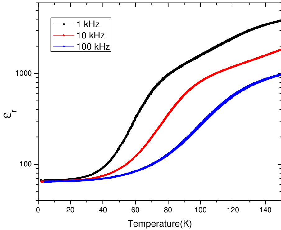
Fig. 5.63. Variation of dielectric constant with T at different frequencies for PbV_{0.6}Fe_{0.4}O_3 (PVF_020).
