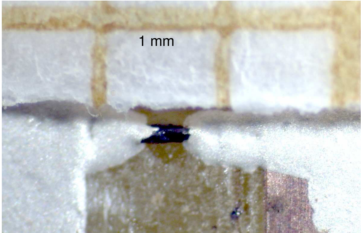
Fig. 5.56. PbVO 3 single crystal (black) with the two contacts made on each side with silver paste.
