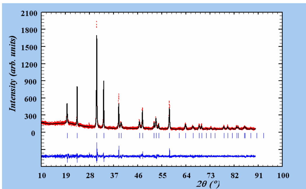
Fig. 4.39. PbV_{0.6}Fe_{0.4}O_3 (PVF_010) XRD Rietveld refinement. Standard synthesis and measurement conditions were employed.
