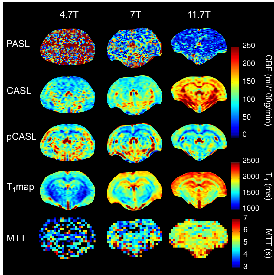
Fig. 6.5. Example of CBF, T_1 , and MTT maps obtained at three magnetic fields. Each column corresponds to a dataset collected in the same animal and during the same MRI session. The same colorbar was used to represent the CBF maps obtained with PASL, CASL, and pCASL at the three magnetic fields.
