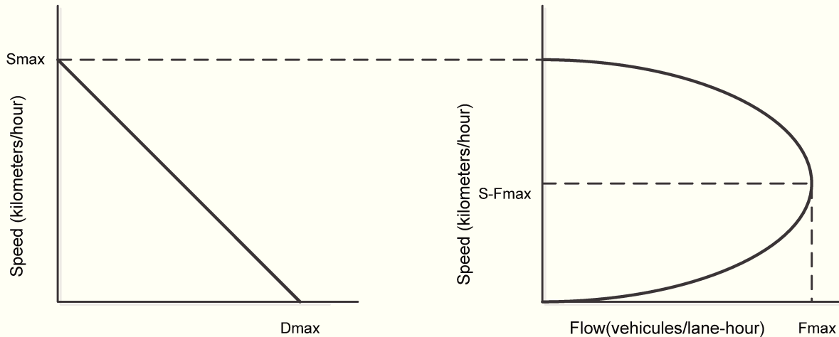
Figure 4: Derivation of the speed-flow curve. Source: Morrison (1986).
