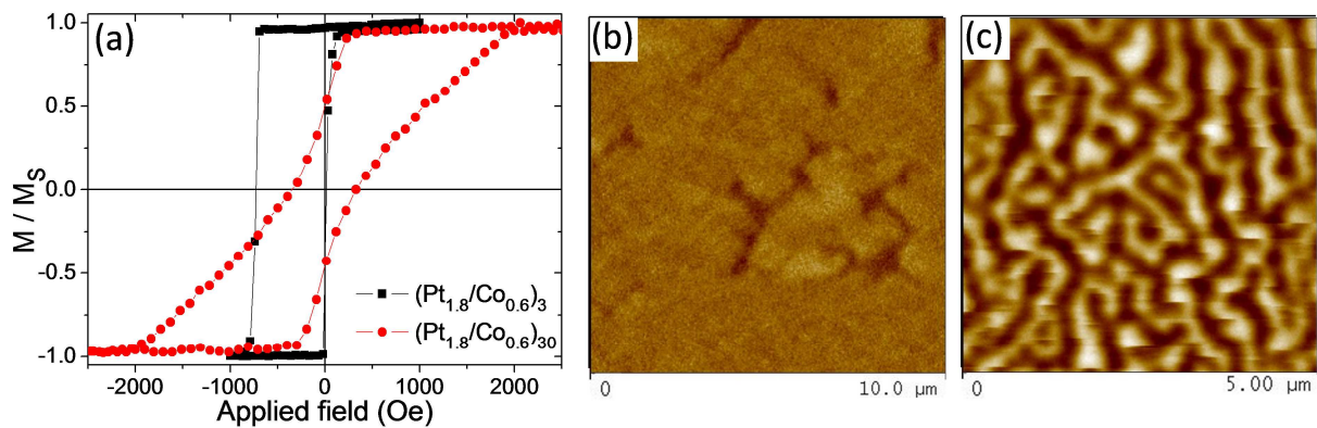
Fig. 5.1 – (a) Out-of-plane hysteresis loops for Ta 3 /(Pt 1.8 /Co 0.6 ) N /IrMn 4 /Pt 2 samples for 3 and 30 multilayer repetitions, with corresponding MFM images at remanence for N = 3 (b) and N = 30 (c).
