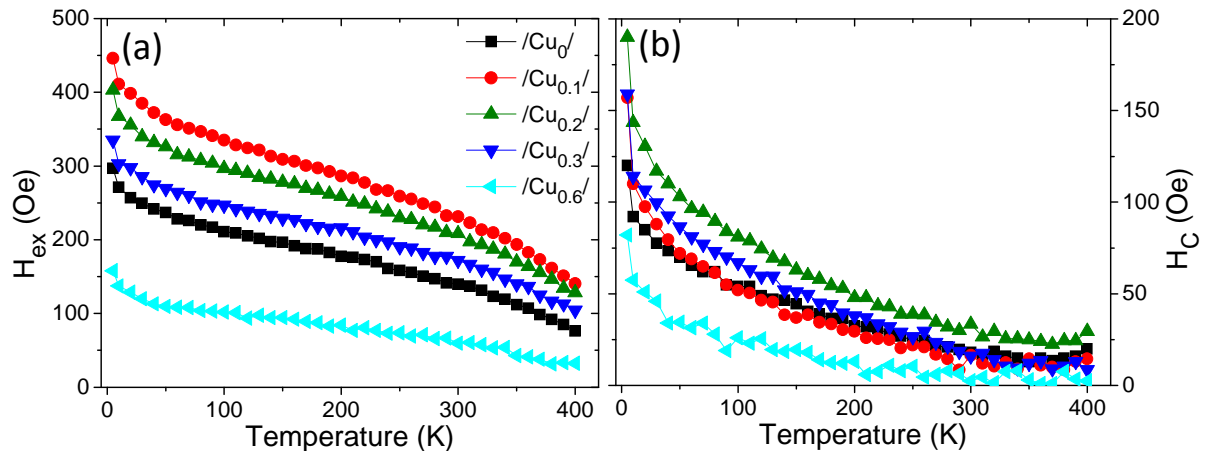
Fig. 6.7 – Exchange bias (a) and coercivity (b) evolution as a function of temperature for IrMn 12 /Cu x /Co 5 bilayers.
