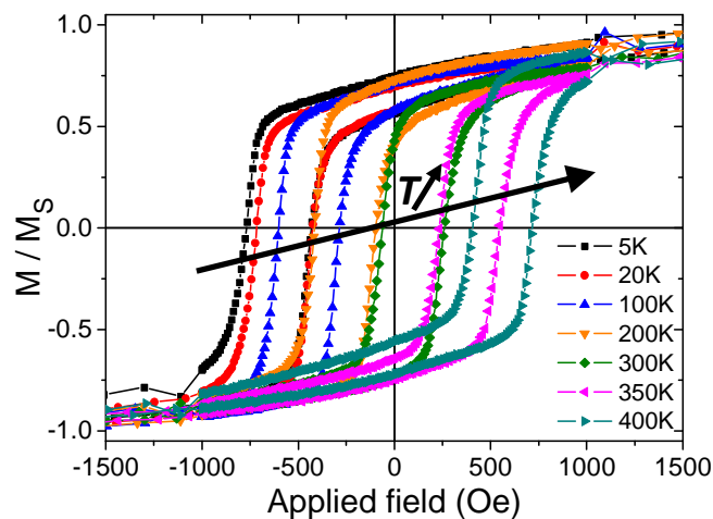
Fig. 5.12 – Hysteresis loops of the Ta_3/(Pt_{1.8}/Co_{0.6})_3/IrMn_3/Co_5/Pt_2 sample after heating at different temperatures T_a , whose values are shown in the legend. The slope is due to the paramagnetic contribution of the sample support and Si/SiO 2 substrate.
