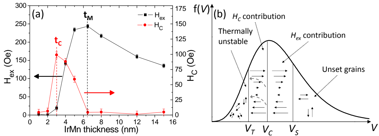
Fig. 5.2 – (a) Exchange bias and coercivity for Ta_3/Cu_2/IrMn_x/Co_5/Pt_2 . Vertical dashed lines indicate the critical thickness t_C in red and the maximum thickness t_M in black. (b) Schematic representation of the AF grain distribution in a polycrystalline system.
