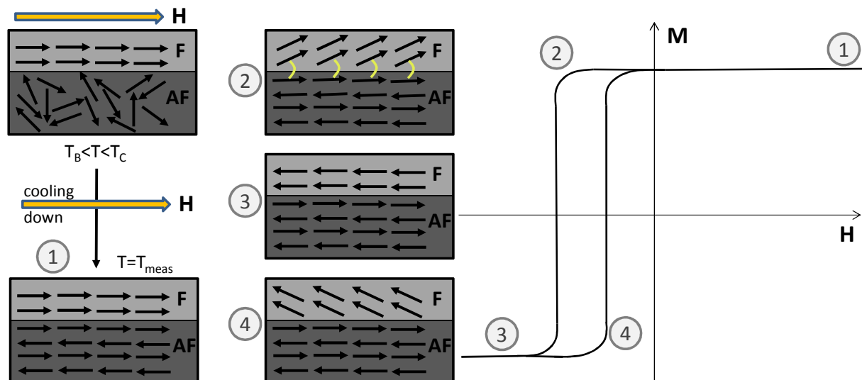
Fig. 1.5 – Schematic of exchange bias coupling.
