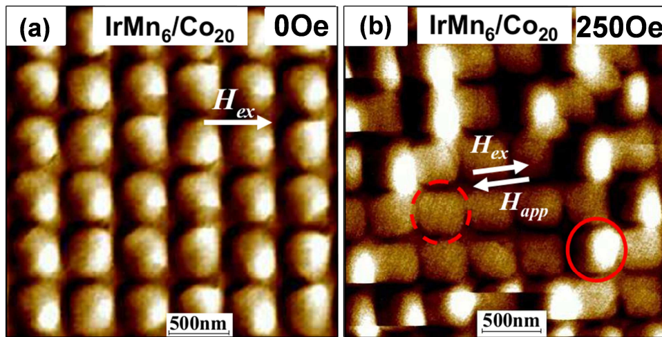
Fig. 4.5 –MFM image at remanence after field saturation (a) and with in-situ applied field (b) for 200 nm square dots of IrMn 6 /Co 20 . The transition from single domain (continuous circle) to multidomain state (dashed circle) is observed in (b)
