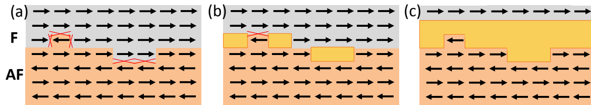
Fig. 6.14 – (a) Example of a F/AF bilayer with rough interface. The red crosses mark the magnetic frustrations due to bumps, steps and holes. (b) The same rough F/AF interface with non-continuous nF interlayer, which removes partially the frustrations. (c) F/AF interface with continuous nF interlayer. The resulting total coupling is reduced compared to case (a).
