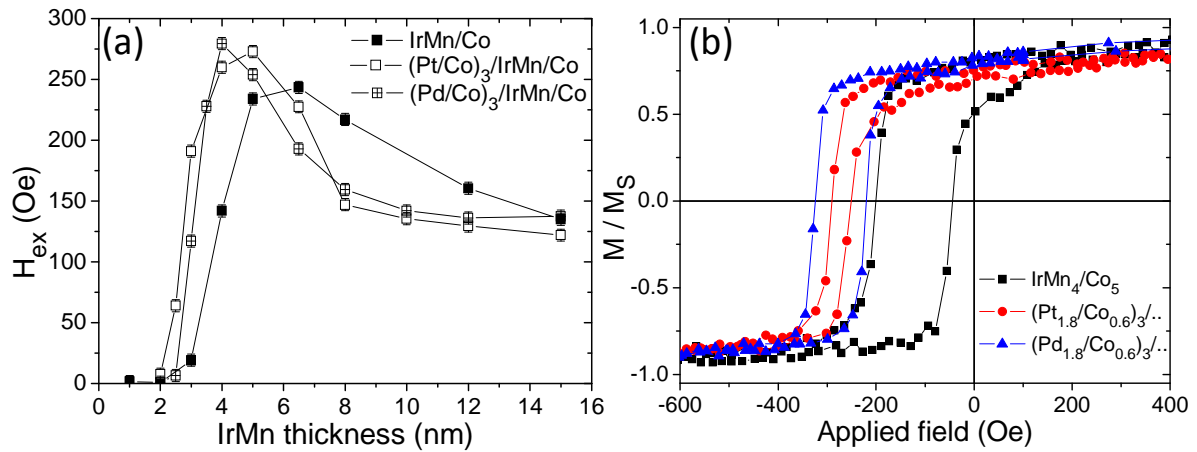
Fig. 5.4 – (a) Comparison of H_{ex} curves as a function of IrMn thickness for the three structures. (b) Hysteresis loops at 300 K for the three structures for 4 nm IrMn thickness.
