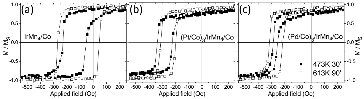
Fig. 5.20 – Hysteresis loops at 300 K for the IrMn 4 /Co (a), (Pt/Co) 3 /IrMn 4 /Co (b) and (Pd/Co) 3 /IrMn 4 /Co (c) structures for 4 nm IrMn thickness in the two annealing process cases.
