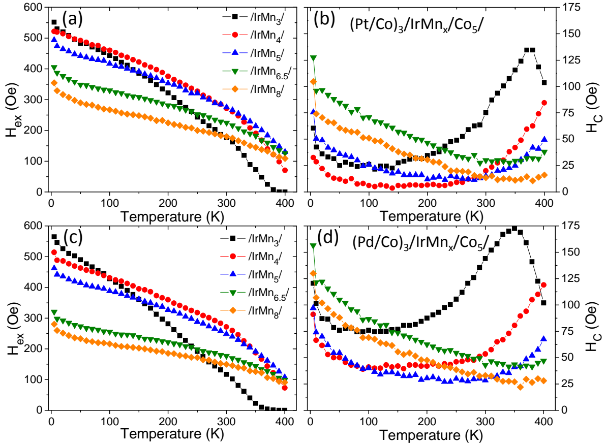
Fig. 5.9 – Temperature dependence of exchange bias H_{ex} (a,c) and coercive field H_C (b,d) for the Ta_3/(Pt_{1.8}/Co_{0.6})_3/IrMn_x/Co_5/Pt_2 (a,b) and Ta_3/(Pd_{1.8}/Co_{0.6})_3/IrMn_x/Co_5/Pt_2 (c,d) structures, for x going from 3 to 8 nm.
