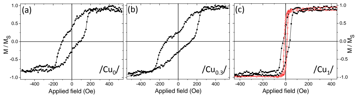
Fig. 6.4 – Hysteresis loops of as deposited samples for no interlayer (a), 0.3 nm (b) and 1 nm (c) Cu interlayer. In (c) the M(H) loop of a sample without IrMn layer is shown in open red circles.
