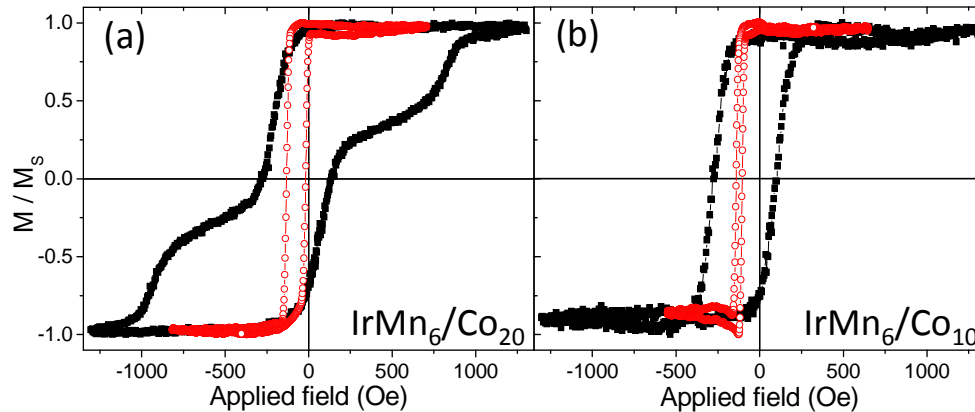
Fig. 4.7 – Hysteresis loops averaged over 50 measurements on different zones for 200 nm square dots (solid squares) and full sheet samples (open circles) for IrMn 6 /Co 20 and IrMn 6 /Co 10 samples.
