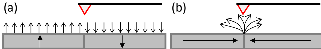
Fig. 3.6 – Interaction between the MFM tip and the perpendicular (a) or planar (b) stray field.
