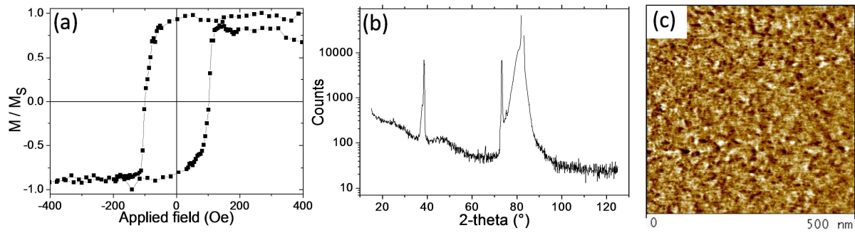
Fig. 4.24 – Hysteresis loop (a), \theta - 2\theta XRD scan (b) and AFM measurement (c) of the \text{Ta}_3/\text{IrMn}_{12}/\text{Co}_5/\text{Pt}_2 .
