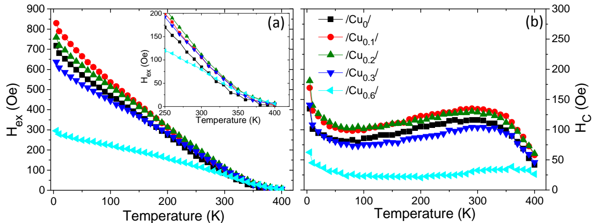
Fig. 6.8 – Exchange bias (a) and coercivity (b) evolution as a function of temperature for IrMn 4 /Cu x /Co 5 bilayers. In (a) the inset shows the H_{ex} evolution close to T_B .
