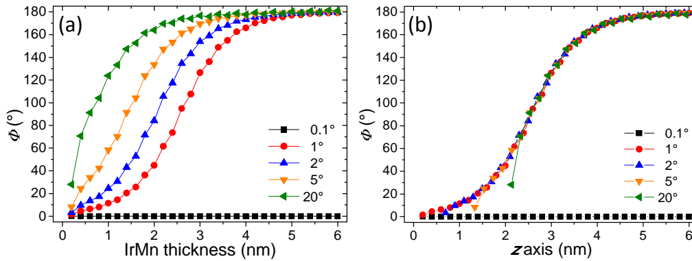
Fig. 4.33 – (a) Orientation \Phi of the AF spins along the AF thickness for different angles \varphi of the anisotropy axis (same K_{AF} ). (b) Translation of the origins along the z axis to prove the superposition of the domain wall profiles.
