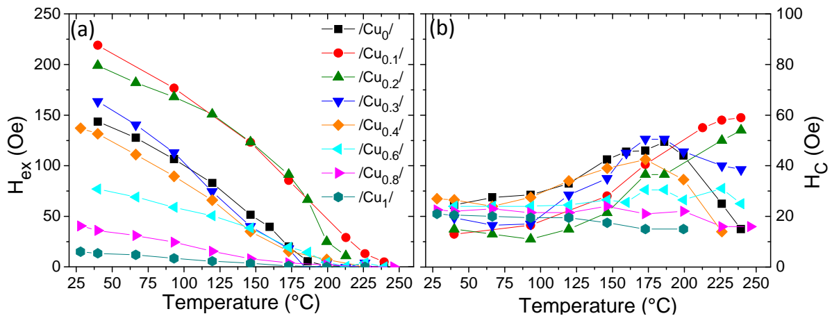
Fig. 6.6 – Exchange bias (a) and coercivity (b) evolution as a function of temperature for IrMn_{12}/Cu_x/Co_5 bilayers at high temperature.
