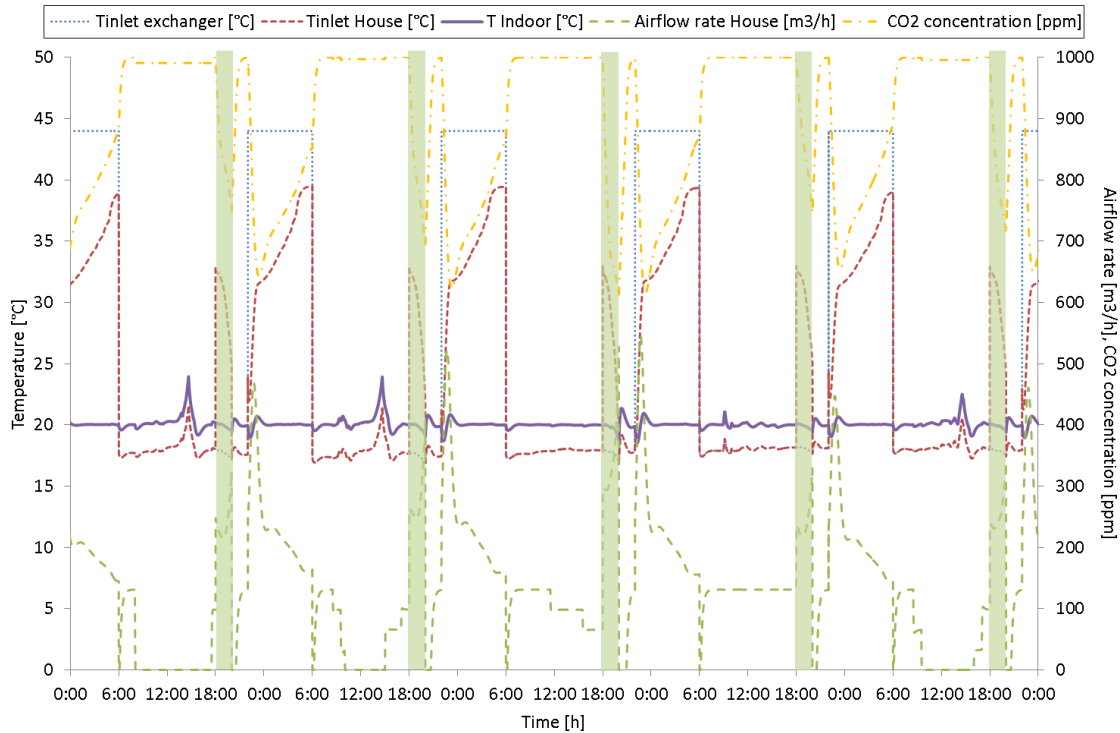
Figure 5.35: Performance of the heat exchanger, days 3-8, case 38, inlet exchanger air temperature=44°C, initial insulation, occupancy scenario, second optimization approach
