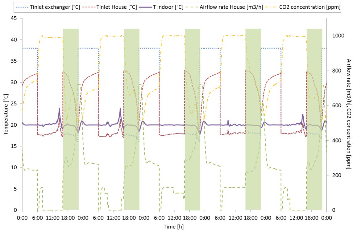
Figure 5.22: Performance of the heat exchanger, days 3-8, configuration 3, inlet exchanger air temperature=38°C, occupancy scenario, first optimization approach
