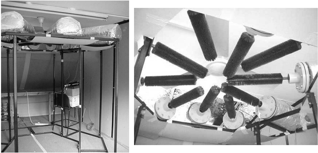
Figure 2.27: Turnpenny et al. LHS unit, overall view (left) and heat exchange pipes (right)
