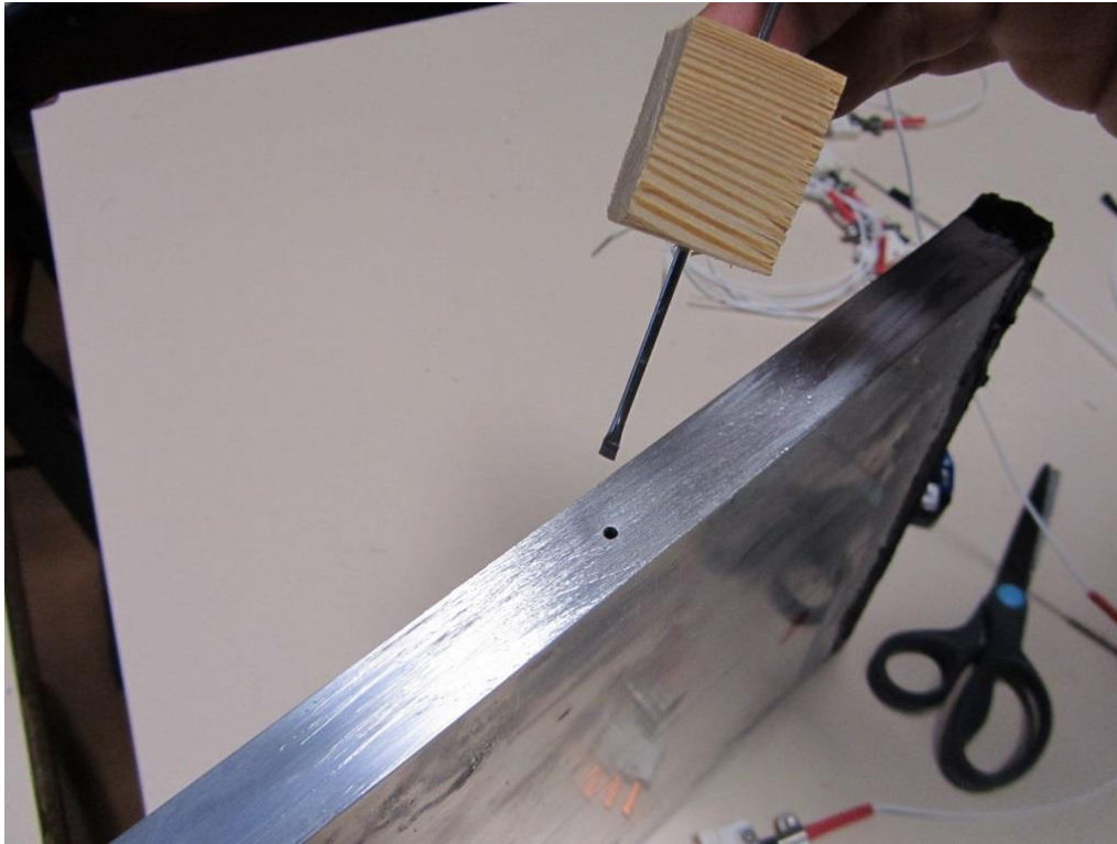
Figure 3.11: Insertion of temperature sensors inside the PCM
