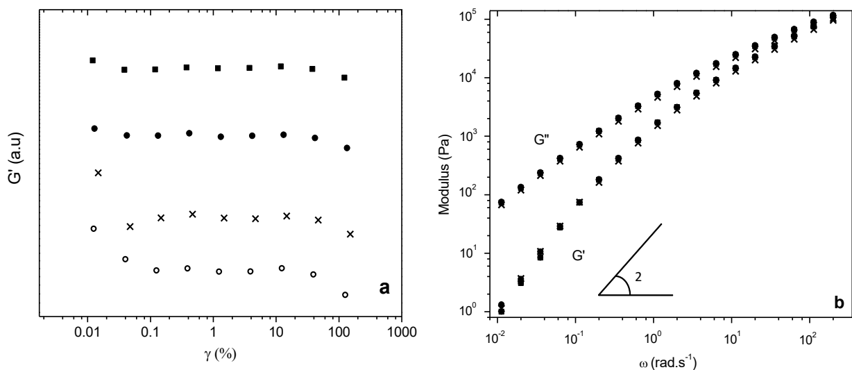
Figure 8. (a) Strain sweep tests and (b) frequency sweep measurements in linear conditions at 150°C for (○)PBAT, (x) PBATC 22 , (●) PBATC 39 and (■) PBATC 50 .
