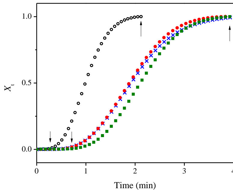
Figure 6. Non-isothermal crystallization data using a cooling rate of -10^\circ\text{C}\cdot\text{min}^{-1} for (o)PBAT, (x) PBATC 22 , (●) PBATC 39 and (■)PBATC 50 .
