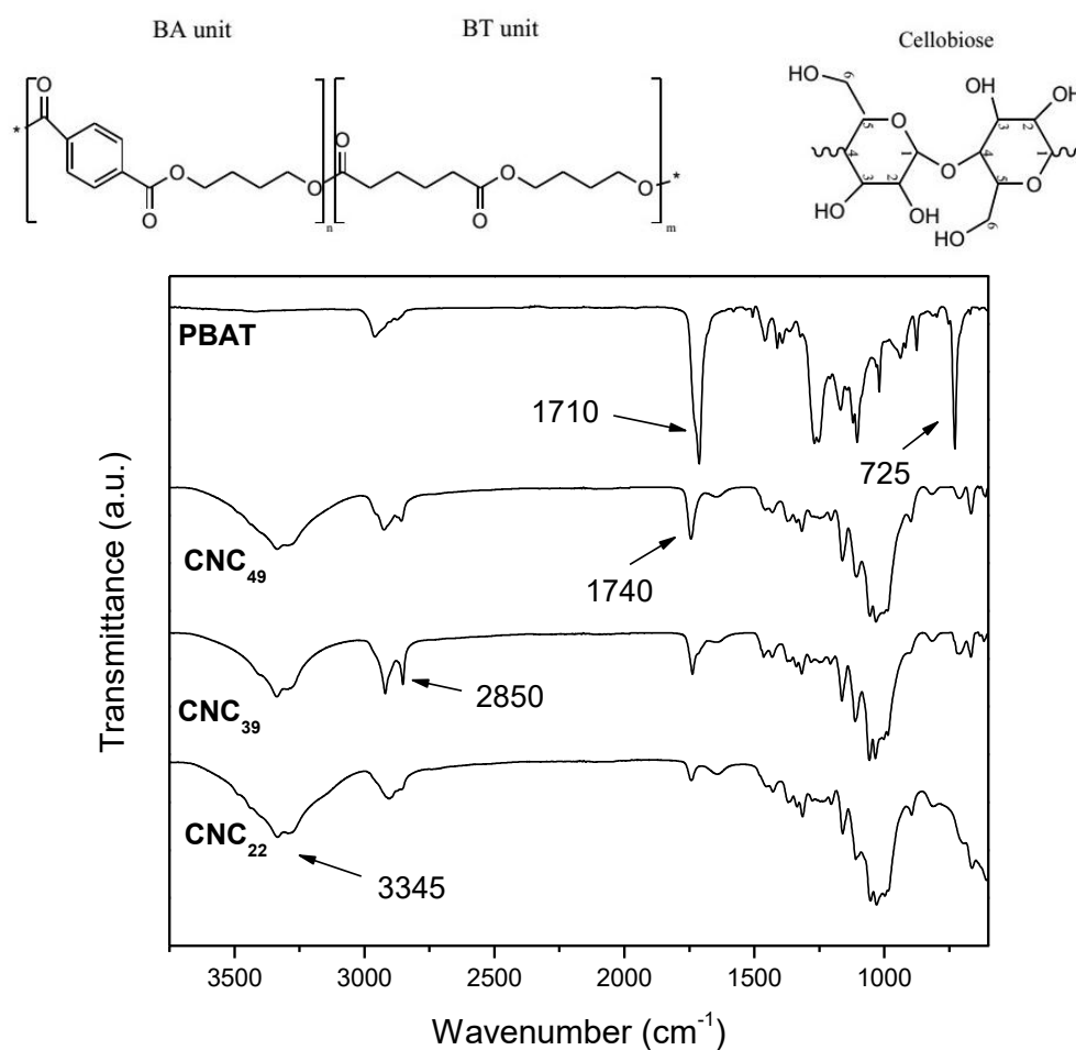
Figure 3. Chemical structure of PBAT and cellulose monomer units, and FTIR spectra for PBAT and the three sets of CNC.
