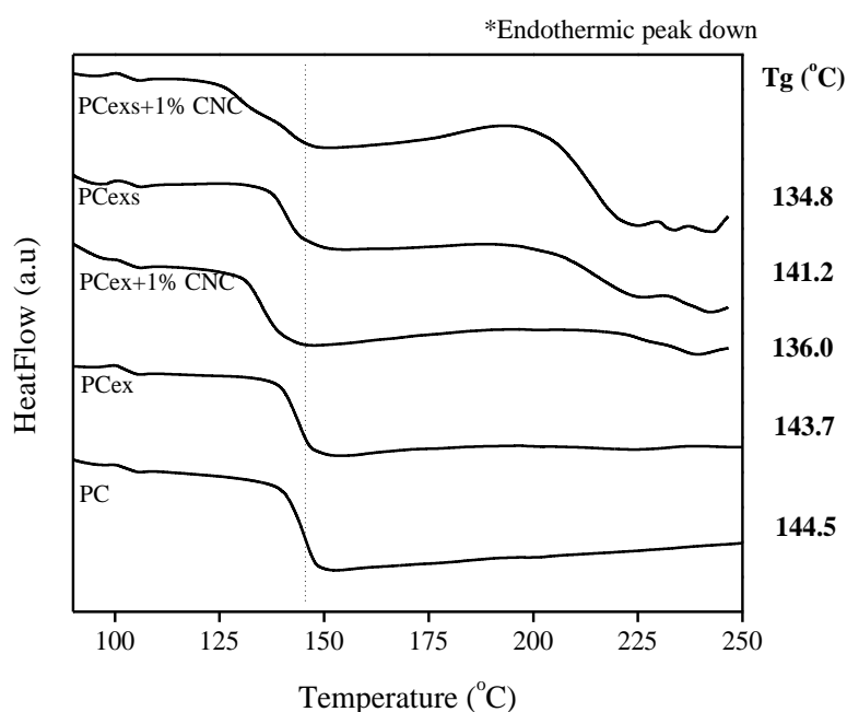
Figure 9. DSC thermograms for neat PC and nanocomposites reinforced with 1 wt% CNC.
