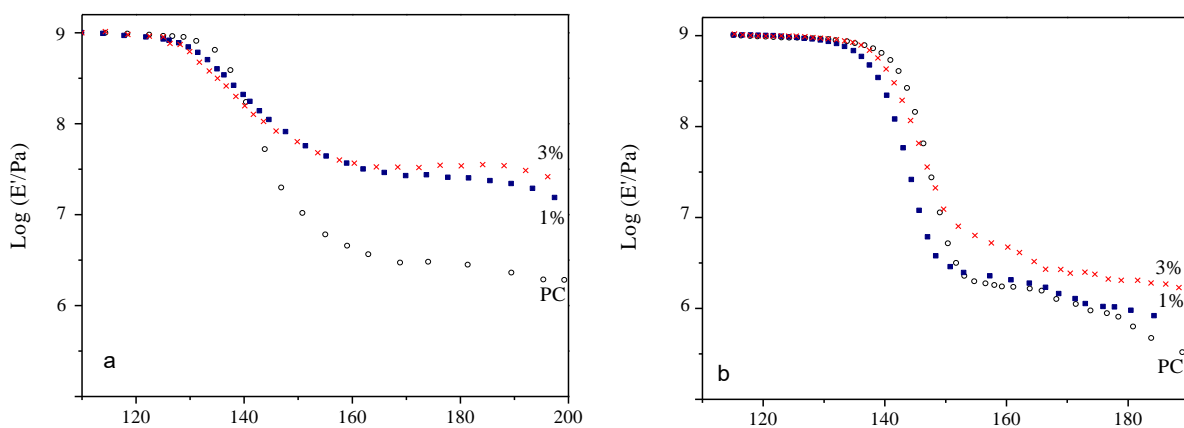
Figure 12. Evolution of the logarithm of the storage modulus as a function of temperature at 1 Hz for (a) PCexs and (b) PCex materials: neat matrix ( \circ ), and nanocomposites filled with 1 wt% ( \blacksquare ) and 3 wt% ( \times ) CNC.
