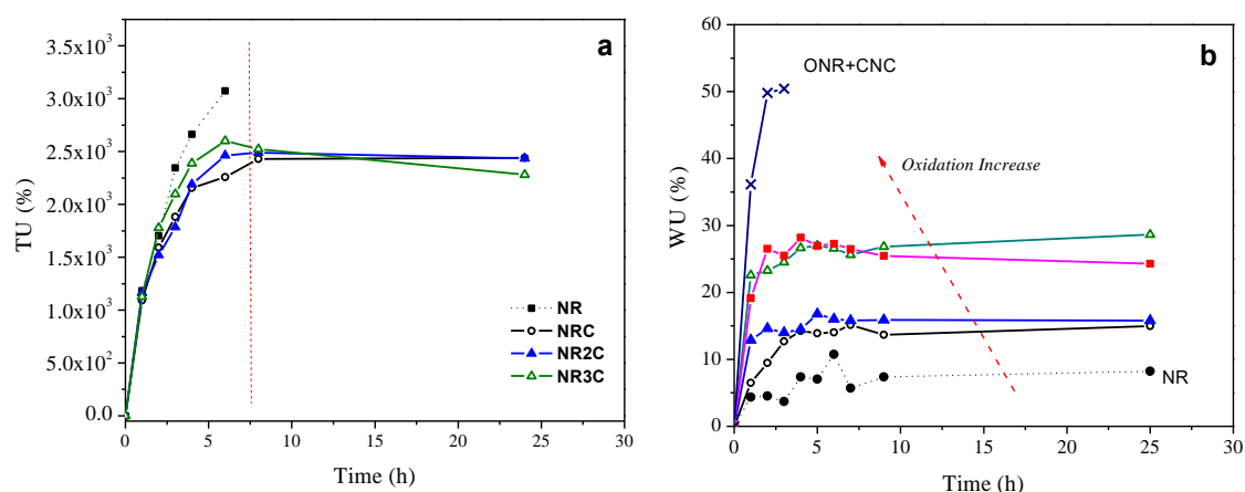
Figure 7. Evolution of (a) the toluene uptake (TU) and (b) the water uptake (WU) as a function of time at room temperature for NR (●), NRC (○), ONR2C (▲), ONR3C (△), ONR4 (■), and ONR5C (×). The solid lines serve to guide the eyes.
