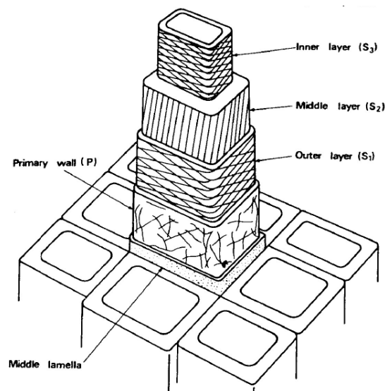
Figure 11. Illustration of the cell wall structure.
