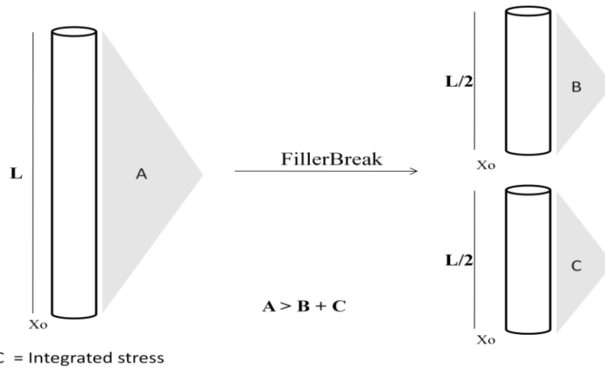
Figure 4. Representation of the stress distribution around the fiber after fracture.
