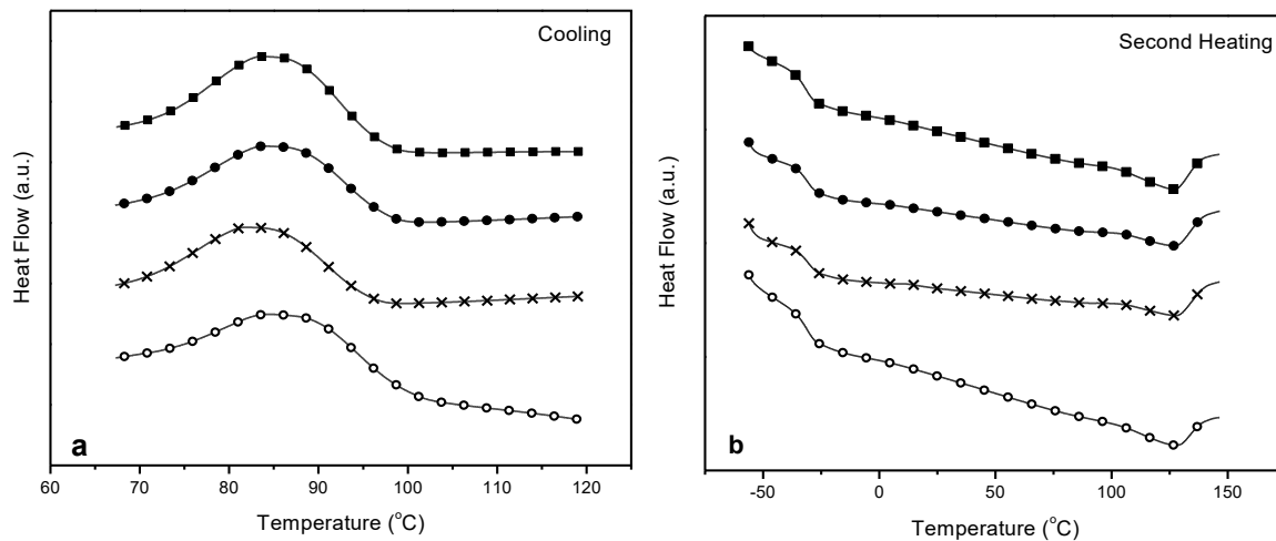
Figure 5. DSC curves recorded during (a) cooling and (b) second heating scan for PBAT and the three sets of CNC reinforced composites: (o)PBAT, (x) PBATC 22 , (●) PBATC 39 and (■) PBATC 50 .
