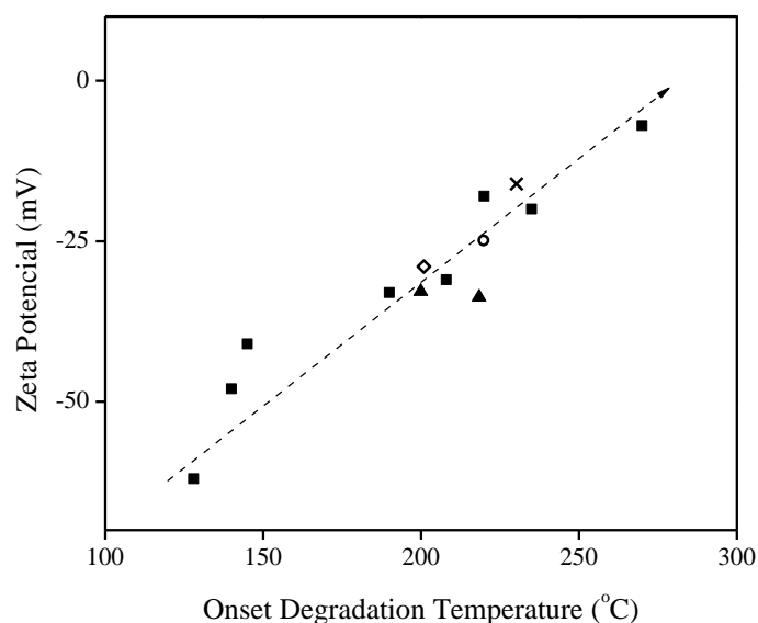
Figure 22. Relationship between degradation temperature and zeta potential for CNC produced by (x) microbial hydrolysis, (o) ammonium persulfate, (▲) TEMPO, (◇) phosphoric acid and (■) sulfuric acid.
