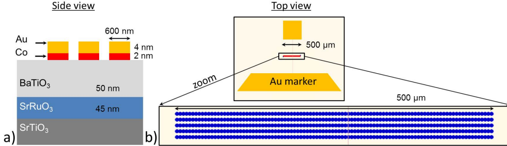
FIGURE 5.1 – Schematic of a) the side view and b) the top view of the sample.
