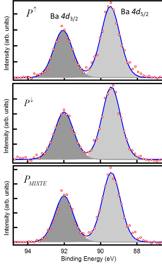
FIGURE 5.11 – Peak fitting of the Ba 4d core-level spectra extracted for the three electrode switched in three different state of polarization P^\uparrow (top) P^\downarrow (middle) and P^{\uparrow\downarrow} (bottom).
