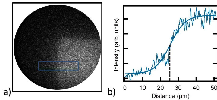
FIGURE 5.6 – a) Image of the Au marker (FoV= 115 \mu\text{m} ) using Au 4f core level. b) Intensity profile as a function of the distance in \mu\text{m} extracted along the blue rectangle in a), fitted with a sigmoid. The position of the edge of the gold pattern is marked by the black dash line.
