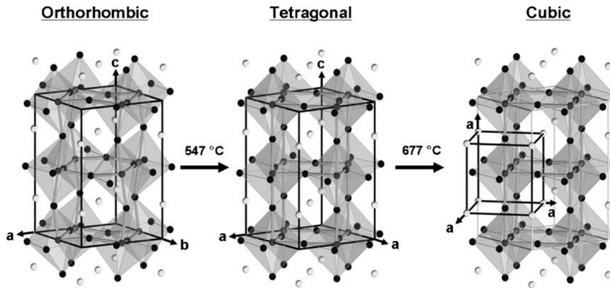
FIGURE 1.10 – A sequence of phase transitions of unstrained bulk SRO from orthorhombic to tetragonal and then cubic symmetry at 547^{\circ}\text{C} and 677^{\circ}\text{C} , respectively. The unit cell of the orthorhombic SRO consists of four formula units of the ideal cubic perovskite structure. The atoms of Ru occupy high-symmetry positions with respect to the orthorhombic shape of the cell. The atoms of O and Sr are displaced from their high-symmetry positions due to the octahedral tilting. The tetragonal SRO is a one-tilt system, where \text{RuO}_6 octahedra are rotated only about the [001] direction. The cube corresponds to the unit cell of each SRO form. Gray, black, and white balls represent Ru, O, and Sr atoms, respectively. From Choi et al. [49].
