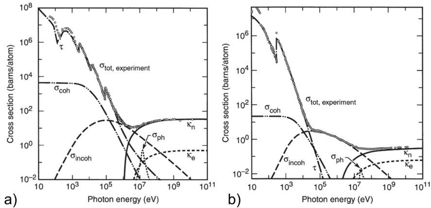
FIGURE 2.11 – Total photon cross section in a) lead and b) carbon, as a function of photon energy, showing the contribution of different processes: \tau atomic photo-effect; \tau_{coh} coherent scattering; \tau_{incoh} incoherent scattering; K_n pair production (nuclear field); K_e pair production (electron field); \tau_{ph} photonuclear absorption. (From Ref. [127]).
