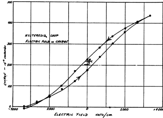
FIGURE 1.1 – First Polarization - Electric Field loop measured by J. Valasek on Rochelle Salt in 1920 [4].
