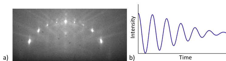
FIGURE 2.30 – a) RHEED pattern obtained from electron diffraction from a clean TiO 2 (110) surface. The bright spots indicate the diffraction peaks. b) Model of the fluctuation of the intensity of a single RHEED point during deposition. Each peak represents the forming of a new monolayer. The degree of order is at a maximum once a new monolayer has been formed. The spots in the diffraction pattern therefore have maximum intensity since the maximum number of diffraction centers of the new layer contribute to the diffracted beam.
