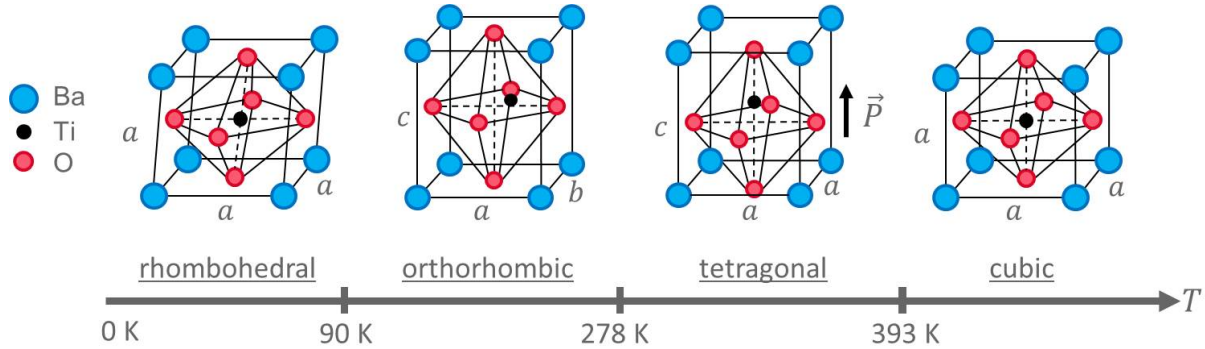
FIGURE 1.3 – BaTiO_3 perovskite structure in the rhombohedral, orthorhombic, tetragonal, and cubic phase depending on the temperature T .
