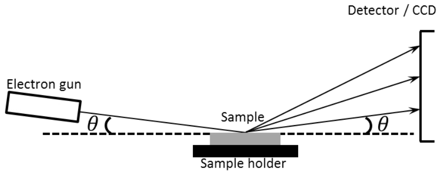
FIGURE 2.29 – Systematic set up of the electron gun, sample and detector/CCD components of a RHEED system. Electrons follow the path indicated by the arrow and approach the sample at angle \theta .
