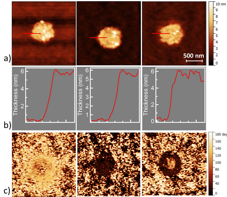
FIGURE 5.2 – a) AFM, b) height profile (along the red line of figure a)), and c) PFM phase images for 3 pads on the Au/Co/BTO/SRO heterostructure of the pad in the P^{\downarrow} state (left), the pad in the P^{\uparrow} state (middle) and the pad in the P^{\uparrow\downarrow} state (right).
