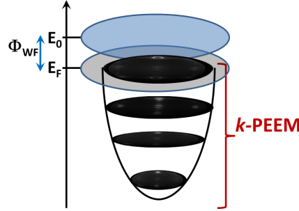
FIGURE 2.24 – Schematic of the I = f(KE, k_x, k_y) stack obtained using the k -PEEM mode. Images presented are from a STO(001) sample.
