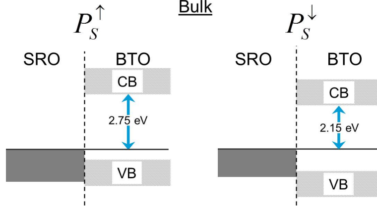
FIGURE 3.22 – Schottky barrier height for electrons deduced from the experimental HAXPES results for the P_S^\uparrow and P_S^\downarrow polarization states at saturation, assuming a band gap of 3.20 eV. The SBH is calculated using the bulk peak component of the Ba 4d.
