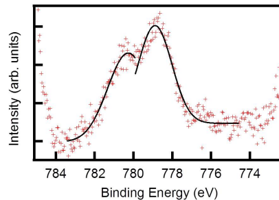
FIGURE 4.12 – Snapshot of the Ba 3d_{5/2} core level acquired during the time-resolved experiment (red crosses) and Gaussian fit (black line).
