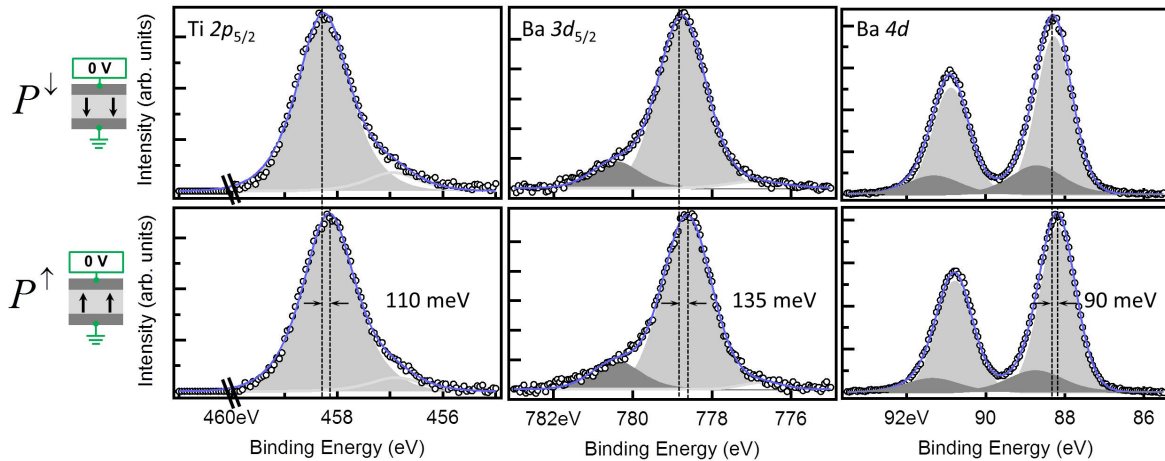
FIGURE 4.6 – Ti 2p_{5/2} , Ba 3d_{5/2} and Ba 4d core level spectra in the P^\downarrow (top) and P^\uparrow (bottom) states in remanence (black empty dots). The peaks used for the peak fitting (filled in dark or light shades of grey) and the corresponding fit (blue line) are superimposed on the spectra.
