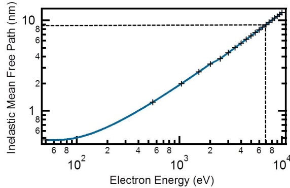
FIGURE 3.9 – IMFP (nm) for the Ba 4d core level in BTO calculated for energies between 50 eV and 10 keV.
