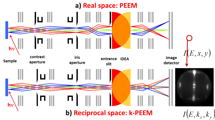
FIGURE 2.23 – Schematic of the electron beam pattern for the real (PEEM) and reciprocal space (k-PEEM).
