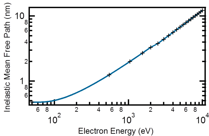
FIGURE 2.16 – IMFP for the Ba 4d core level in BTO for energies going from 50 eV to 10 keV.
