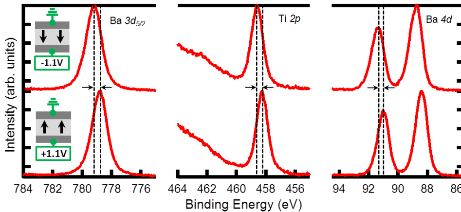
FIGURE 3.19 – Ba 3d_{5/2} , Ti 2p_{3/2} and Ba 4d core level spectra acquired in saturation for both P^\uparrow (bottom) and P^\downarrow (top). Vertical dotted lines indicate the shift in intensity maximum.
