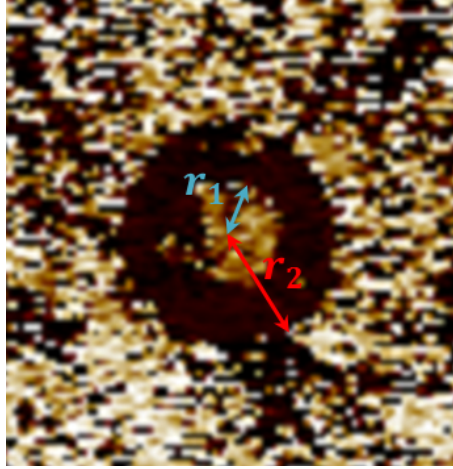
FIGURE 5.13 – PFM image of the electrode B switched in the P^{\uparrow\downarrow} polarization state. The blue arrow indicates r_1 the radius of the inner circle in the P^\downarrow state and the red arrow indicates the radius r_2 of the total pad.
