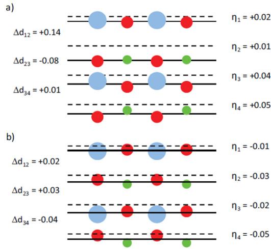
FIGURE 1.15 – Relaxation and rumpling for the first four atomic layers in a) P^+ and b) P^- domains obtained from the Ba 4d XPD. The original and relaxed atomic layer positions are indicated by dotted and solid lines, respectively. The atomic displacements are multiplied by 10 for clarity. Ba atoms are represented in blue, oxygen in red and titanium in green. From Ref [89].
