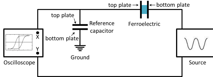
FIGURE 2.2 – Schematic circuit for a Sawyer - Tower measurement.
