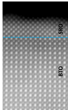
FIGURE 2.28 – High Resolution TEM section of the top SRO/BTO interface of a studied sample, grown by PLD.
