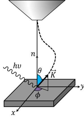
FIGURE 2.22 – Geometry of the emission and collection of photoelectrons. The surface of the sample (in grey) is illuminated with a beam of photons of energy h\nu and electrons are emitted, with an energy KE , a wave vector \vec{K} and emission angles \theta and \varphi . The photoelectrons particular trajectory (dashed line) is due to the high potential difference between the extractor lens and the sample.
