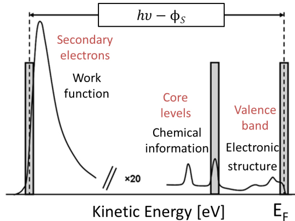
FIGURE 2.12 – Typical photoemission spectrum, showing the measured intensity as a function of the kinetic energy for three types of electrons: secondary electrons, electrons coming from core-levels and the valence band.
