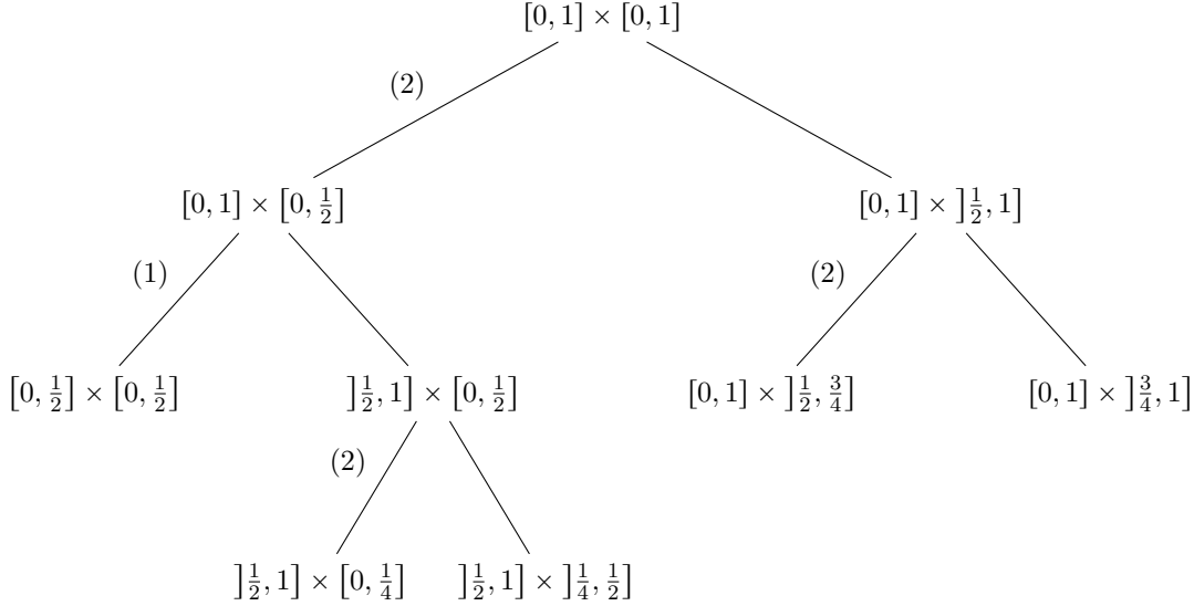
Figure 3: Binary tree labeled with the sequence of cutting directions (2, 1, 2, 2) corresponding with the dyadic partition represented on the right side of Figure 2.
