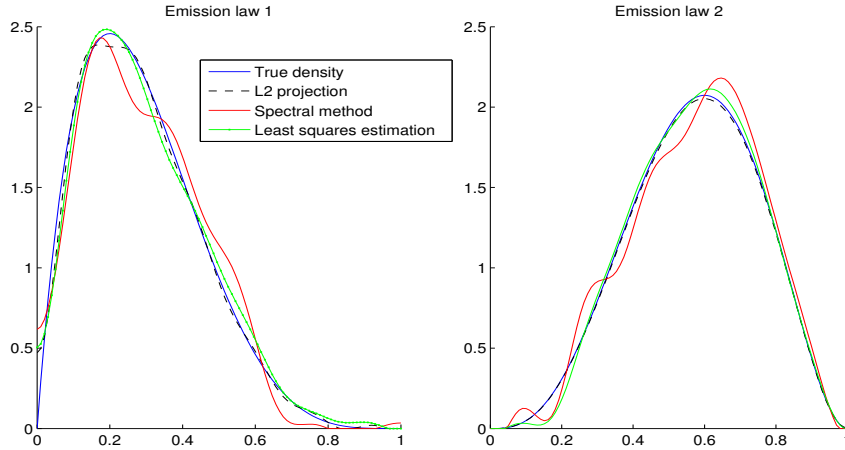
Figure 20: Estimators of the emissions densities using the Fourier basis
