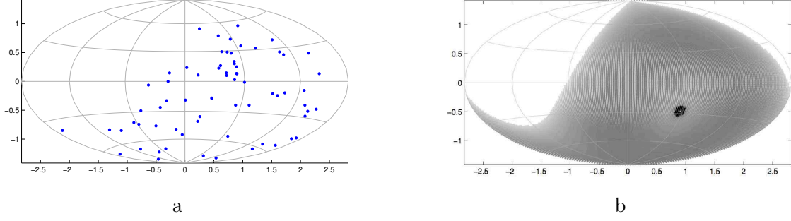
Figure 17: a/ Representation of the 69 arrival directions of highest energy cosmic rays (Pierre Auger data) b/ Coverage function g_0 for the Pierre Auger observatory (the darker the more observed, white area non-observed)
