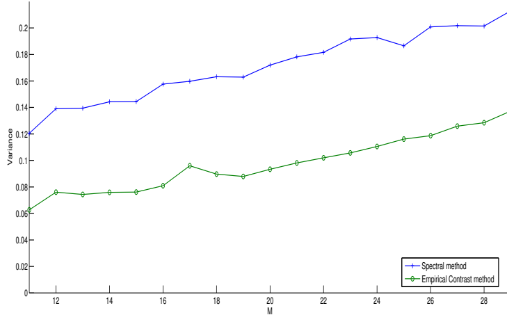
Figure 18: Comparison of the variances of the spectral and the least squares estimators.
