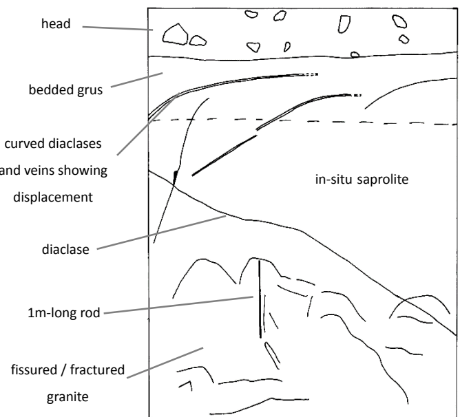
Figure 3-11. Section 2 - close-up view of the middle of the quarry face.
