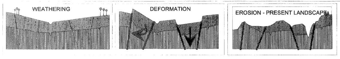
Figure C-4. Formation of the present-day landscape from the infra-Cretaceous planation surface (from Lachassagne et al. 2001b).
