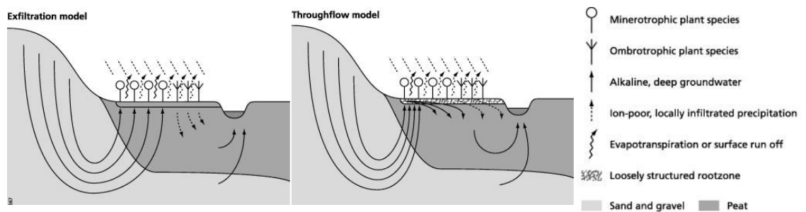
Figure 1-13. Exfiltration and throughflow models tested by van Loon et al. (2009).
