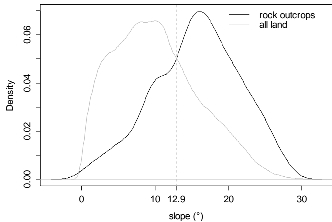
Figure 3-27. Kernel density estimation of slope distribution at mapped rock outcrops vs. in the entire area.
