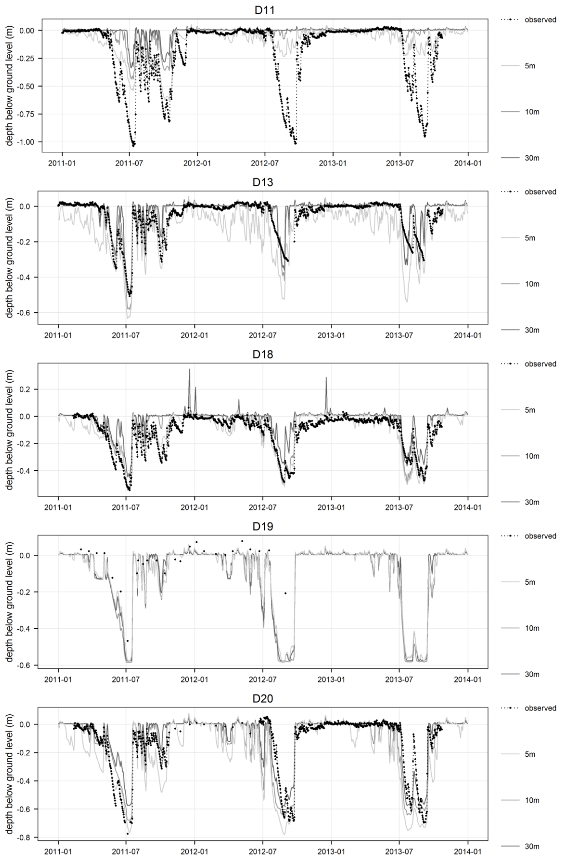
Figure 6-14 (continued). Effect of model resolution on simulated groundwater table depth.
