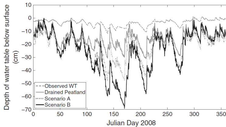
Figure 1-11. Impact of afforestation (including drainage) on simulated groundwater table depth in the blanket bog modelled by Lewis et al. (2013).
