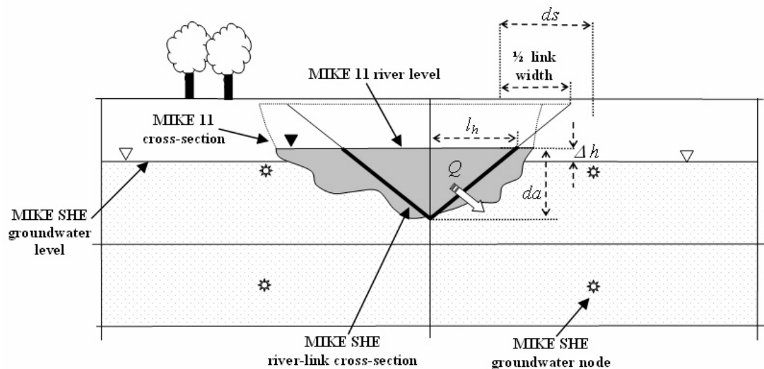
Figure 5-5. Linkage between MIKE SHE links and MIKE 11 cross-sections (from Anonymous 2009c).
