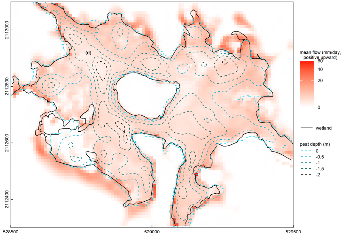
Figure 7-2. Simulated mean upward groundwater flow from lower to upper computational layers (01/01/2011-31/12/2013).
