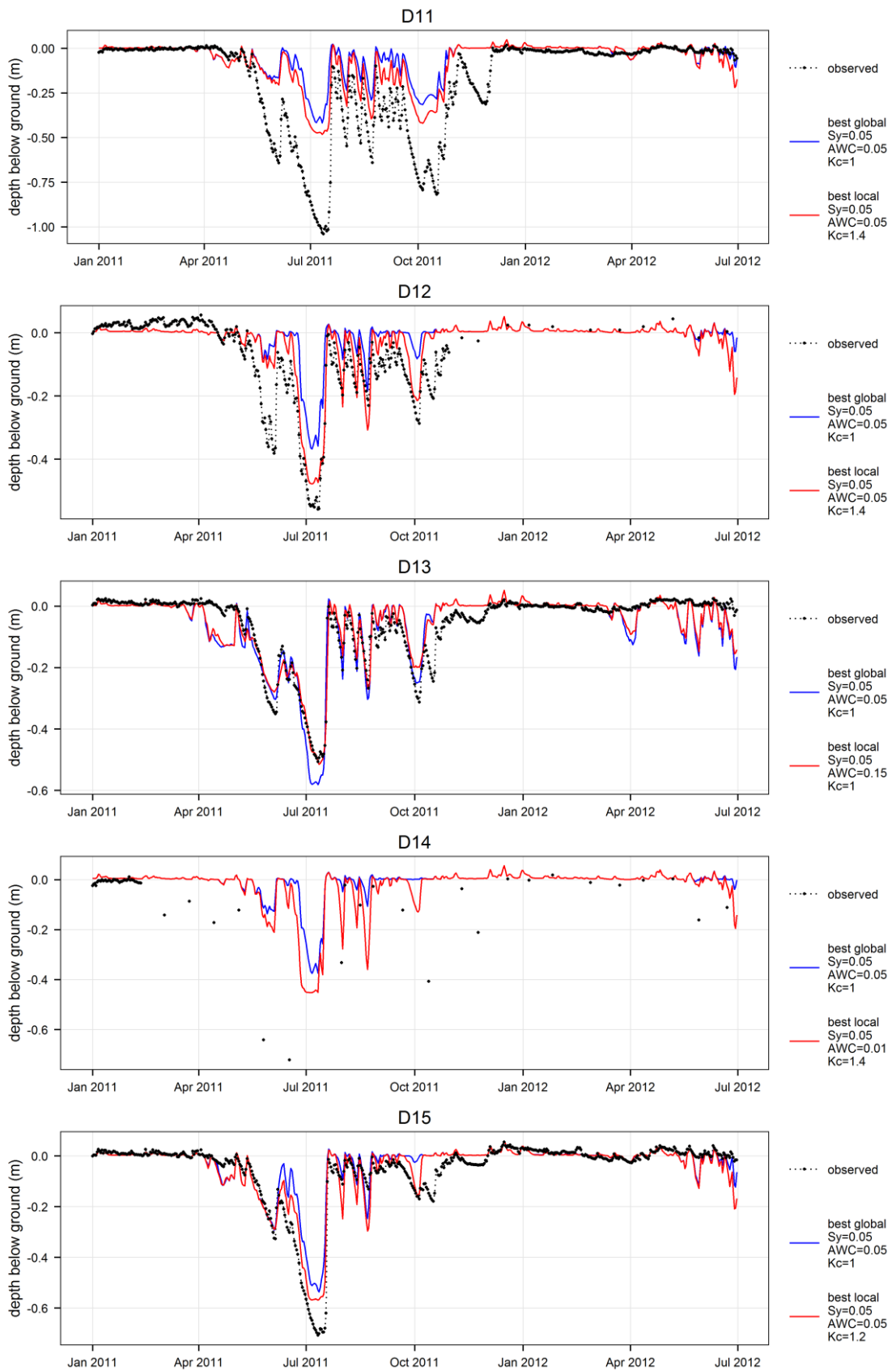
Figure 6-15 (continued). Effect of local peat specific yield, peat available water capacity and wetland crop coefficient on simulated groundwater table depth.
