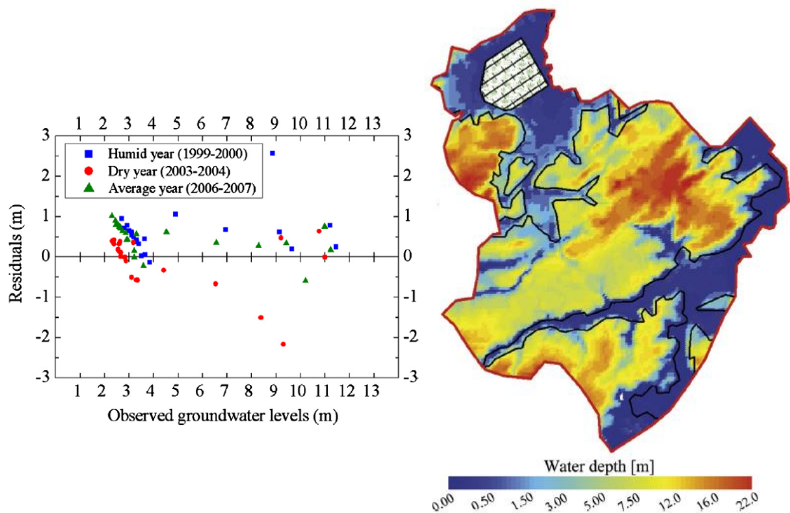
Figure 1-17. Performance of the model developed by Armandine Les Landes et al. (2014) with regard to groundwater table levels (left) and wetland spatial distribution (right).
