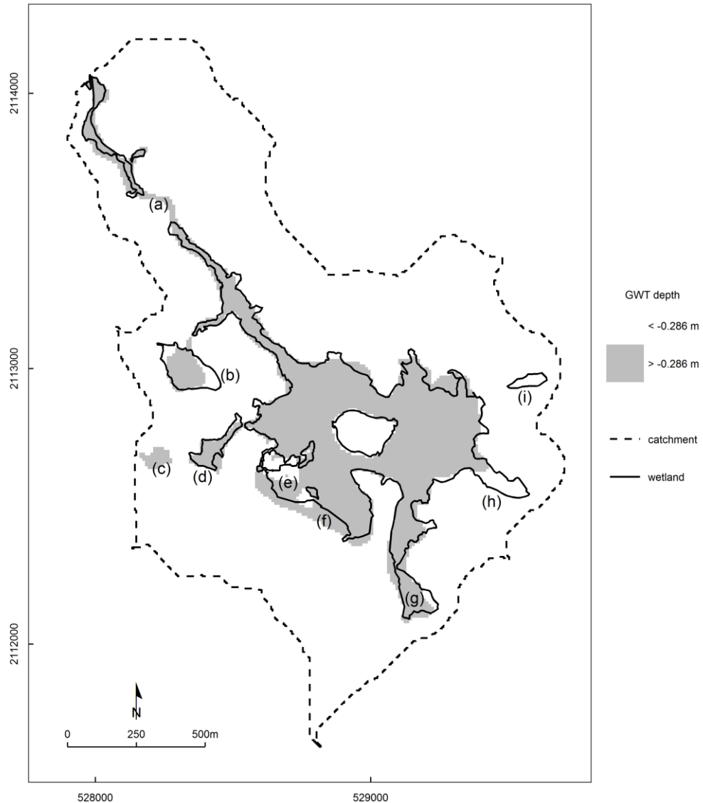
Figure 6-6. Spatial distribution of shallow groundwater tables (2011-2013 mean higher than -0.286\text{m} below ground level) and of wetland vegetation.
