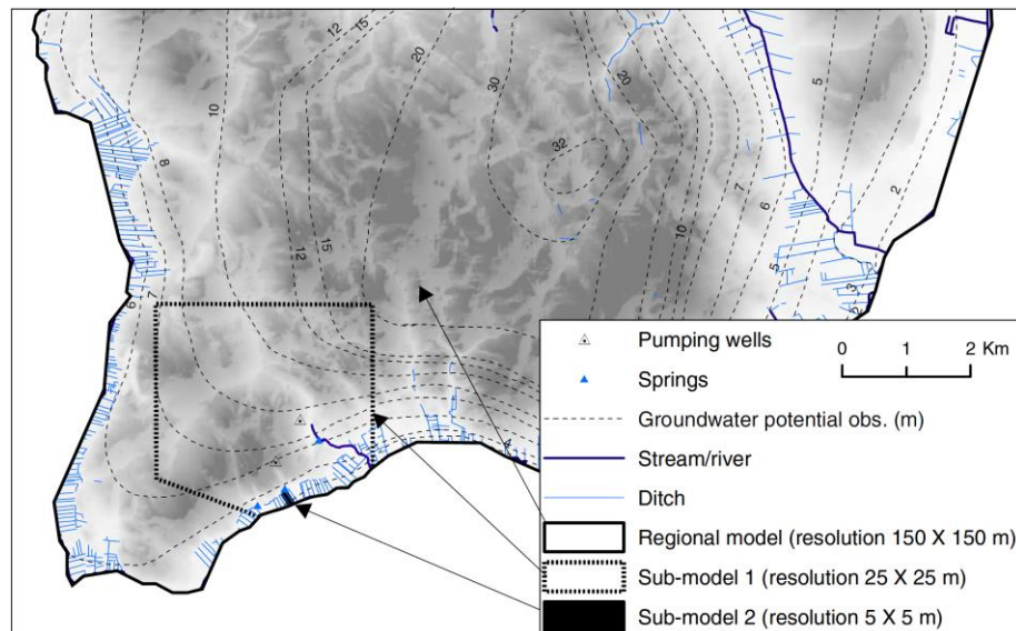
Figure 5-11. Nested models used by Johansen et al. (2014) to model the Lindenberg fen.
