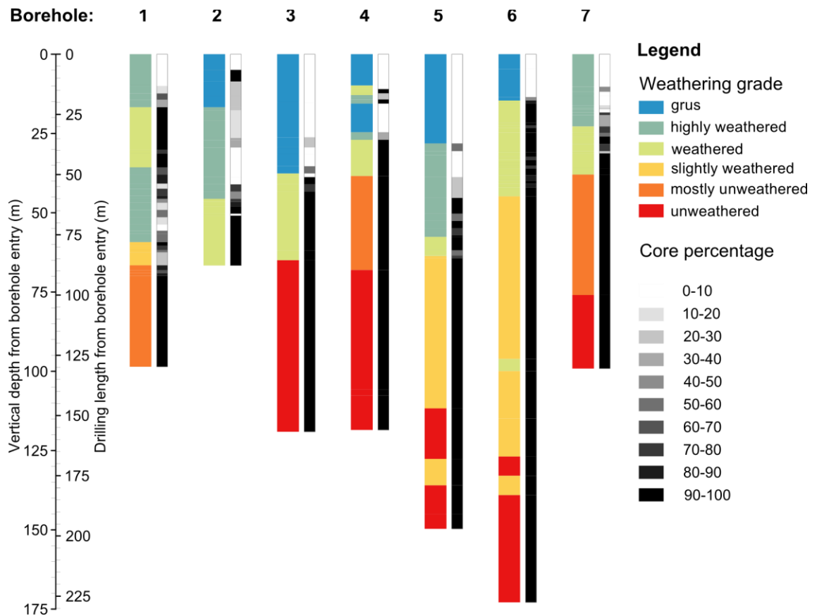
Figure 3-14. Weathering grades and core recovery percentage in the CEA boreholes
