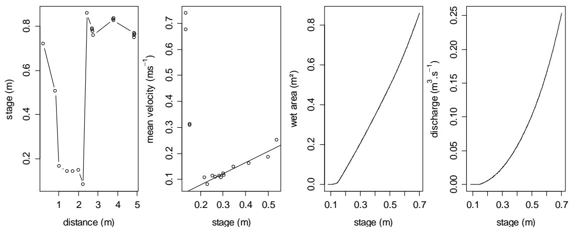
Figure 4-11. Stage-area-mean velocity plots at the Pont-de-Pierre gauging station.
