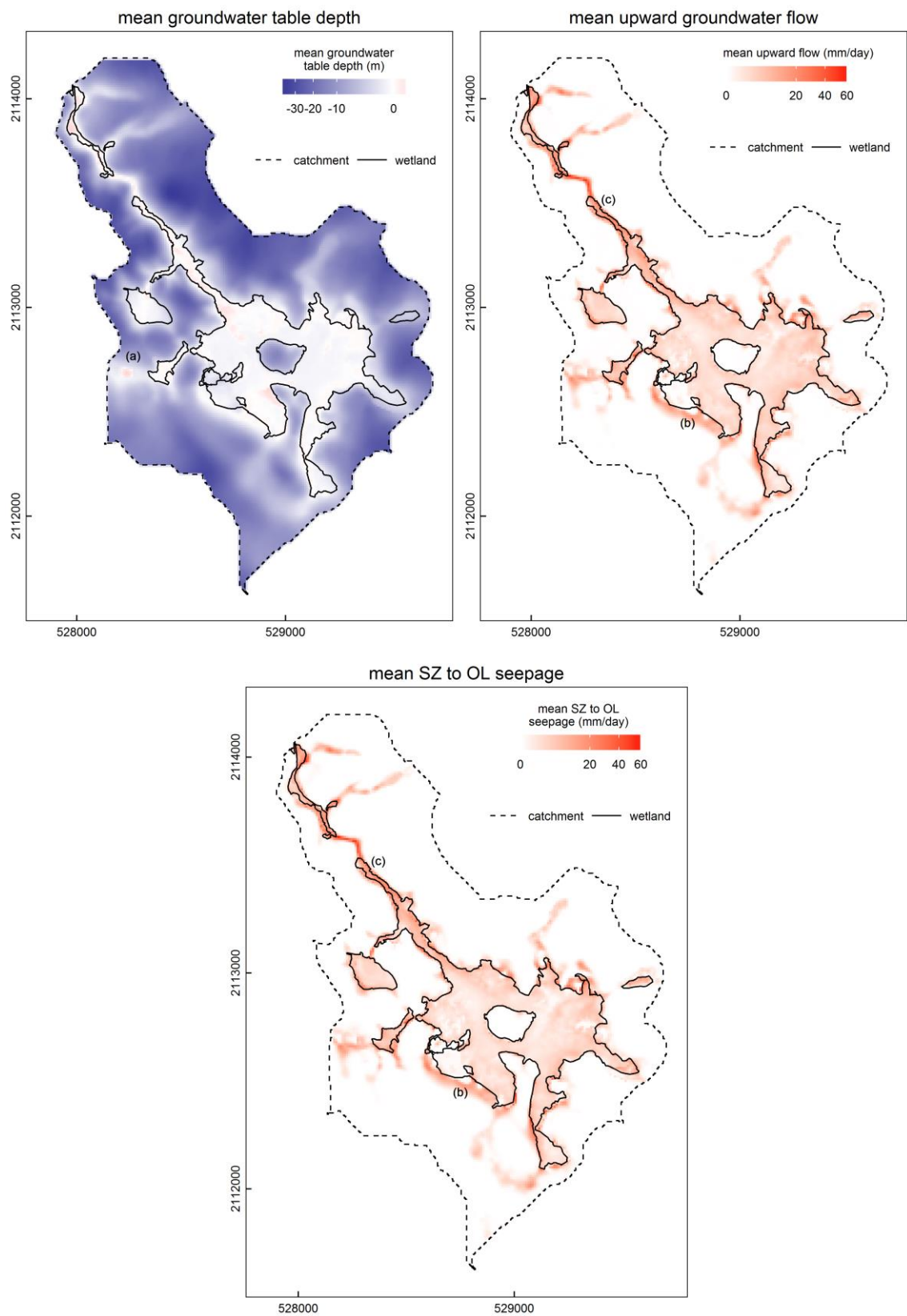
Figure 7-1. Simulated mean groundwater table depth, upward groundwater flow from lower to upper computational layers and seepage from saturated zone to overland flow (01/01/2011-31/12/2013).
