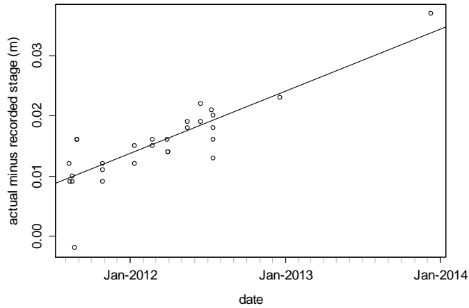
Figure 4-8. Logger drift at the Pont-de-Pierre gauging station.
