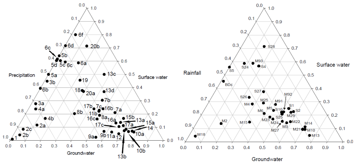
Figure 1-7. Average contribution of precipitation, surface water and groundwater to the maintenance of summer water levels in English and Welsh mires as a function of (left) identified wetland water supply mechanism and (right) plant community (from Wheeler et al. 2009).
