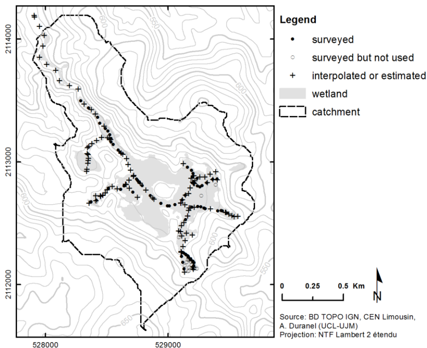
Figure 5-23. MIKE 11 cross-sections.
