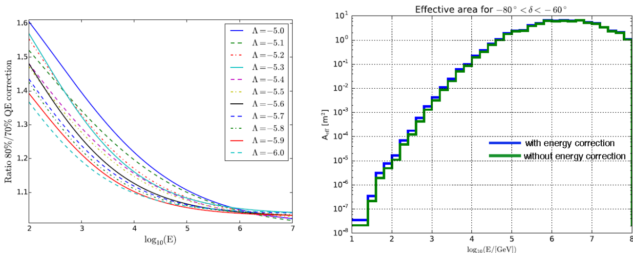
Figure 11.6.: ( Left ) Weight applied on each MC events simulated for the December 2015 period to compensate for the OM efficiency loss. The energy is given in GeV. Different \Lambda cuts have been tested and it seems that the weight is almost insensitive to it. ( Right ) Comparison of the ANTARES effective area (in the declination range -80^\circ < \delta < -60^\circ ) before and after the corrections have been applied. The effect of the corrections is mainly observed at low energies.
