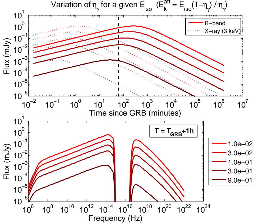
Figure 6.1.: ( Top: ) Evolution of the x-ray (dotted line) and optical (solid line) GRB afterglow light curves (forward shock) as function of \eta_\gamma . The black dashed line corresponds to one hour after the prompt emission ( Bottom: ) Broadband synchrotron spectra emitted by the shock-accelerated electrons 1 hour after the prompt emission for different values of \eta_\gamma .
