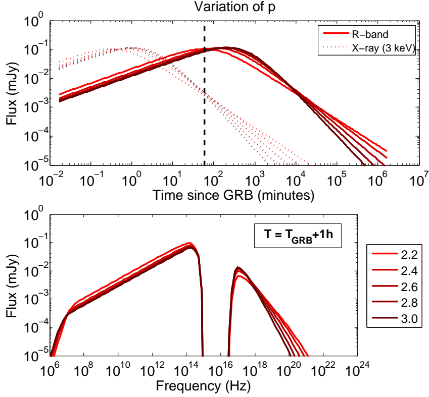
Figure 6.5.: ( Top: ) Evolution of the x-ray (dotted line) and optical (solid line) GRB afterglow light curves (forward shock) as function of p . The dashed-dotted line corresponds to one hour after the prompt emission ( Bottom: ) Broadband synchrotron spectra emitted by the shock-accelerated electrons 1 hour after the prompt emission for different values of p .
