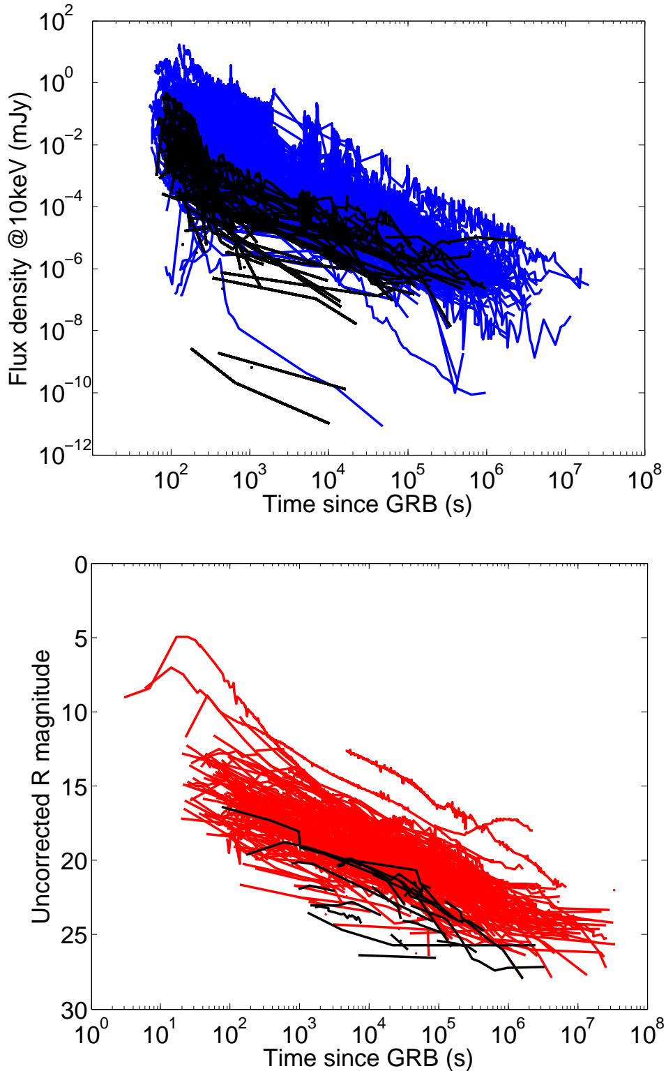
Figure 5.8.: Top: Swift-XRT afterglow light curves of 284 long GRBs (blue) and 69 short GRBs (black). Bottom: R-band afterglow light curves of 322 long GRBs (red) and 23 short GRBs (black). The R magnitudes are not corrected by the galactic extinction. For clarity we do not represent the upper limits on the afterglow brightness both in x-rays and in R-band.
