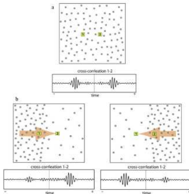
Fig. B.1 Schematic illustration of the effect of inhomogeneous noise sources distribution on the degree of symmetry of cross correlation function. (a) Symmetric cross correlation between 1 and 2 obtained when the sources of noise are evenly distributed. (b) Asymmetric cross correlation (but symmetric travel
