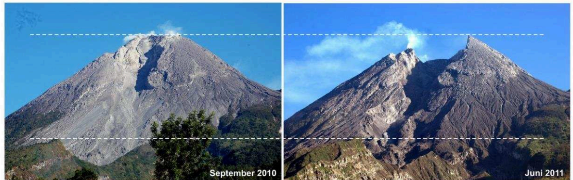
Fig. 1.1 Morphology of Merapi edifice seen from South flank before and after the 2010 eruption (Suroño et al., 2012).
