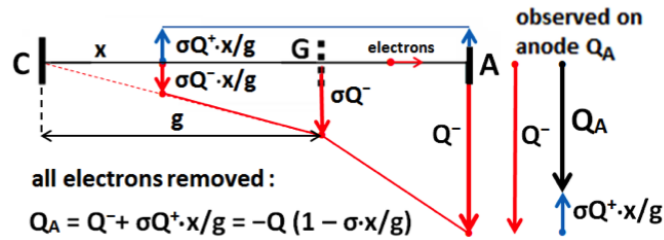
Figure 2.5: Gridded ionisation chamber with grid inefficiency being taken into account. From [52].
