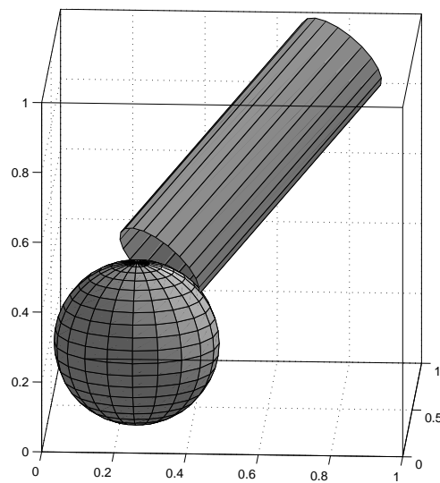
Figure E.5 – Intersection sphère-cylindre de type sc4 .
