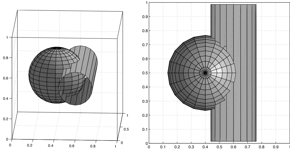
Figure E.2 – Intersection symétrique sphere-cylindre de type sc2 .
