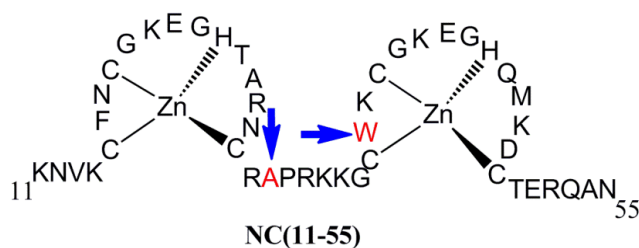
Figure 2.1.3. Structure of NC(11-55) peptide.
