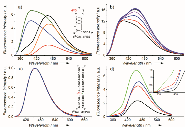
Figure 4. Emission spectra of d^{\text{th}}\text{G7}(-)\text{PBS} (a, b) and d^{\text{th}}\text{G7}(-)/(+)\text{PBS} duplexes (c, d). (a) Emission spectra of d^{\text{th}}\text{G7}(-)\text{PBS} recorded at different excitation wavelengths: 298 nm (blue), 320 nm (green), 345 nm (black), 360 nm (orange), and 380 nm (red). Inset: structure of d^{\text{th}}\text{G7}(-)\text{PBS} , the G7 residue (red) is replaced by d^{\text{th}}\text{G} . (b) Emission spectra of d^{\text{th}}\text{G7}(-)\text{PBS} in the absence (black) and in the presence of 1 to 6 equivalents of NC(11-55) protein (red to violet) at 320 nm excitation wavelength. (c) Emission spectra of the matched d^{\text{th}}\text{G7}(-)/(+)\text{PBS} duplex at the same excitation wavelengths as in (a). Inset: structure of d^{\text{th}}\text{G7}(-)/(+)\text{PBS} duplex. In mismatched duplexes, the C residue in green is replaced by a A, G or T. (d) Emission of the matched and mismatched d^{\text{th}}\text{G7} -labeled (-)/(+)\text{PBS} duplexes at 310 nm excitation wavelength. The base opposite to d^{\text{th}}\text{G} is C (black, native duplex), T (blue), G (red), or A (green). Inset: zoom of the blue part of the spectra. The buffer was as in Figure 2.
