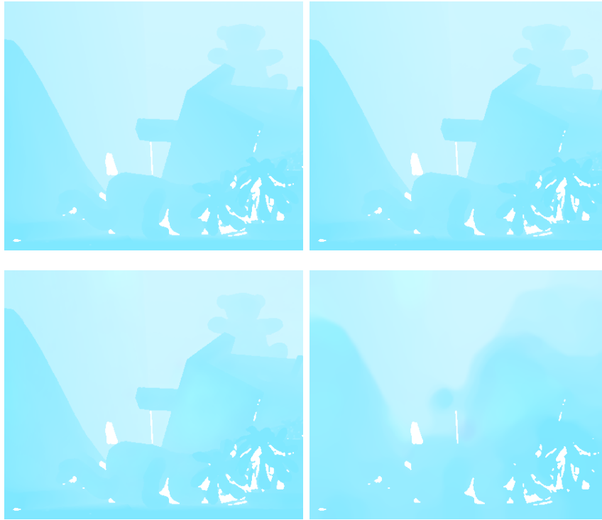
Fig. 6.4: Optical flow estimates for the Teddy stereo dataset. From left to right, from top to bottom: (a) Ground-truth, and (b) twist-motion, (c) 3D-motion and (d) 2D-motion representations.
