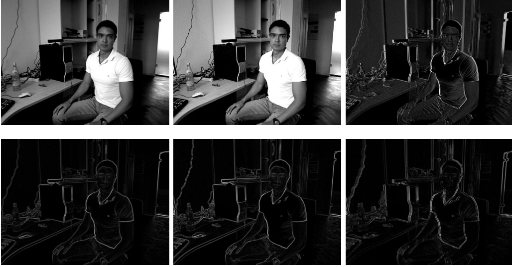
Fig. 5.3: Brightness constancy violation. From left to right, top to bottom: (a) first image, (b) second image, (c) image difference, (d) first and (e) second images of the magnitude of the gradient, and (f) their difference. While the camera is moving, there exists an automatic white balance that modifies the gray value image, as can be noted in the image difference (c), changes that are not related to the motion. On the other hand, the magnitude of the gradient is too little affected since it measures the image structure, or texture, regardless uniform changes in luminance.
