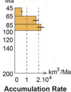
Figure 7-2 Late Cretaceous – Early Eocene (100 – 45 Ma) denudation and accumulation. (A) Cenomanian-Santonian denudation map (100 – 85 Ma, Figure 6-21) and Upper Cenomanian paleogeographic map (97 – 93 Ma, Figure 3-9) overlapping on the topographic map of West Africa. Arrows indicate potential draining directions of eroded materials. Denudation rate in West Africa (B) and accumulation rates in the Equatorial Atlantic basins (C) are shown.
